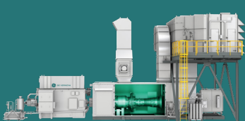
TM2500 Power plant on wheels
