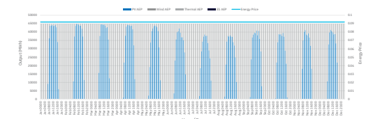
Typical Hybrid annual energy production operation
