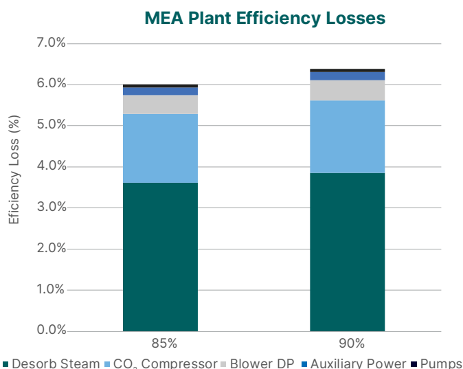
Figure 9: Plant efficiency losses for a combined cycle plant at 90 percent and 85 percent carbon capture.
