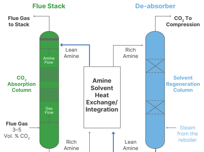
Figure 8: Post combustion amine process diagram
