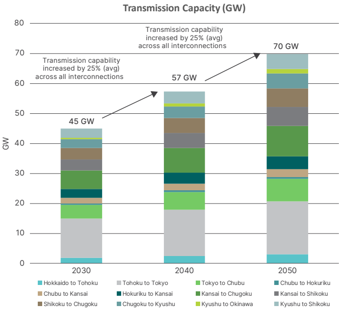
Figure 9: Interconnection capacity (GW)
