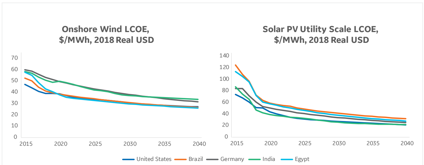
FIGURE 4: LCOE of Onshore Wind and Utility Scale Solar PV are expected to continue to drop.
