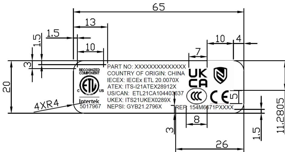
Figure 3: Example Reduced Size Nexus OnCore Module IECEx Nameplate
