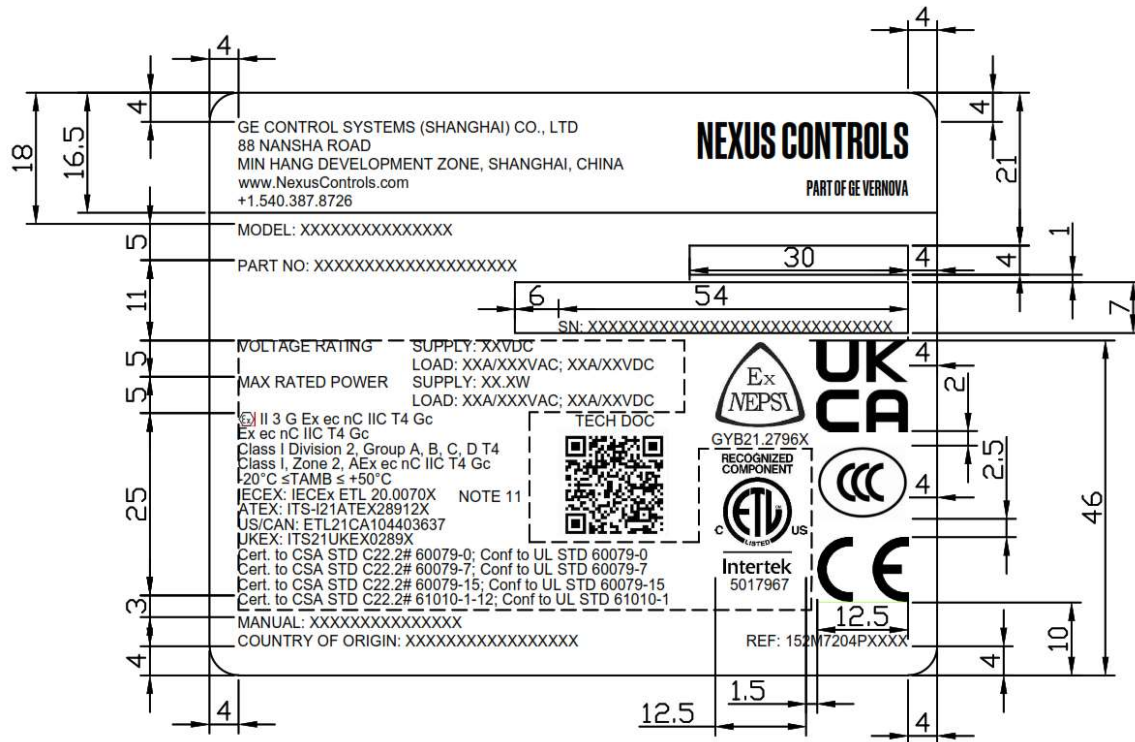
Figure 1: Example Nexus OnCore Module IECEx Nameplate for China
