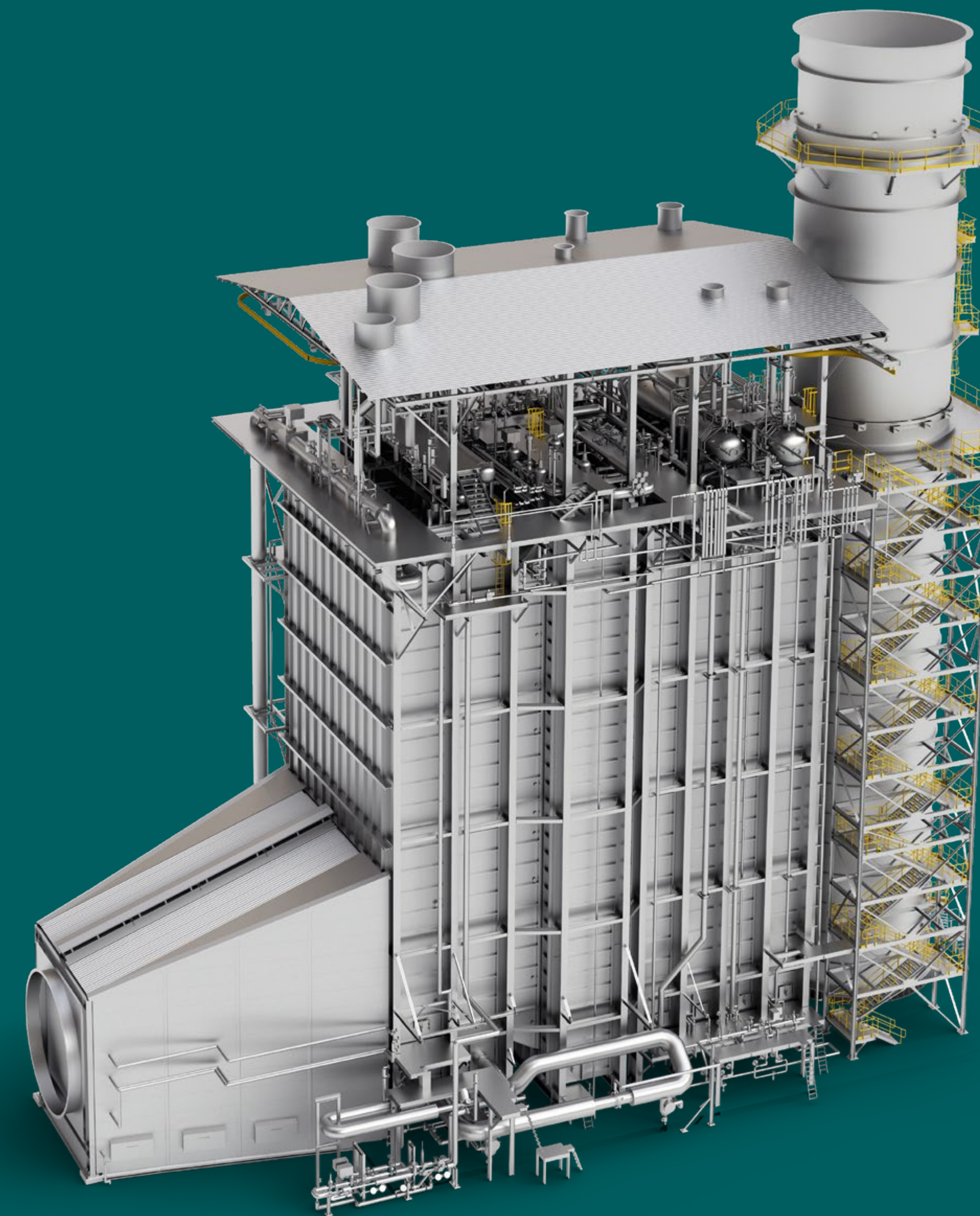
Horizontal Once Through (OT)
