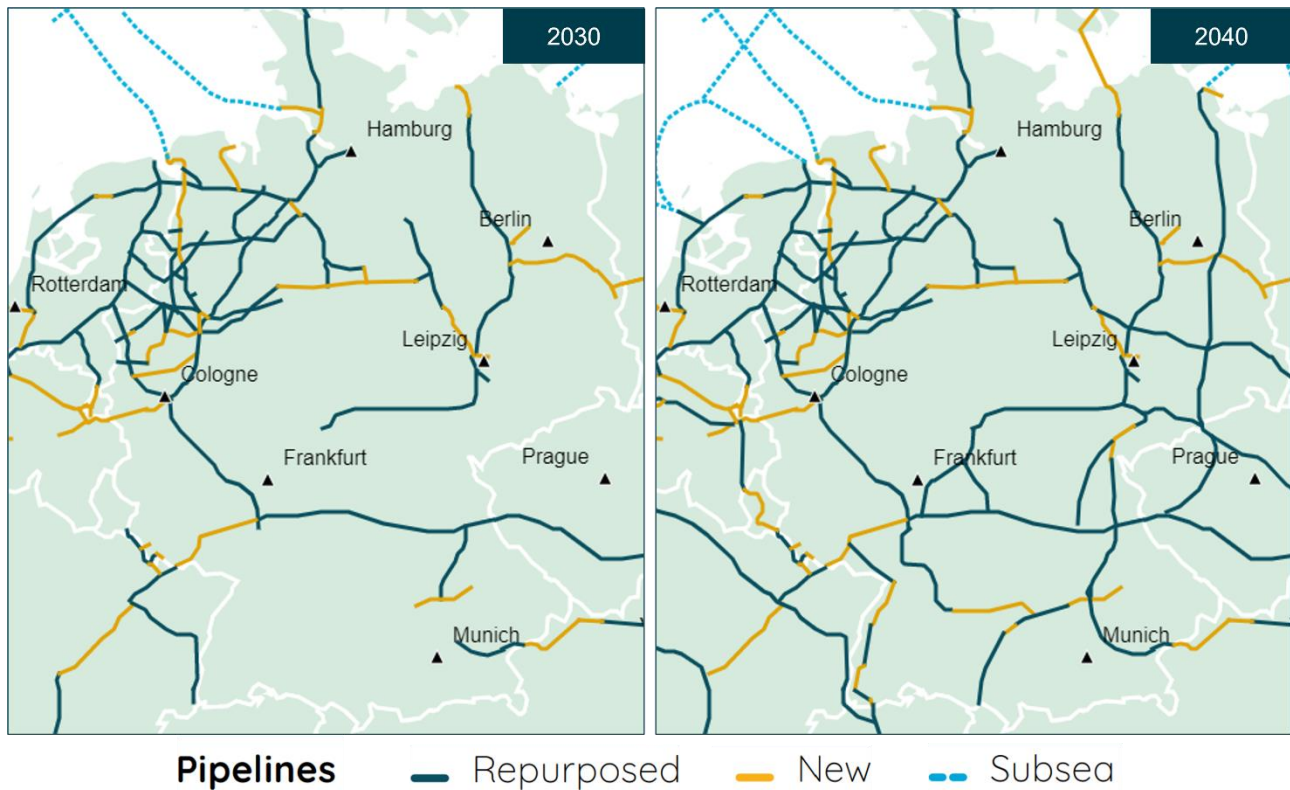
Figure 10 The European Hydrogen Backbone in Germany by 2030 and 2040
