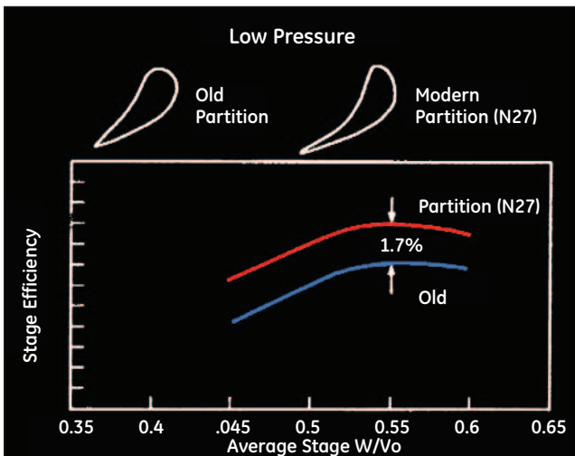
Figure 5. Improved nozzle design
