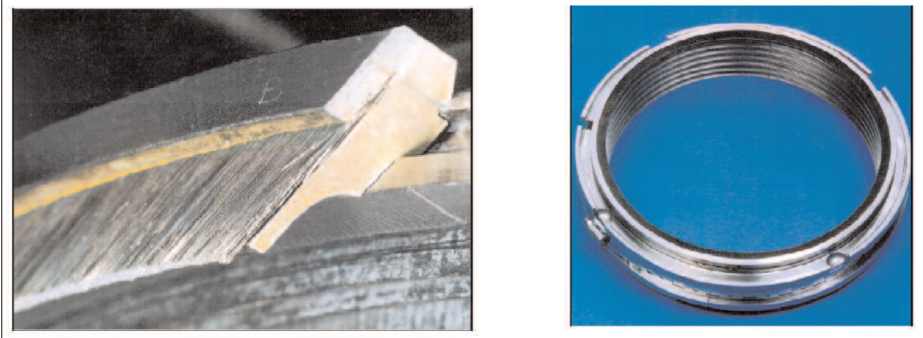
Figure 12. GE brush seal designs
