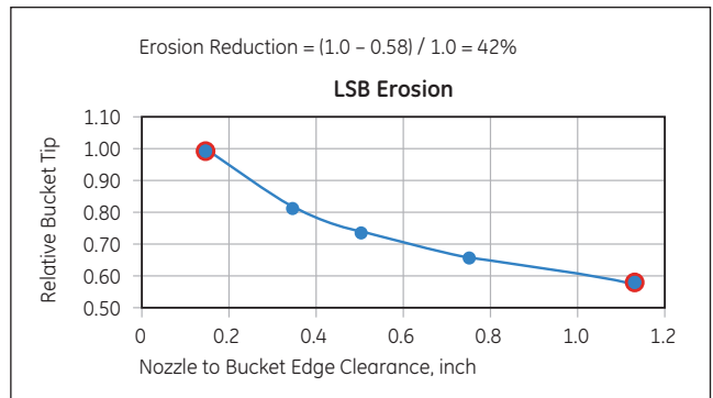
Figure 18. 20-inch LSB erosion reduction using new generation diaphragm
