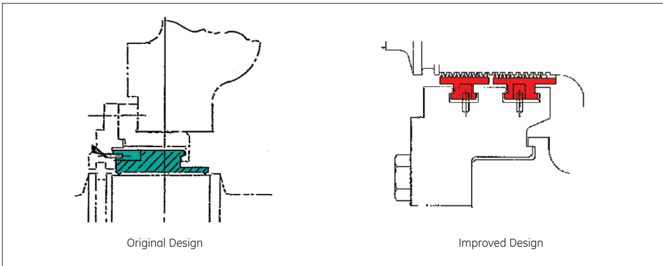
Figure 11. Comparison of original and improved nozzle box packing designs
