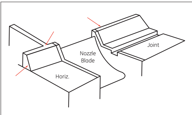
Figure 16. Enhanced design has Z-joint
