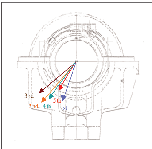
Figure 10. Sketch of bearing with partial arc valve forces for each valve point. Vector magnitudes are to scale relative to each other.
