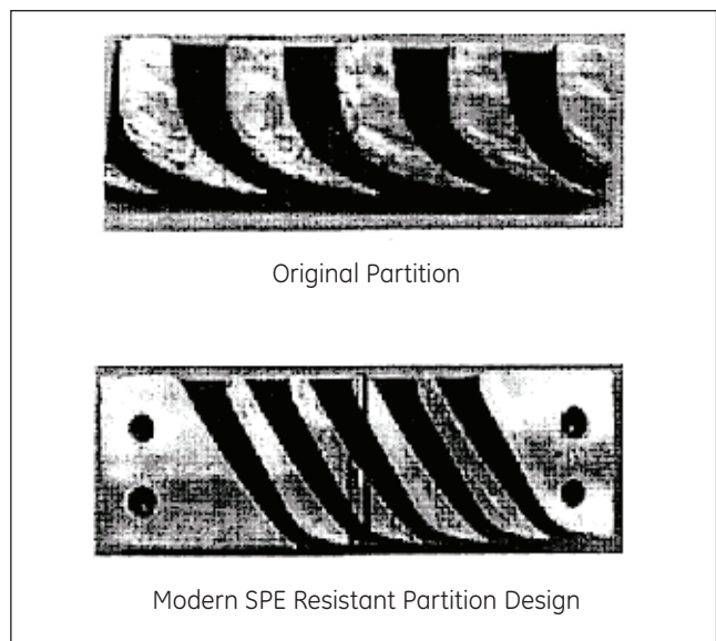
Figure 13. Comparison of nozzle profiles to minimize solid particle erosion
