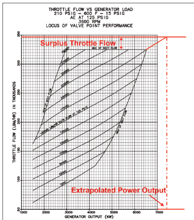
Figure 9. Extraction map extrapolation
