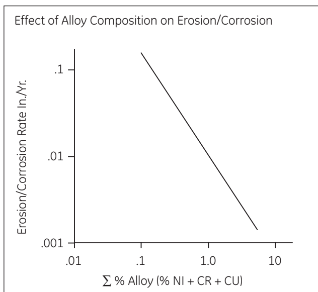
Figure 14. Effect of alloy composition on erosion rates
