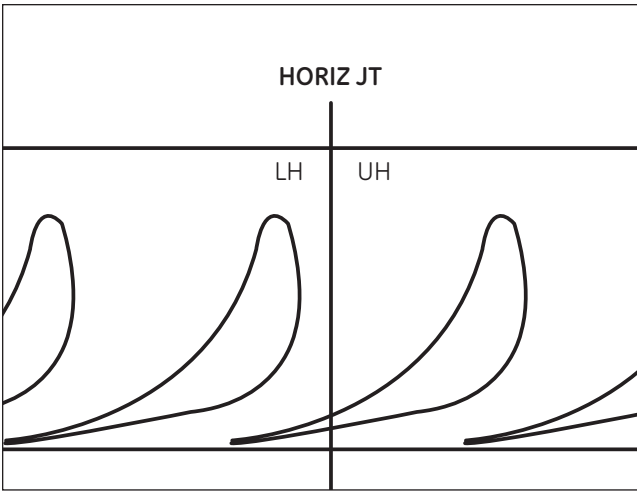
Figure 15. Existing design has split vane at joint
