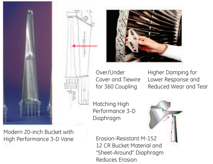
Figure 4. 3D 20-inch last stage bucket and diaphragm
