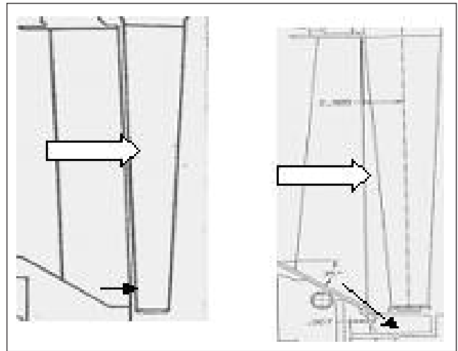
Figure 17. Old vs. new generation shoot-around diaphragm design
