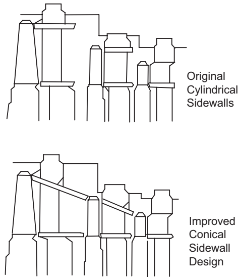
Figure 6. Conical sidewall diaphragm construction
