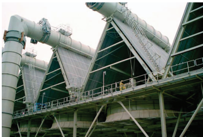
Figure 4. Air-cooled condenser showing horizontal cooling fans and heat exchanger tubes
