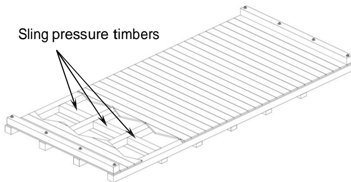
Figure 13: Sling pressure timbers as a part of the bottom design
