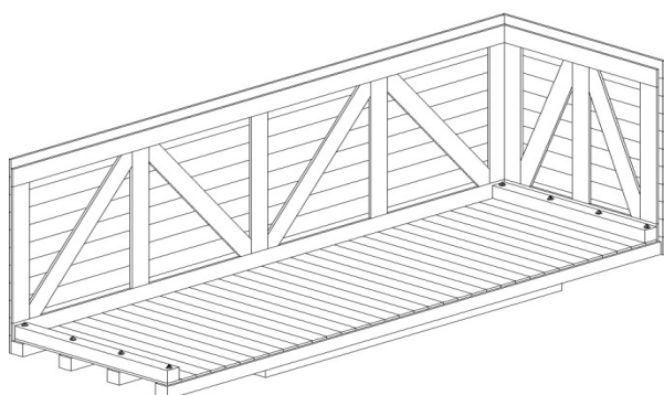
Figure 24: Box with horizontal saw wood boarding.
