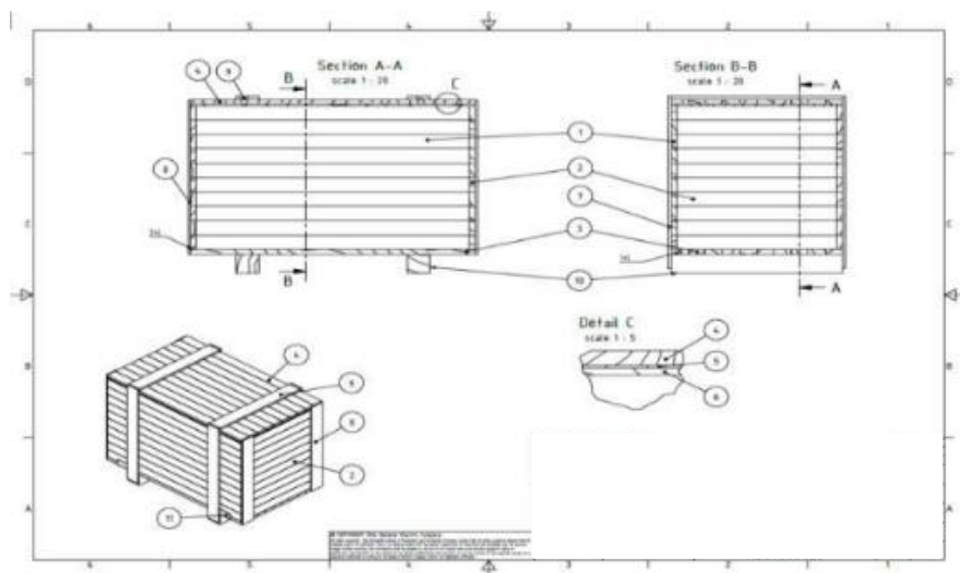
Figure 1: Solid wooden box type 1
