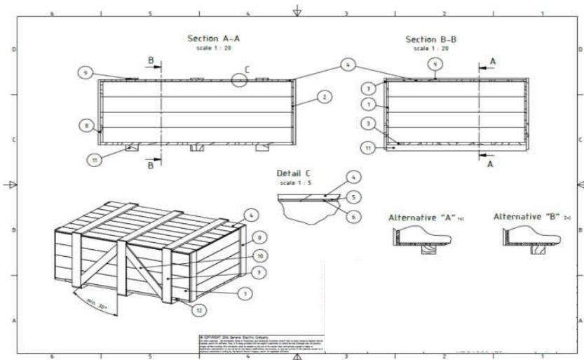
Figure 4: Solid wooden box type 6
