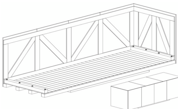
Fig 25: Box cladding made of plywood panels
