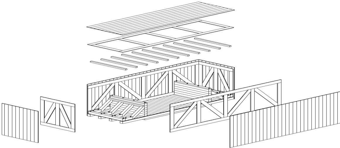
Figure 20: Composition of box walls
