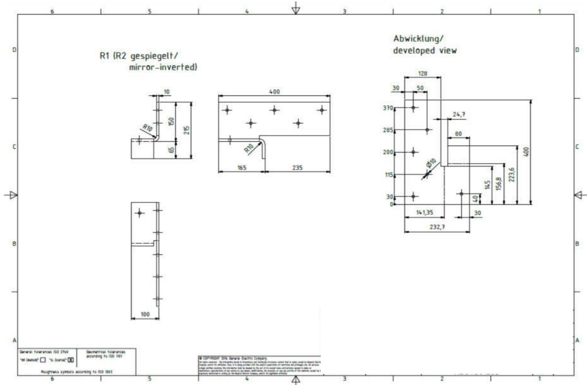
Figure 28: Sling protection 20 to 50 tonnes
