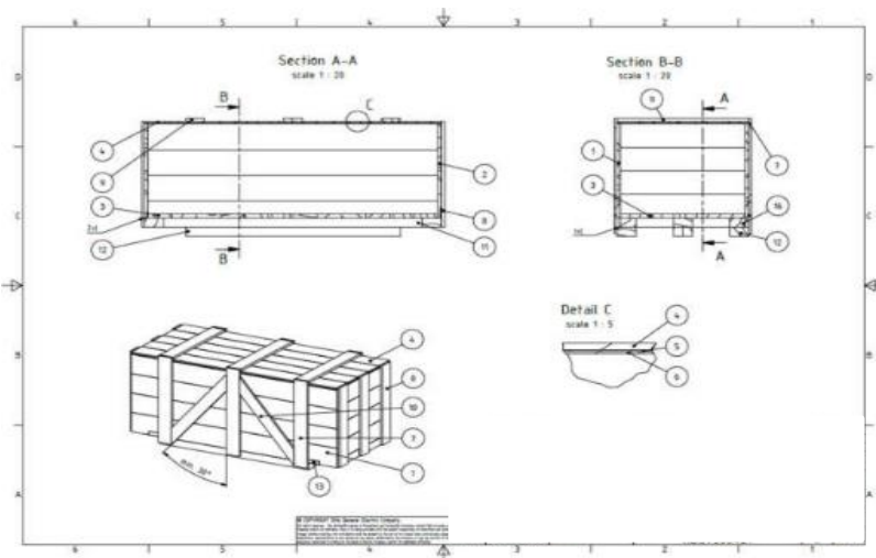
Figure 2: Solid wooden box type 4
