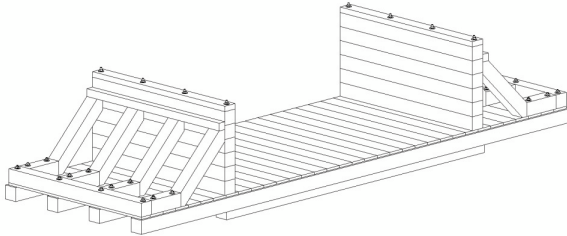
Figure 17: Bottom design with supports and supporting beams
