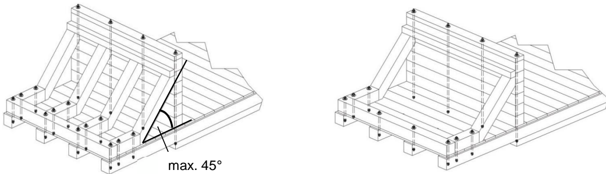
Figure 17: Bottom design with supports and supporting beams
