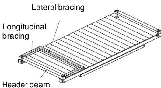
Figure 15: Structure of bracing without direct bolting.
