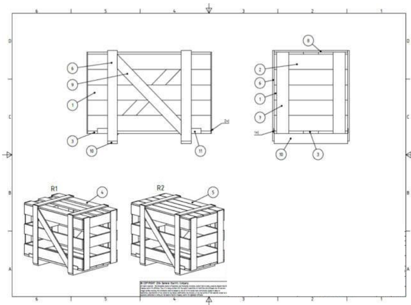
Figure 7: Solid wooden crate type 1 and 2
