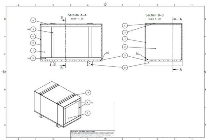
Figure 5: Plywood box type 7
