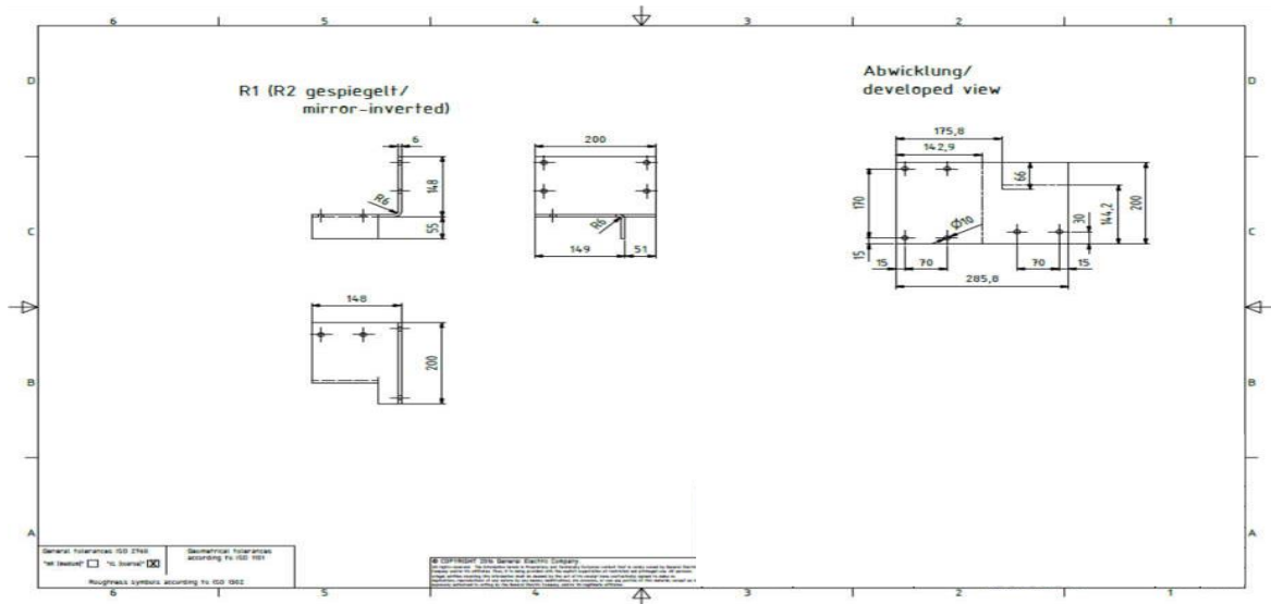
Figure 27: Sling protection 5 to 20 tonnes
