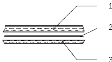
Figure 23: Composition of rain protection lid using PE foil
