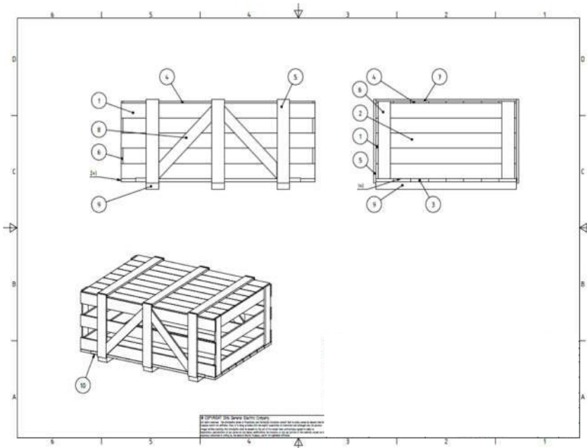
Figure 8: Solid wooden crate type 3
