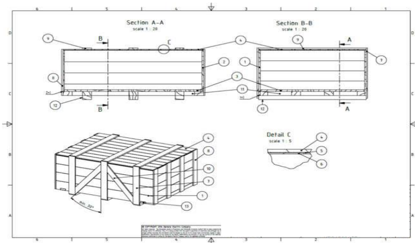
Figure 3: Solid wooden box type 5
