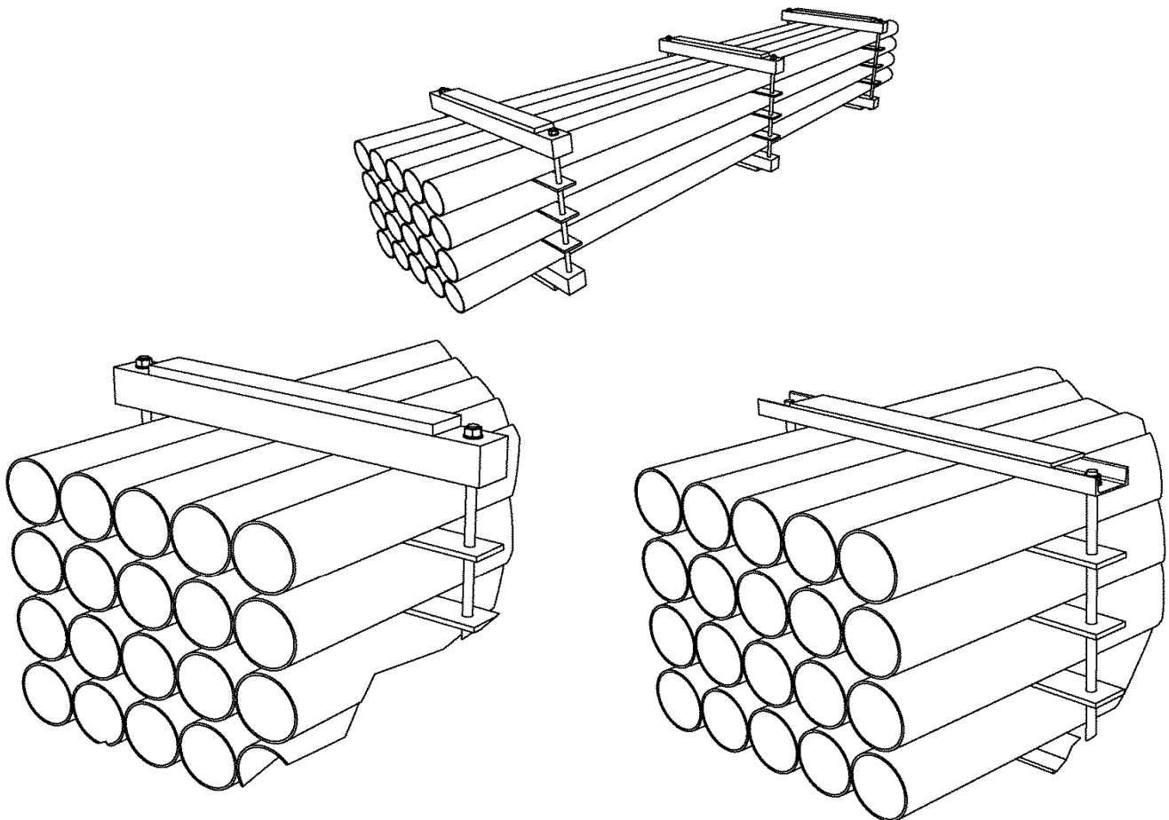
Figure 10: Bundles having clamps made of squared timbers or sectional steel
