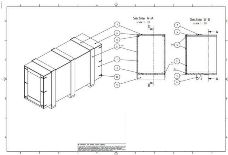
Figure 6: Plywood box type 8
