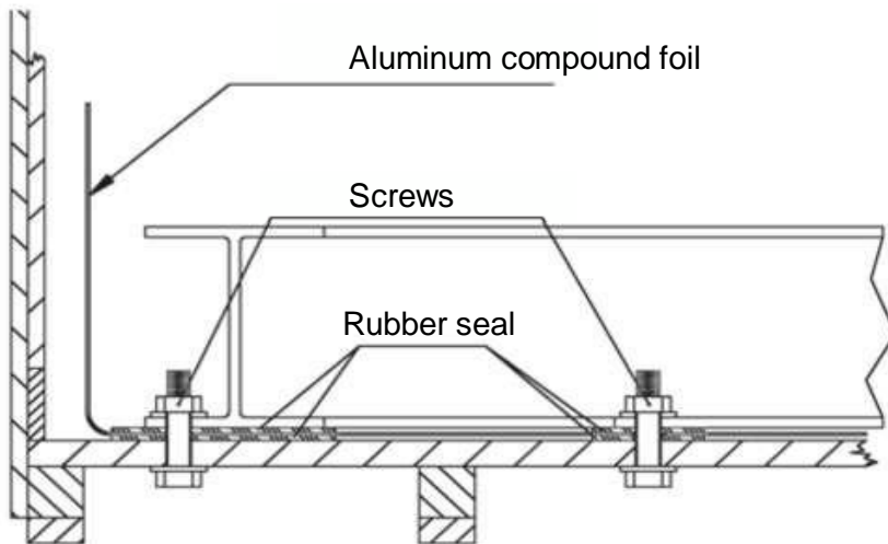
Figure 14: Foil sealing of bolted connections
