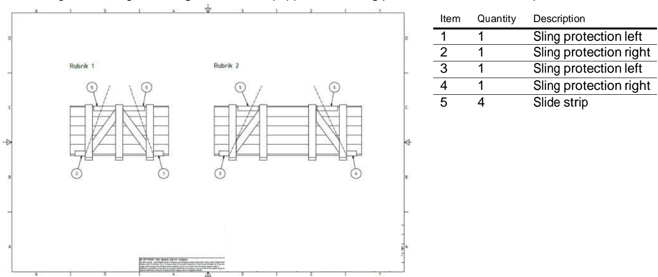
Figure 26: Fittings for box protection
