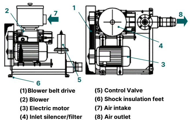
Fig. 1: drawing of the blower skid and list of its main components
