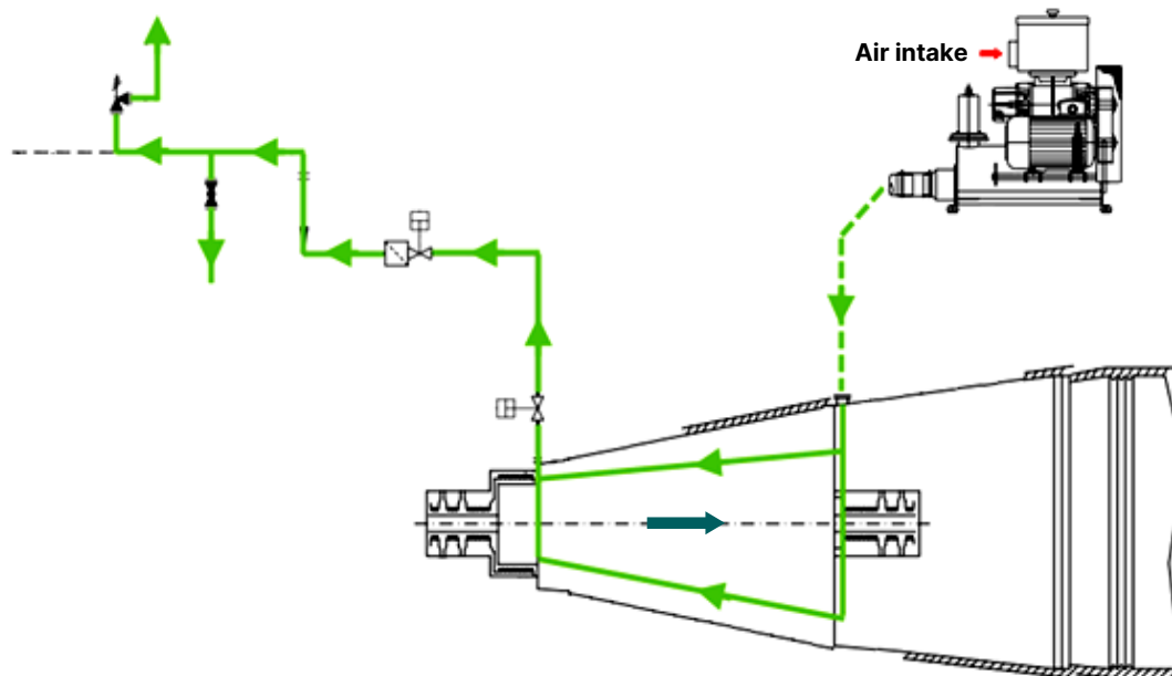
Fig. 2: Counter air flow path
