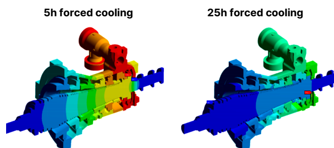
Fig. 3: 3D Thermal distribution during cool down
