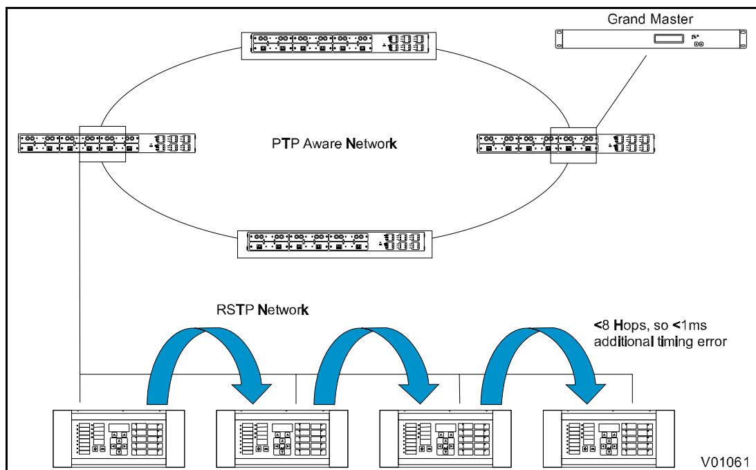
Figure 23: Timing error using ring or line topology
