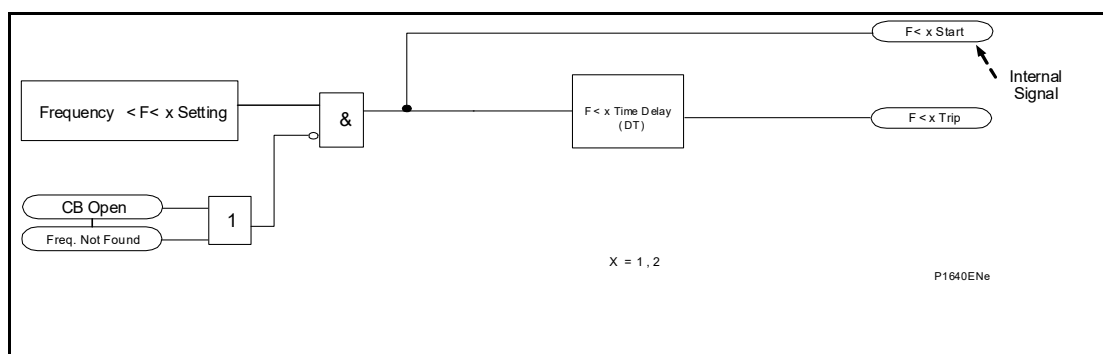
Figure 30: Underfrequency logic
