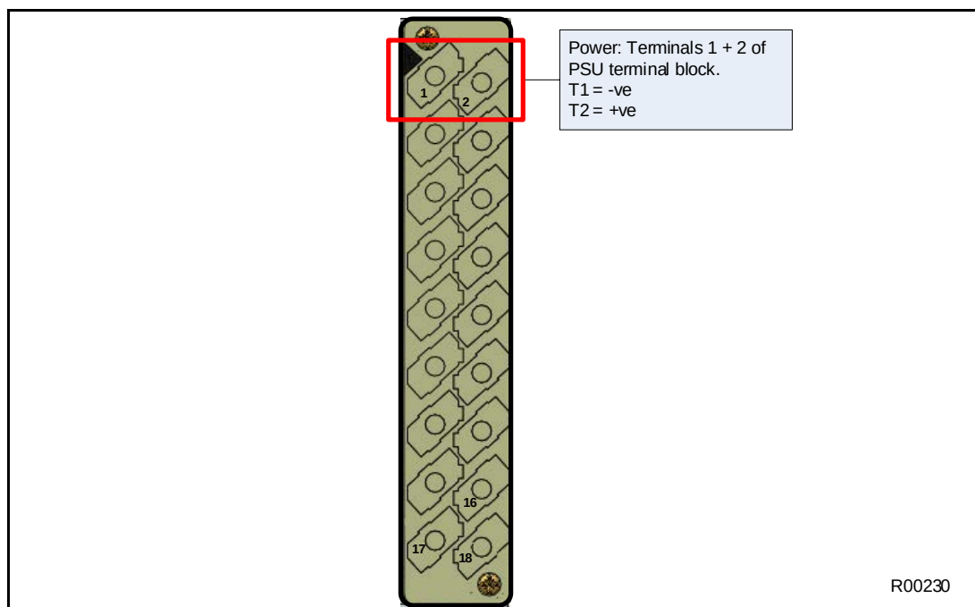
Figure 6: Power supply terminals
