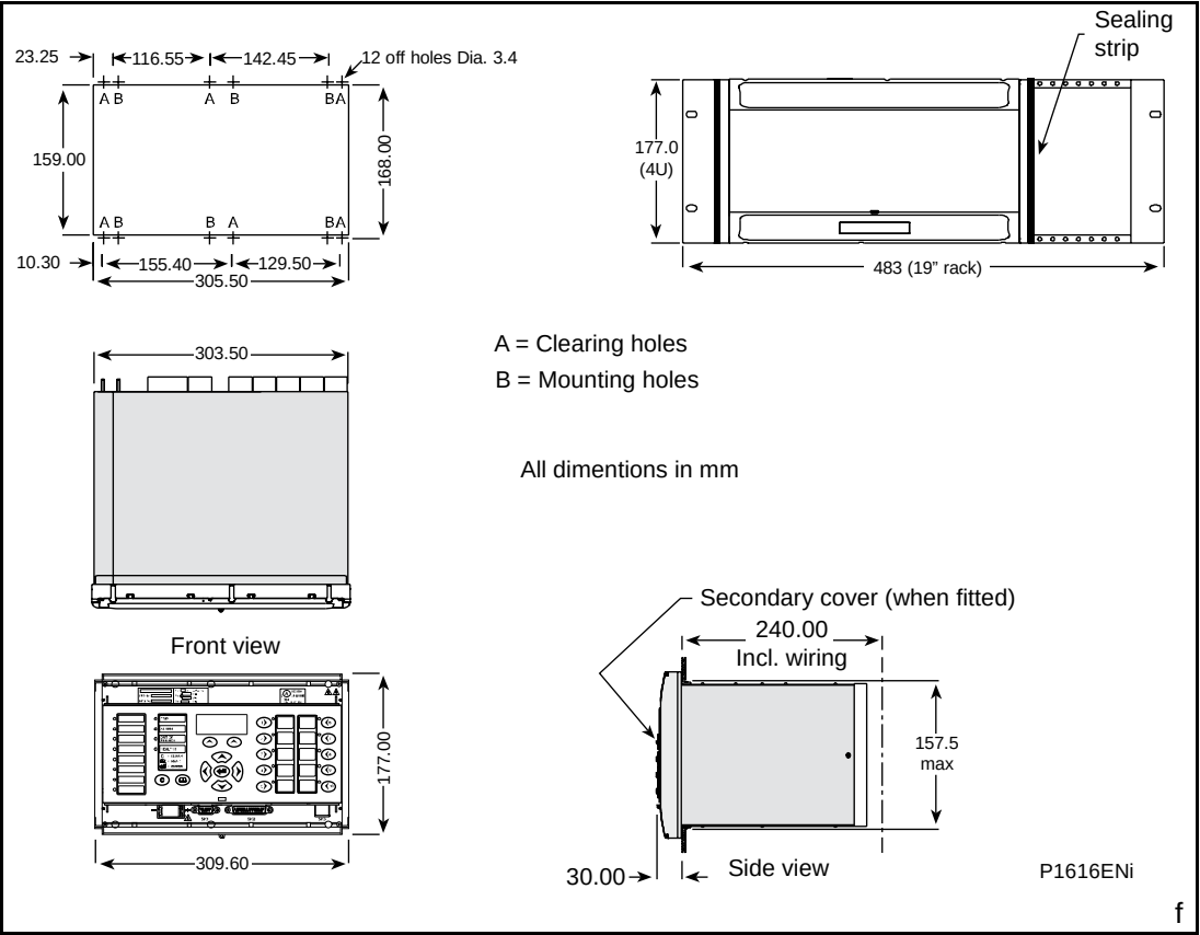
Figure 12: P242 case dimensions (60TE case)
