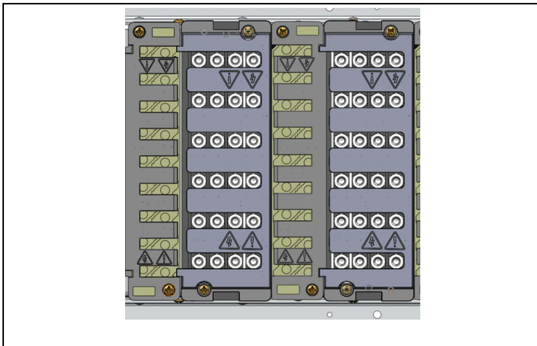
Figure 4: Example—fitted IP2x shields (cabling omitted for clarity)
