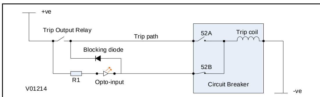
Figure 21: TCS scheme 1
