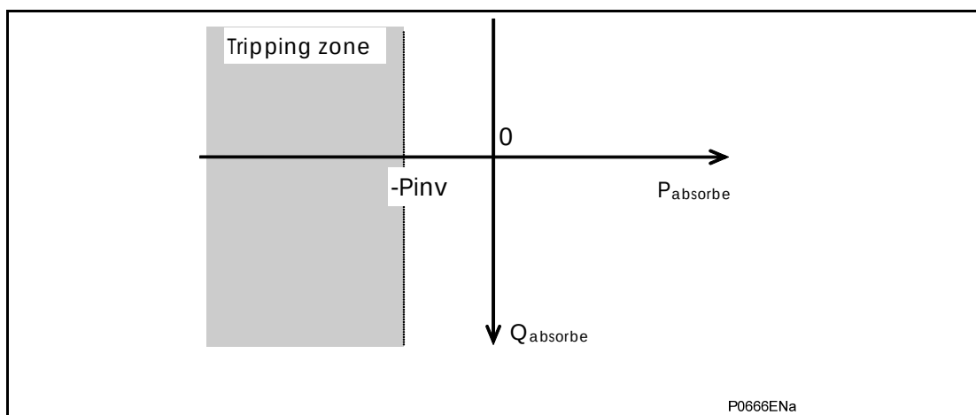
Figure 33: Reverse power protection
