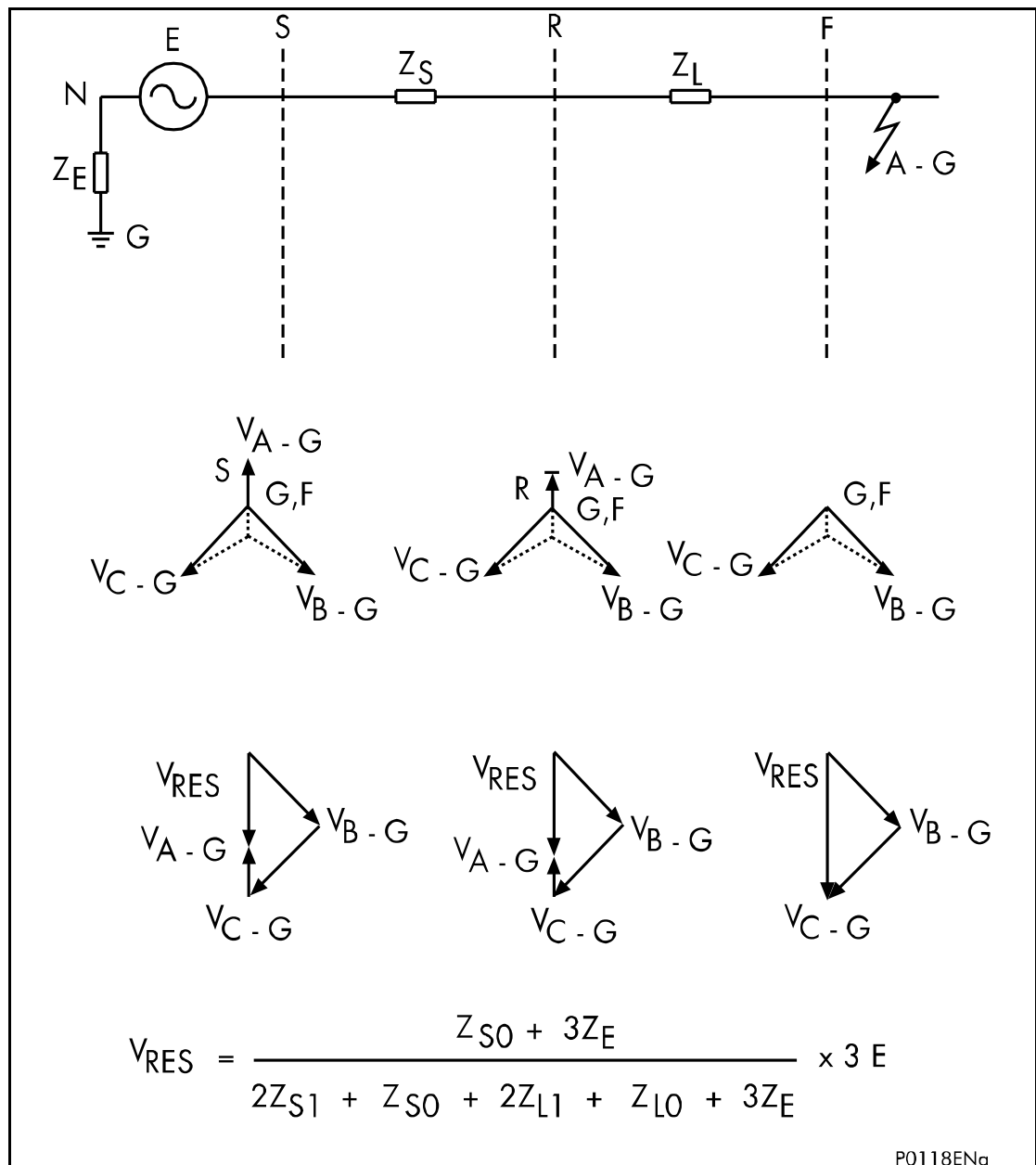
Figure 19: Residual voltage
