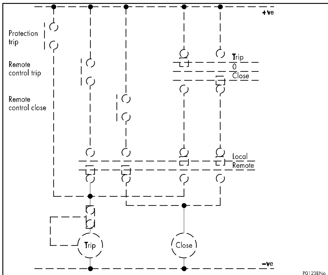
Figure 55: Remote control of circuit breaker
