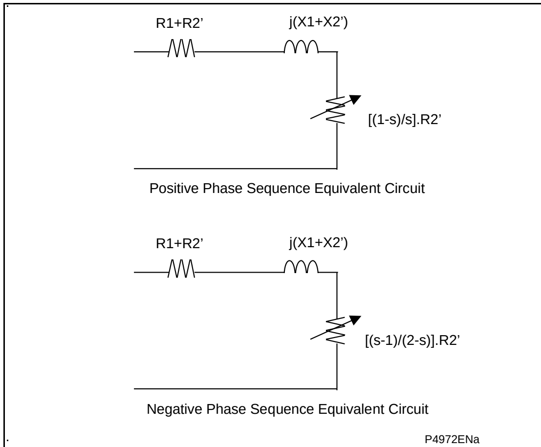
Figure 20: Equivalent circuits
