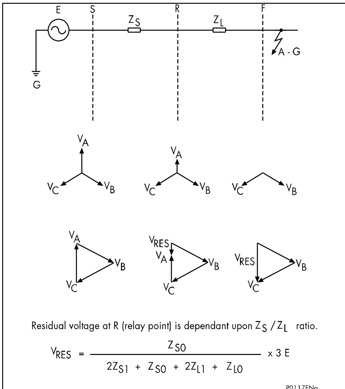
Figure 18: Residual voltage
