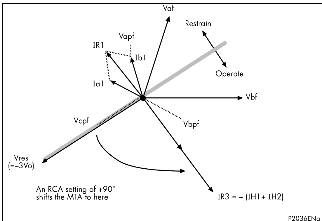
Figure 10: Phasor diagrams for insulated system with C phase fault
