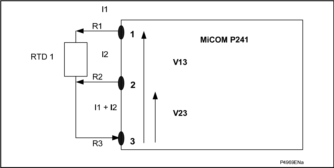
Figure 47: RTD connection
