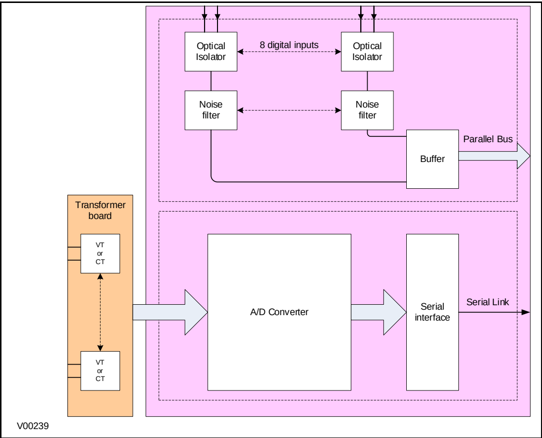
Figure 10: Input module schematic
