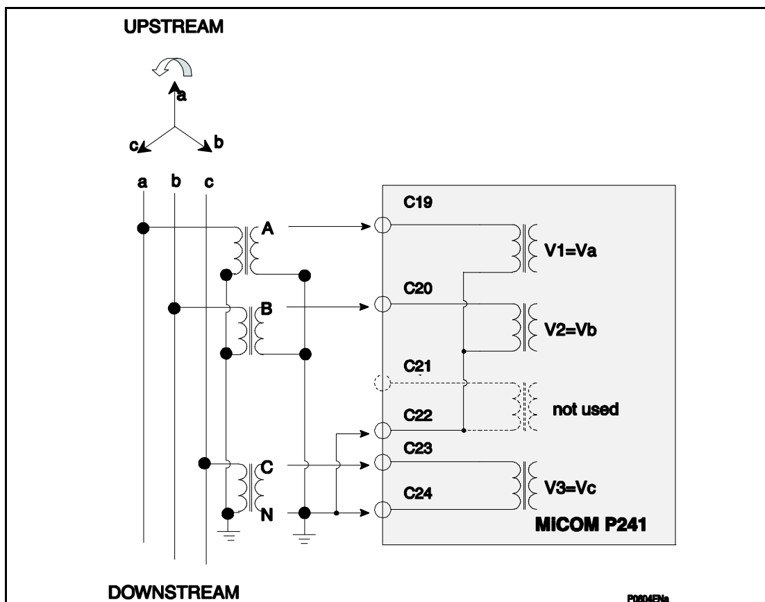
Figure 27: 3 VTS configuration
