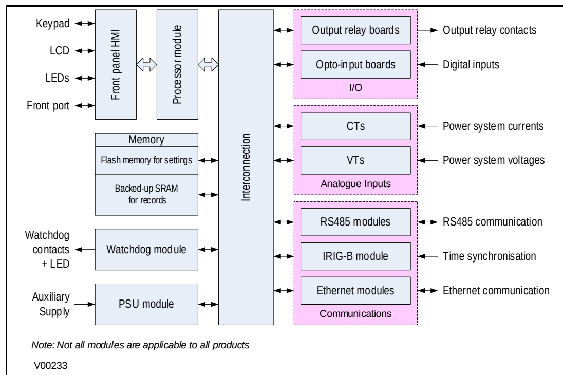
Figure 1: Hardware architecture
