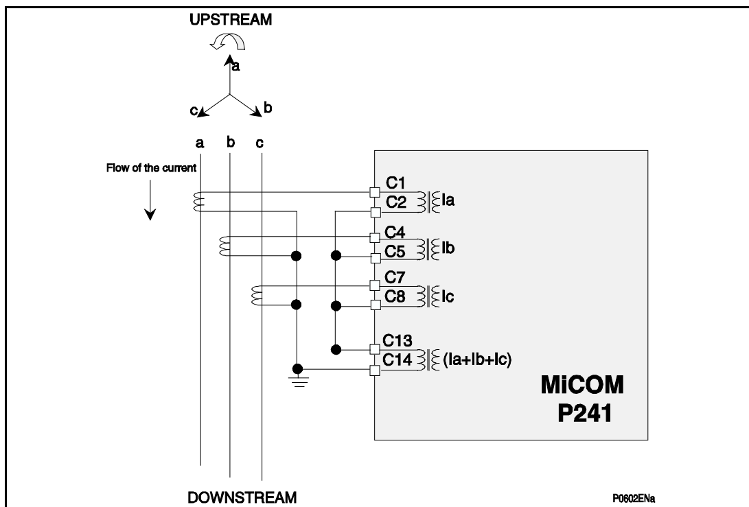
Figure 6: 3 CT configuration
