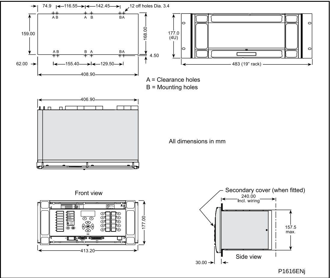
Figure 13: P243 case dimensions (80TE case)
