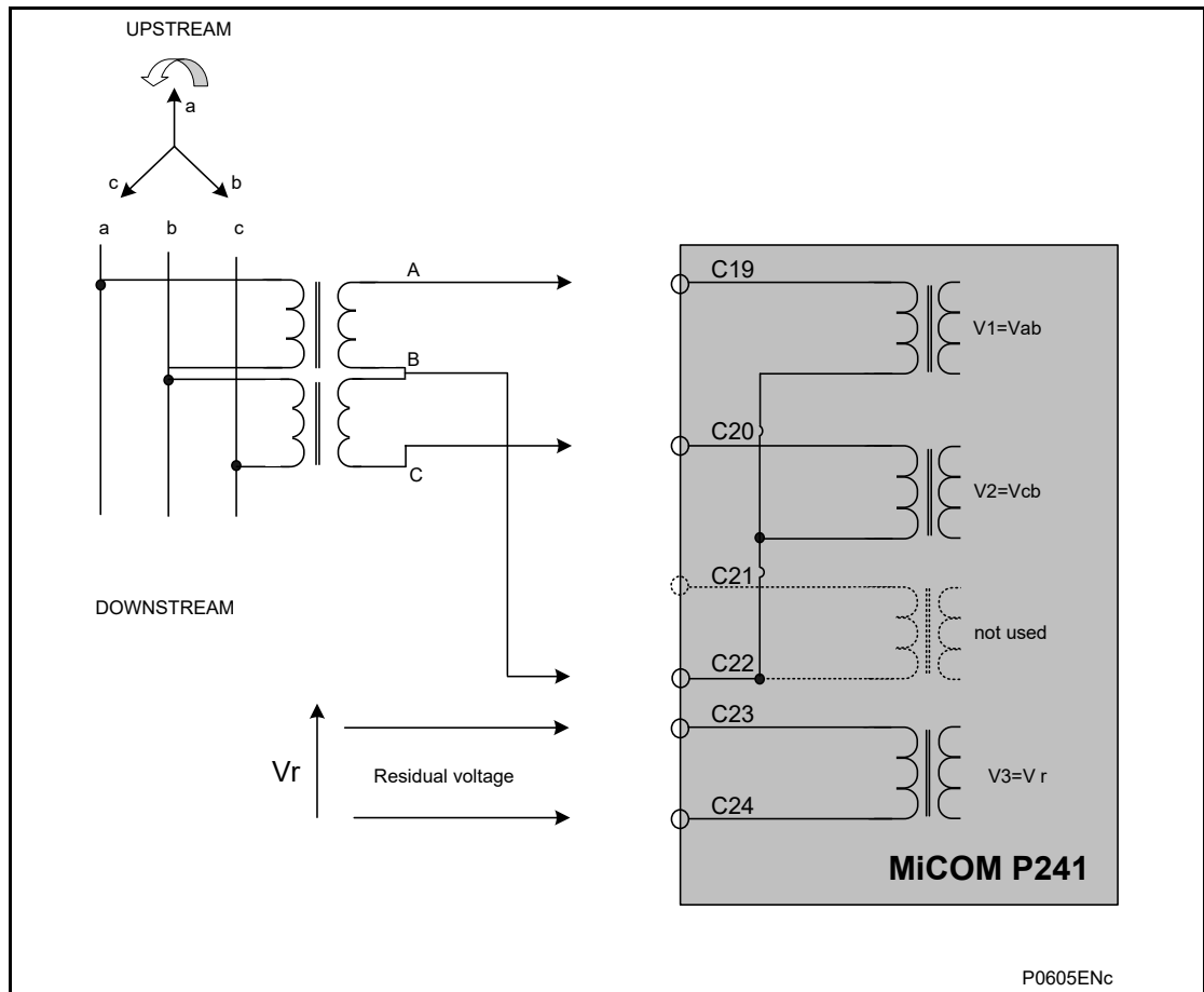
Figure 28: Alternative relay connections for residual overvoltage/NVD protection
