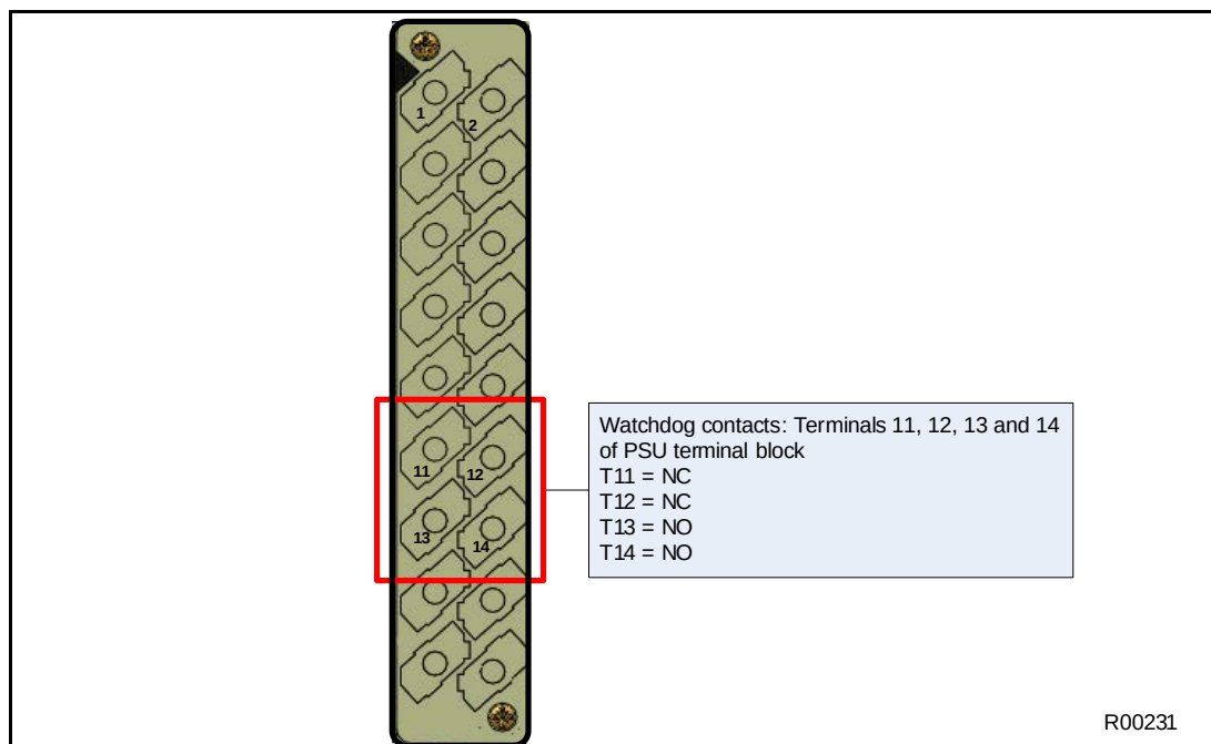
Figure 7: Watchdog contact terminals
