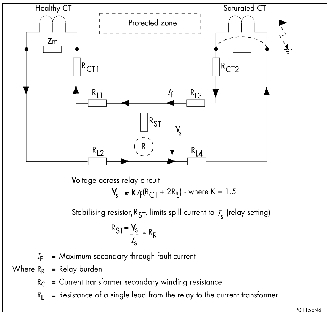
Figure 19: Principle of high impedance differential protection
