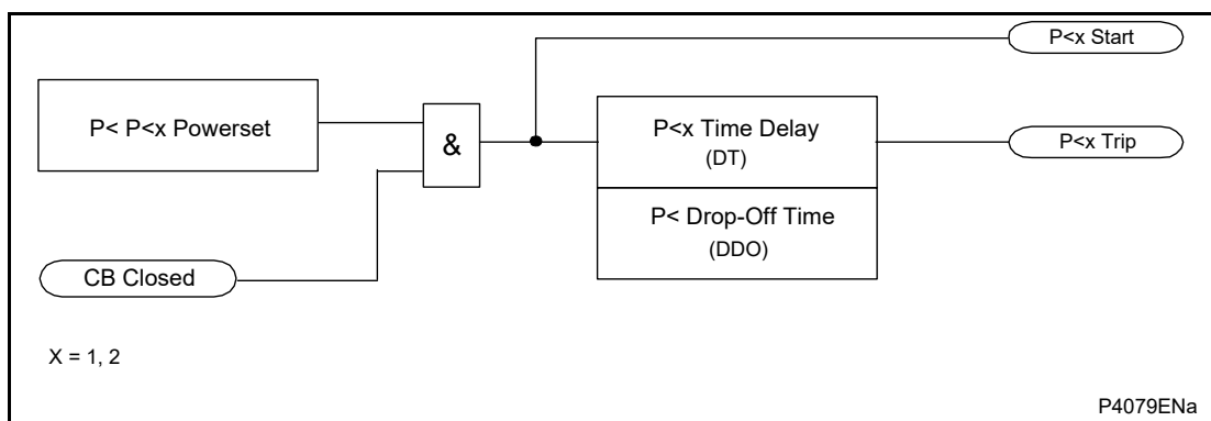
Figure 38: Loss of load logic diagram
