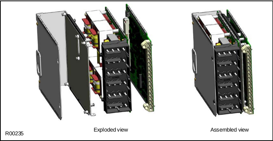
Figure 9: Input module – 1 transformer board
