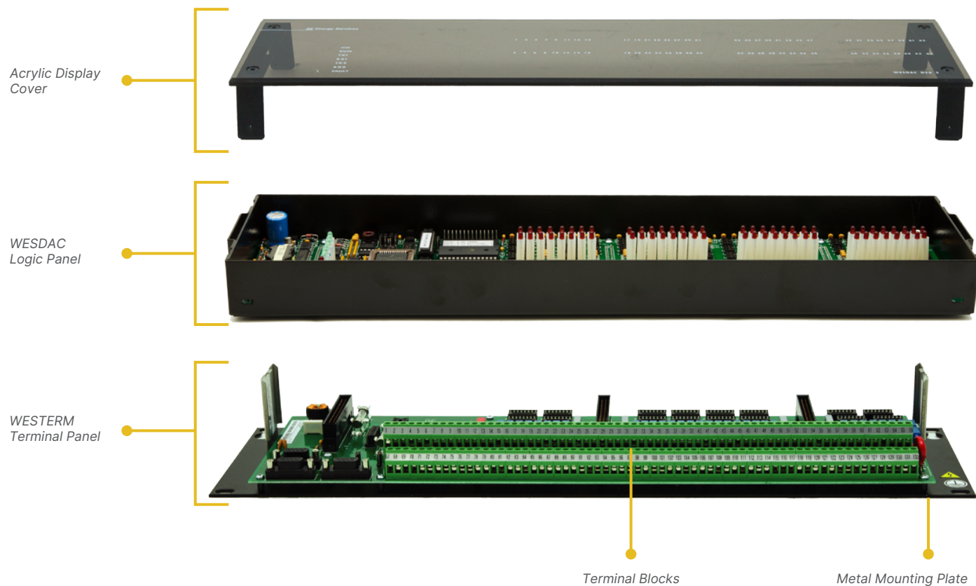
Figure 2: Architecture of I/O logic and termination panels
