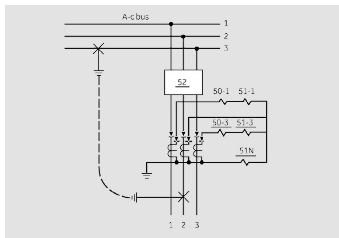
Figure 6. Elementary diagram of overcurrent relays used for phase- and ground-fault protection of three-phase circuit
