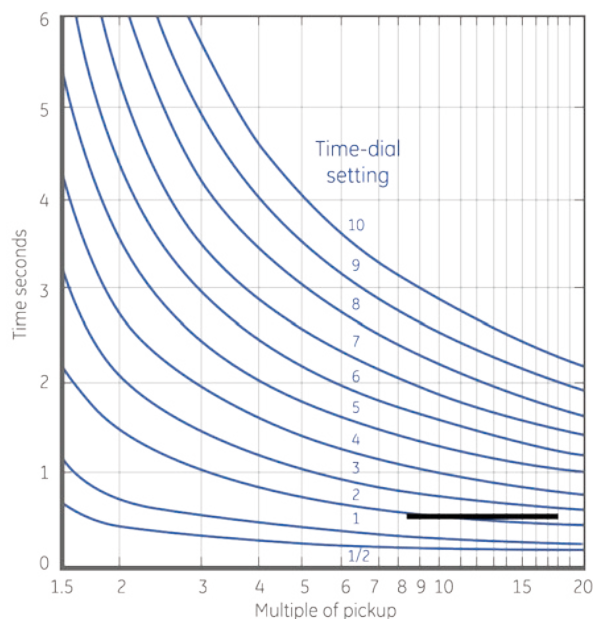
Figure 3. Inverse time curves
