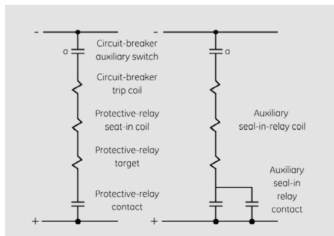
Figure 7. Alternative contact seal-in methods
