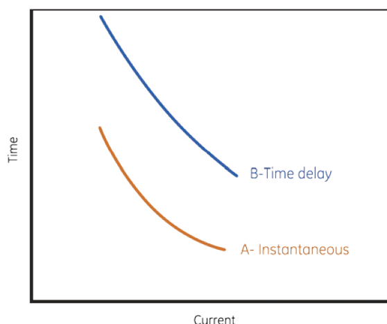
Figure 17. Tripping characteristic for conventional automatic circuit recloser
