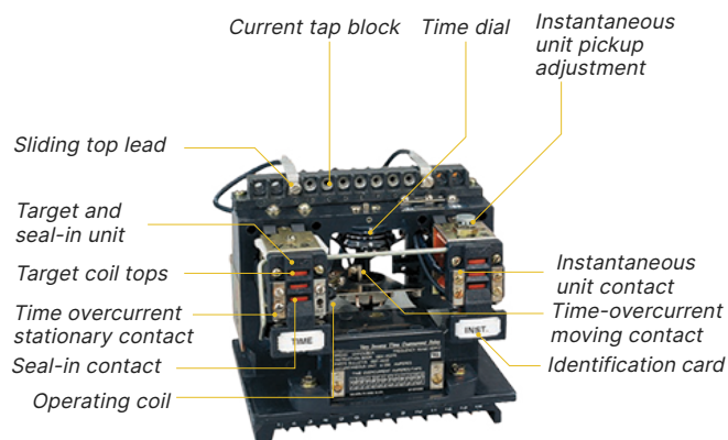
Typical IFC relay mechanism with standard hinged armature instantaneous unit withdrawn from case (model 12IFC53B1A)
