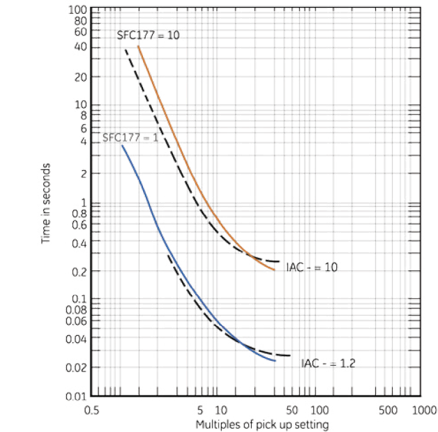
Figure 22. Comparison of extremely inverse time-current characteristics of SFC 177 and IAC 77 relays
