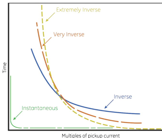
Figure 2. Time-current characteristics of overcurrent relays
