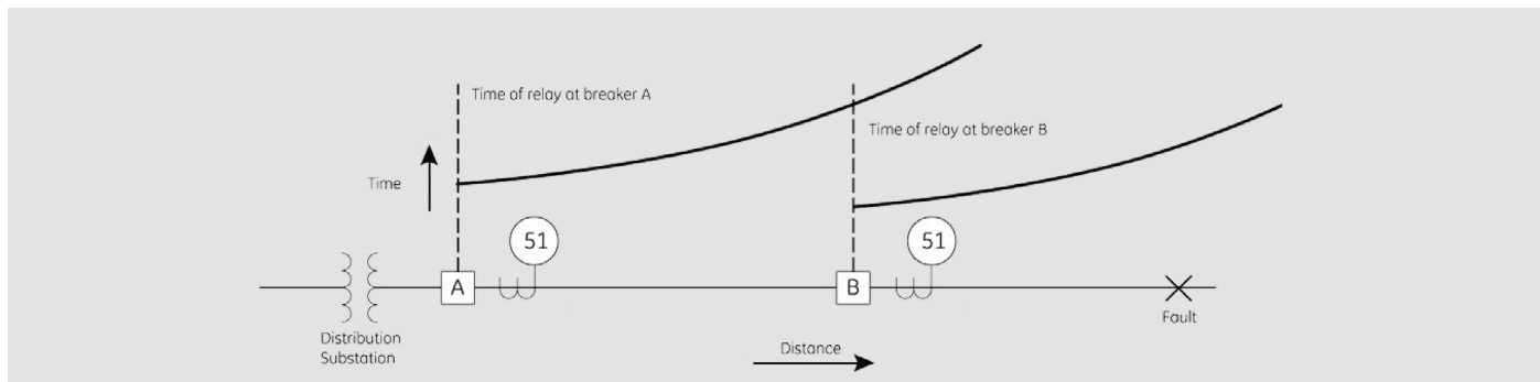
Figure 4. Operating time of overcurrent relays with inverse time characteristics
