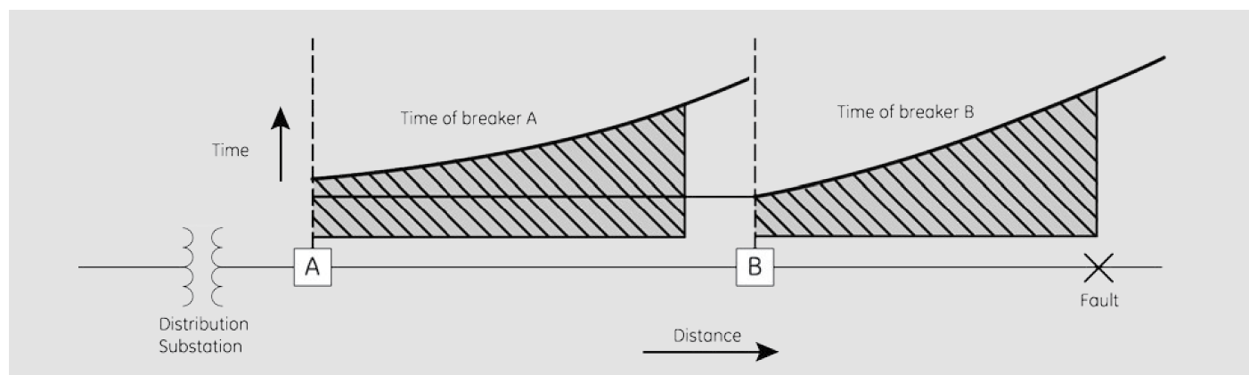
Figure 5. Reduction in tripping time using instantaneous relaying
