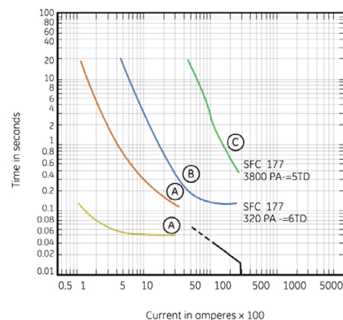
Figure 25. Pole-type recloser vs SFC 177 relay coordination example
