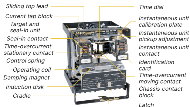
Typical IAC relay mechanism with standard hinged armature instantaneous unit withdrawn from case (Model 12IAC53BB10A)
