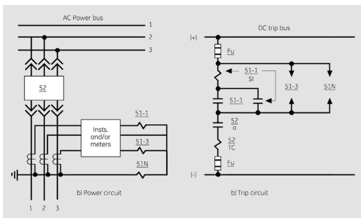
Figure 8. Elementary diagram of overcurrent relays used with DC battery tripping
