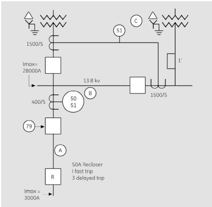
Figure 23. Sample system for recloser-relay coordination illustration
