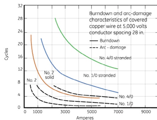
Figure 26. Burndown characteristics of several weatherproof conductors
