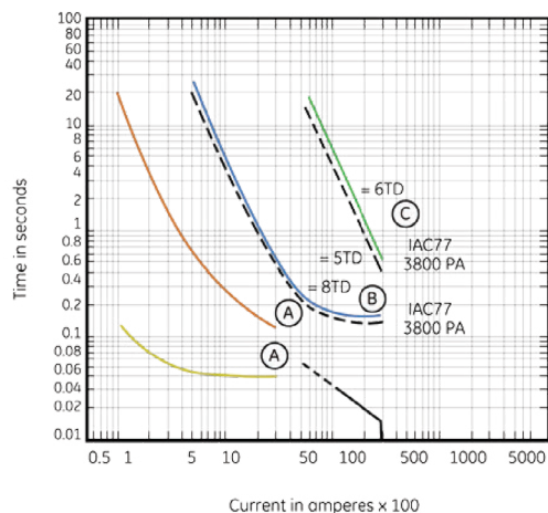
Figure 24. Pole-type recloser vs IAC 77 relay coordination example
