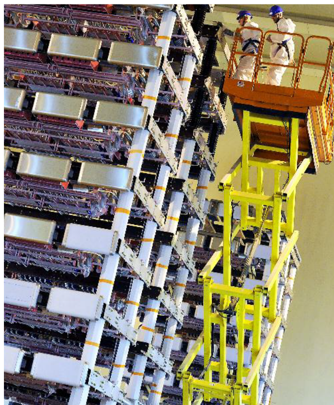
Valve stack during construction
