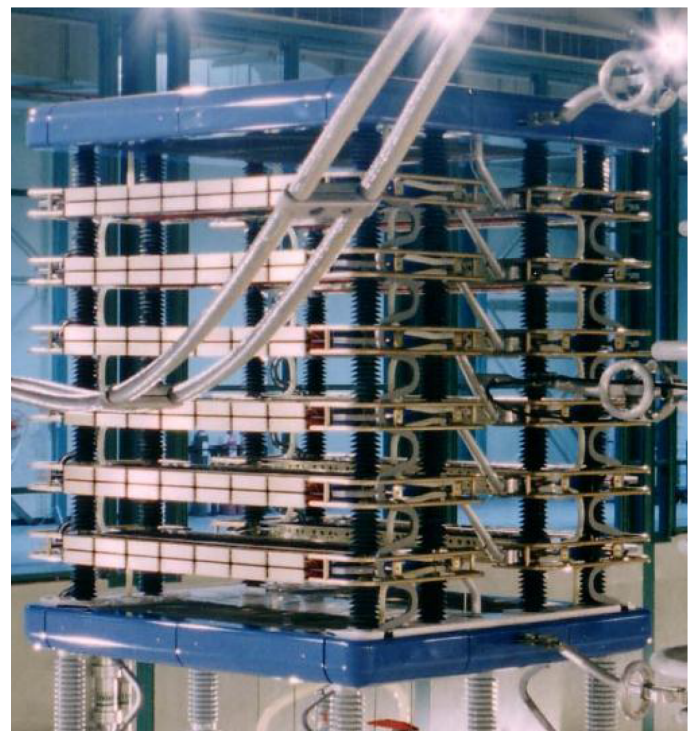
H400 valves
