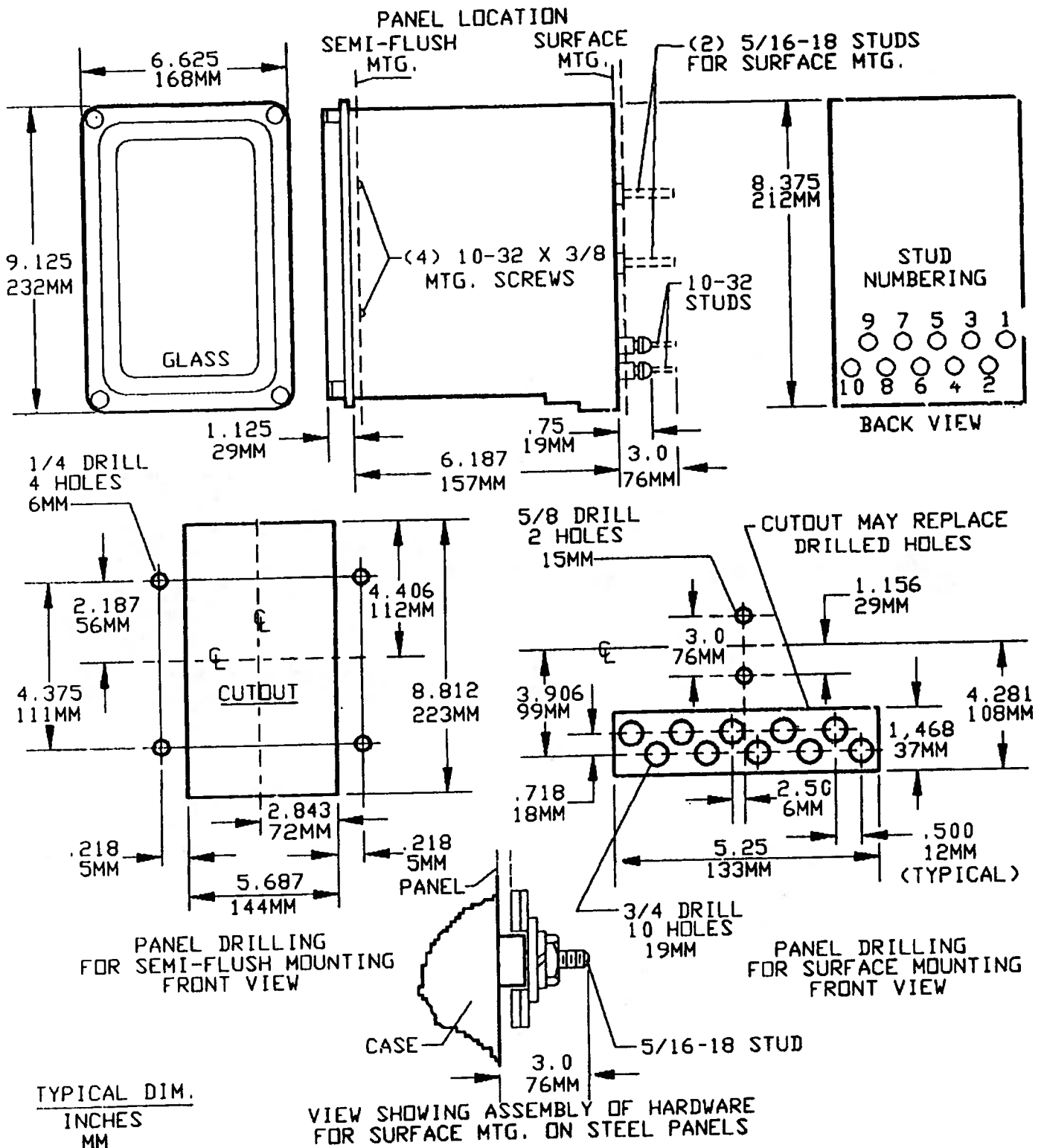
* Figure 19 (6209271 [8]) Outline and Panel Drilling for Drawout Relays - Size S1
