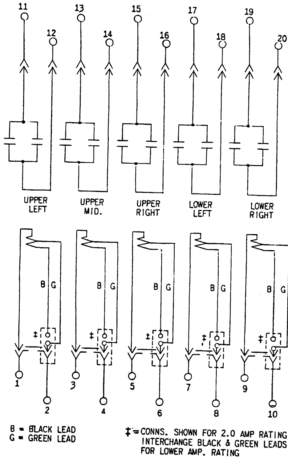
Figure 4 (0127A9439-0) Internal Connections of the HAA11A Relay (Front View)
