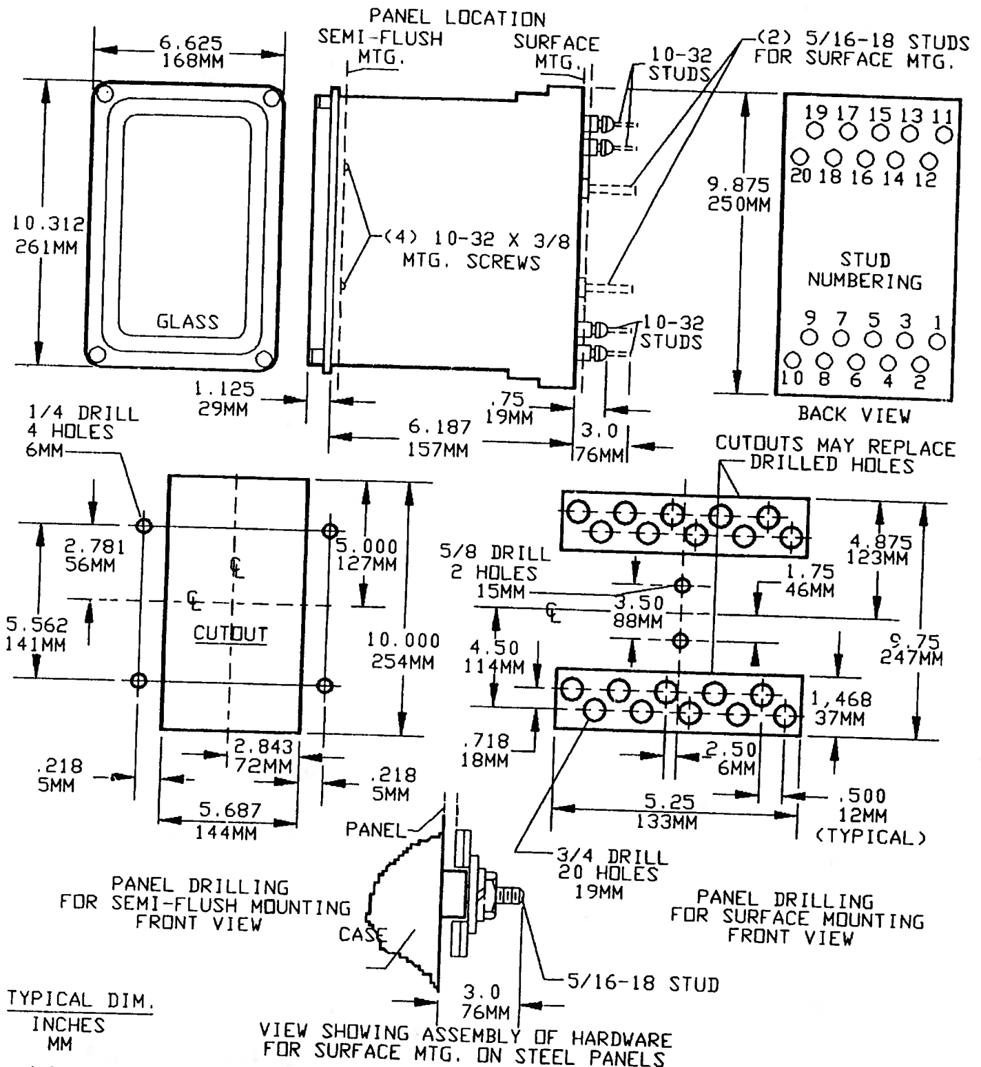
* Figure 20 (6209272[6]) Outline and Panel Drilling for Drawout Relays - Size S2
