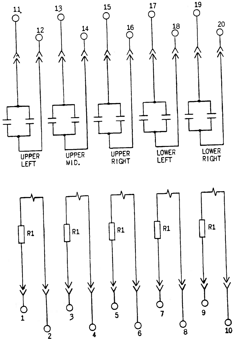
Figure 5 (0165A6086-1) Internal Connections of the HAA11B Relay (Front View)
