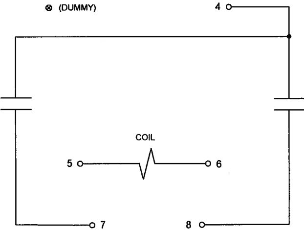
Figure 6 (0257A5083-0): HAA15D/15G INTERNAL CONNECTION DIAGRAM (BACK VIEW)
