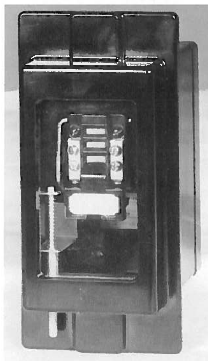
Figure 2 (8912917): HAA15 RELAY IN FLUSH MOUNTED CASE
