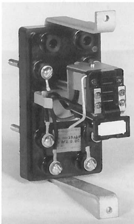
Figure 1 (8030184): HAA15 RELAY REMOVED FROM CASE
