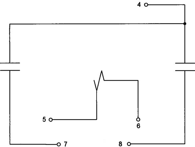
Figure 5 (0195A9121-0): HAA15C INTERNAL CONNECTION DIAGRAM (BACK VIEW)
