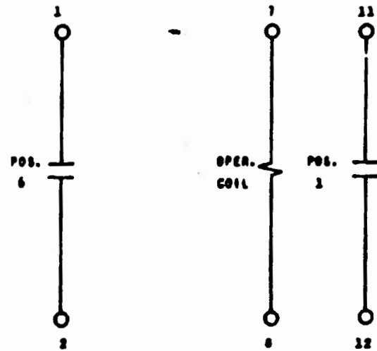
Fig. 2 Internal Connections For NFA60 Relays (Back View)
