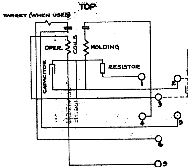
FIG. 4 INTERNAL CONNECTION DIAGRAM FOR TYPE HGA18C RELAY - UNIVERSAL CASE
