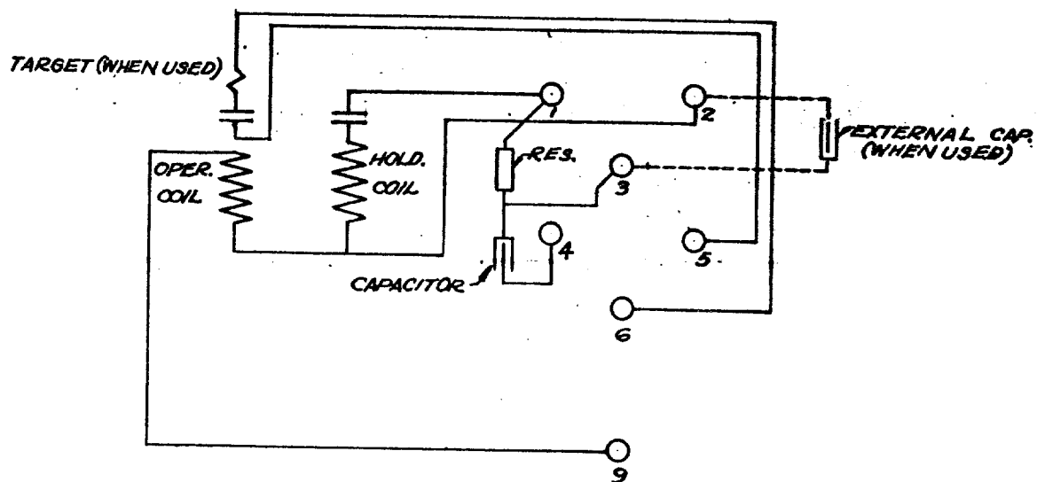
INTERNAL CONNECTIONS (BACK VIEW)
