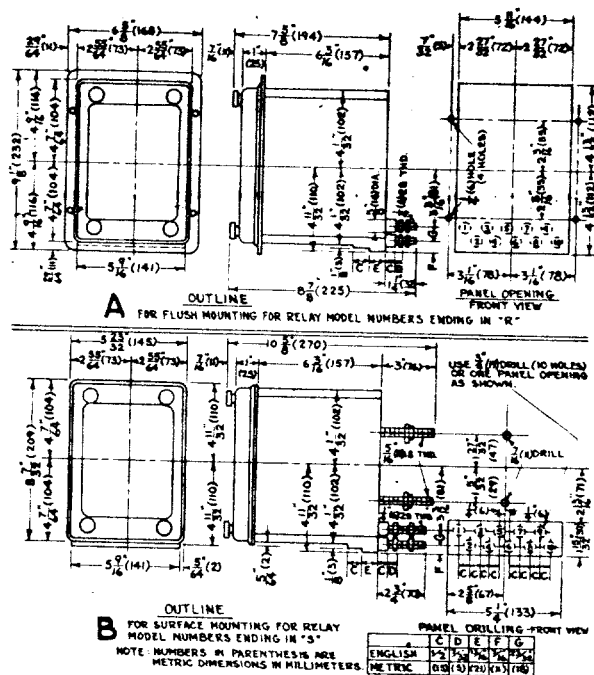
FIG. 2 OUTLINE AND PANEL DRILLING FOR TYPE HGA18A AND HGA18B (D.C.) RELAYS - DRAWOUT CASE. ONE UNIT-SINGLE END.
