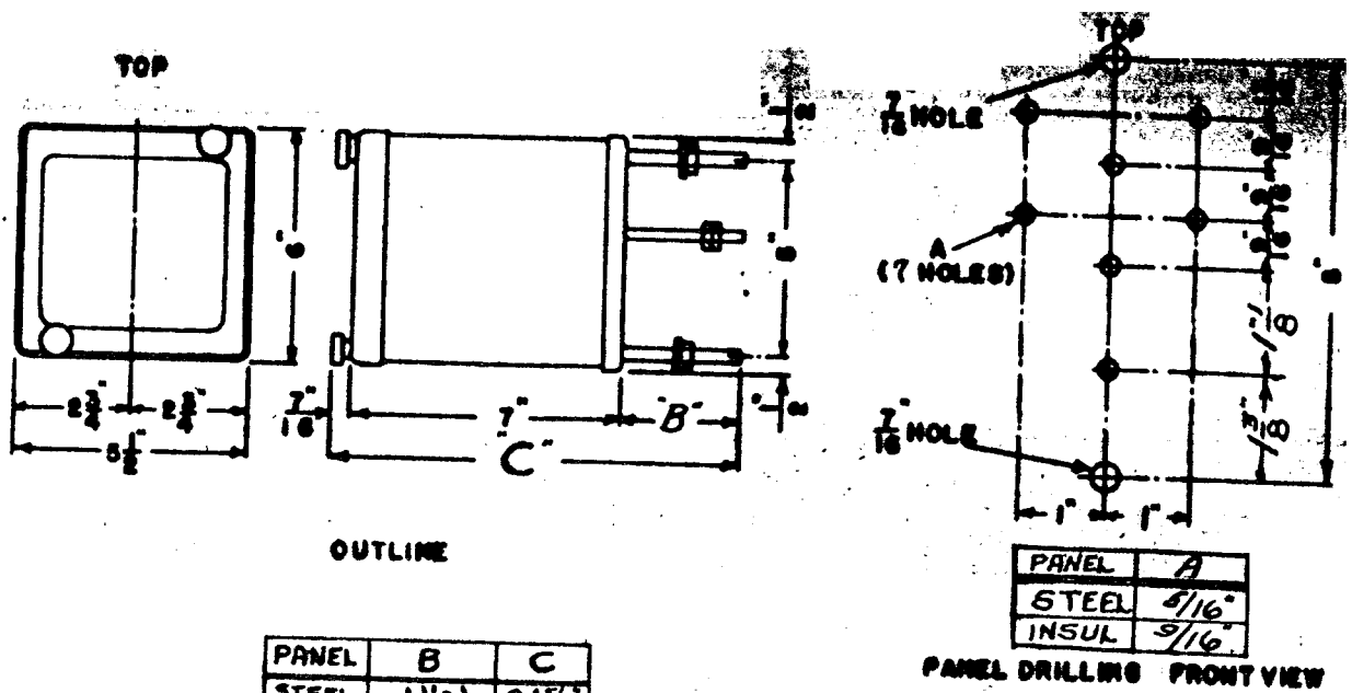
FIG. 1 OUTLINE AND PANEL DRILLING FOR TYPES HGA18A, HGA18B, HGA18C AND HGA18D RELAYS. (UNIVERSAL CASE)
