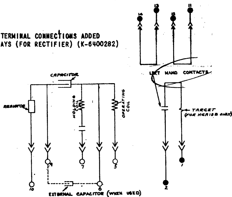
FIG. 5 INTERNAL CONNECTIONS FOR TYPES HGA18A AND HGA18B RELAYS. DRAWOUT CASE
