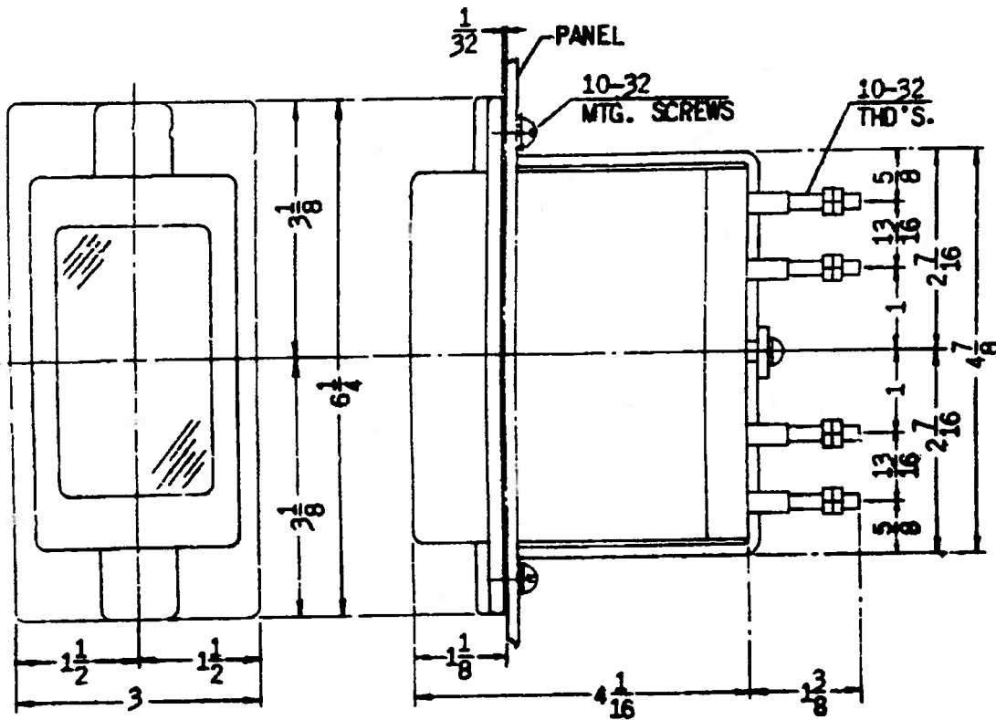
Figure 3 (0104A8557-2) Outline Dimensions for the HGA14A(-)F Semi-flush Mounted Relay
