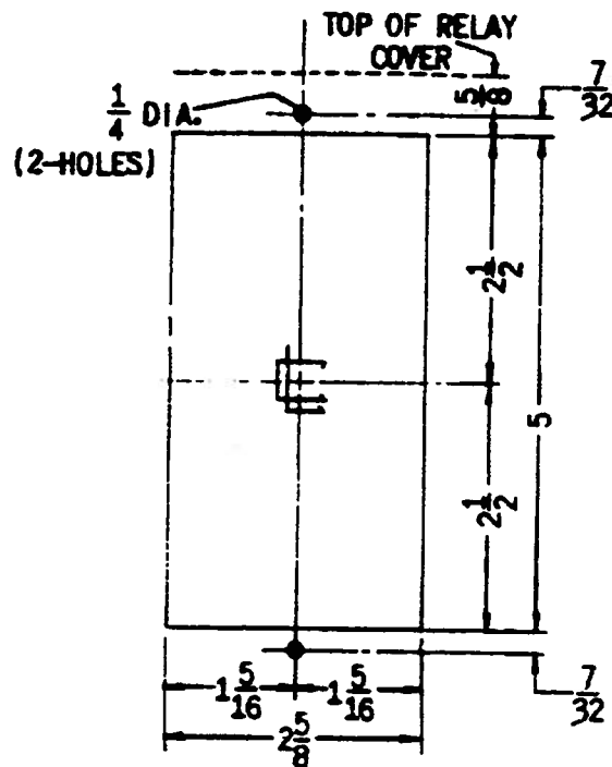
Figure 9 (0104A8557-2) Panel Drilling Diagram for HGA14A(-)F Relay (Front View)
