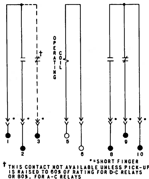
Fig. 1 Internal Connection Diagram for Type HGA17J Relay.
