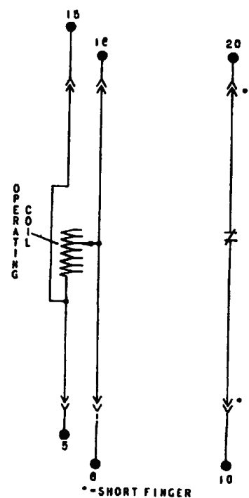
Figure 8 (K-6556476) Internal-Connection Diagram for Type-IAV53L and -IAV53N Relays
