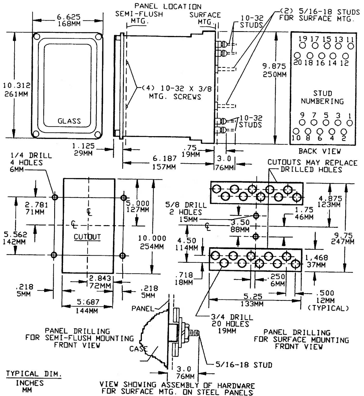
FIG. 8 (K6209272 [7]) OUTLINE AND PANEL DRILLING DIMENSIONS FOR THE IAV73A AND IAV73B RELAYS
