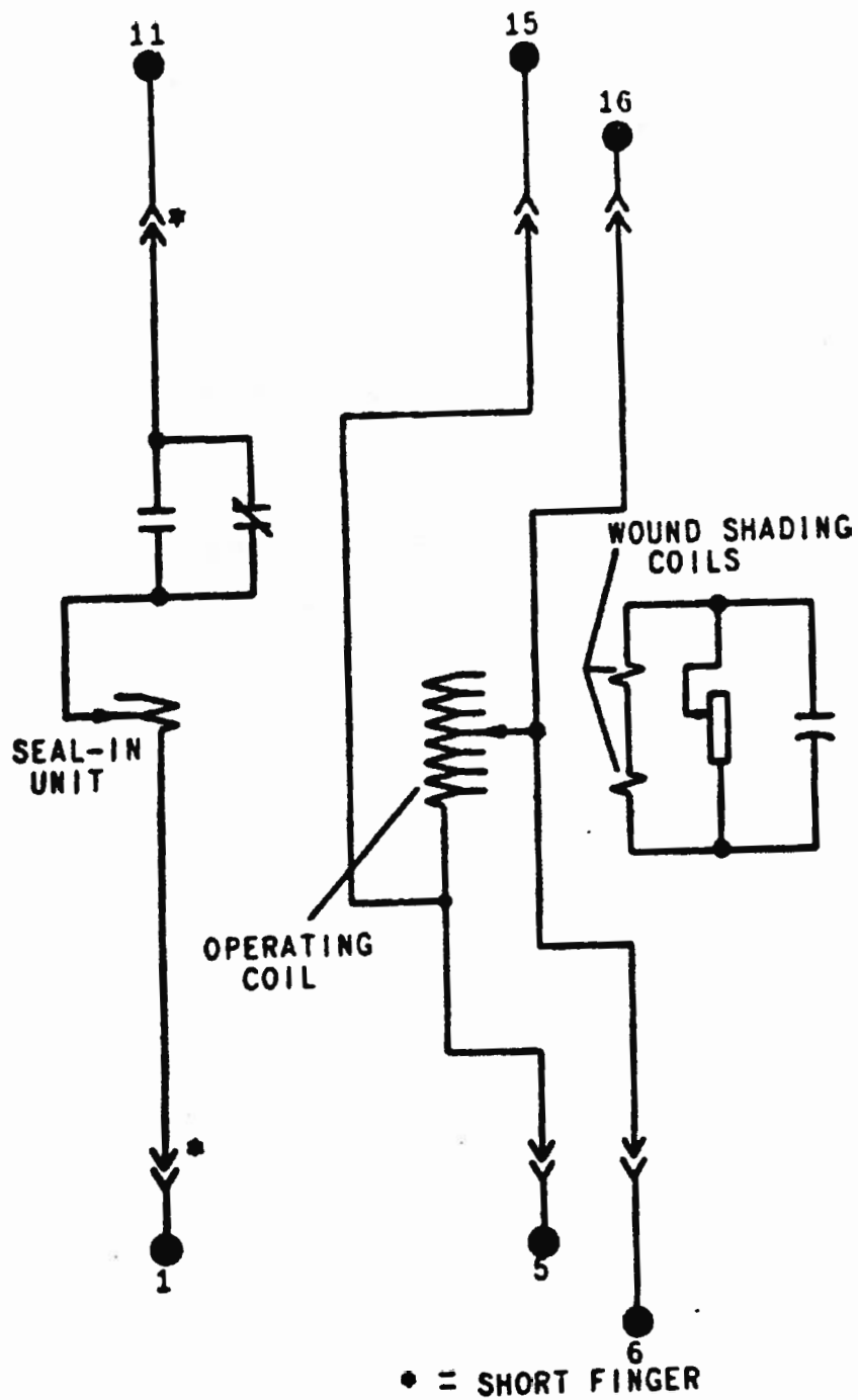
Figure 1 (362A524-1) Internal Wiring Diagram of IAV74A Relay (Front View)
