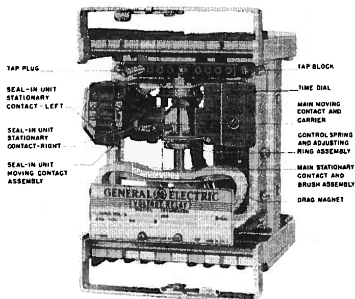
Figure 10 (8007475) Type IAV54E Relay Removed from Case (Front View)
