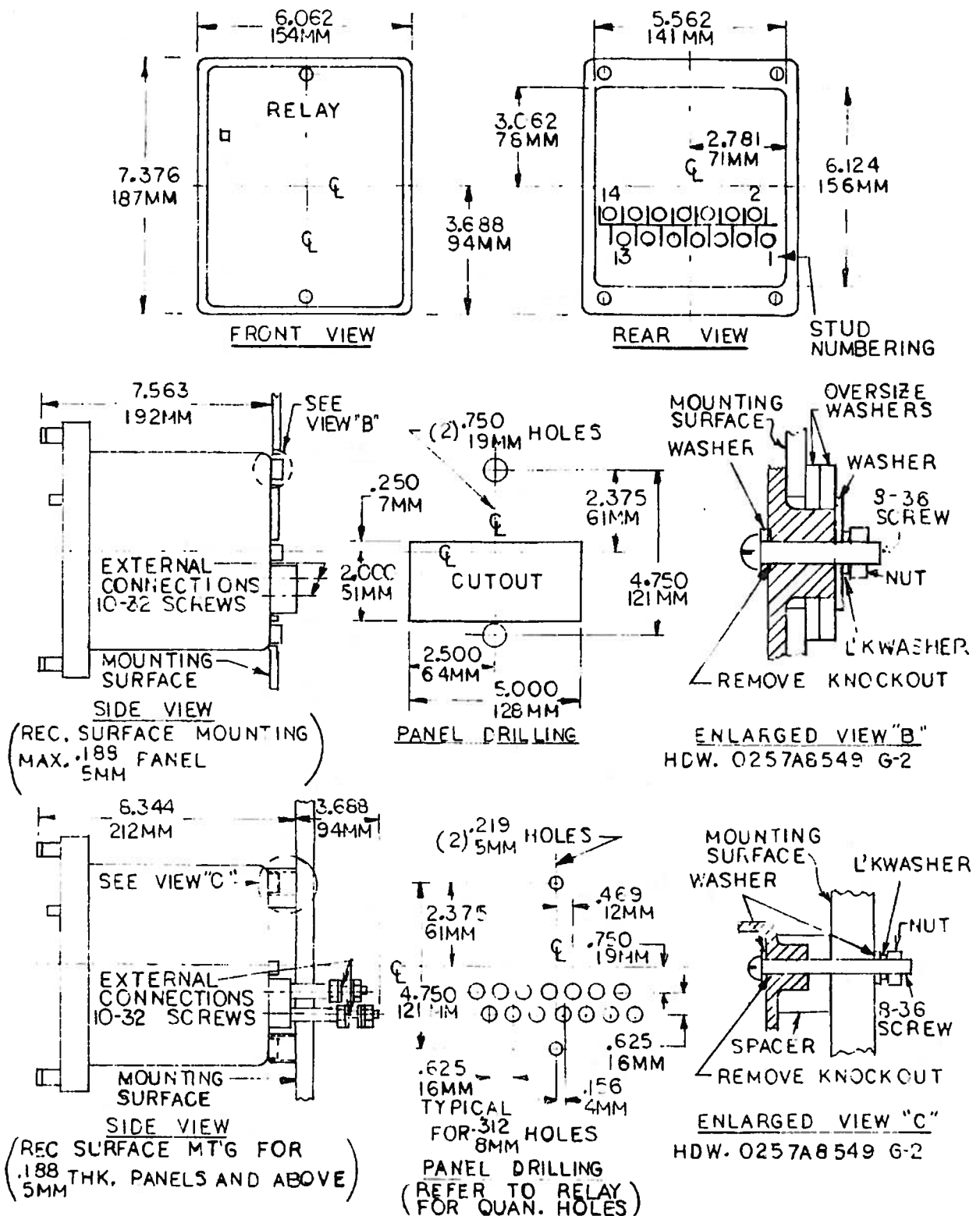
*Figure 17 (0257A8452 Sh.2 [3]) Outline and Panel Drilling for Surface Mounting of Relay Type IFC57
