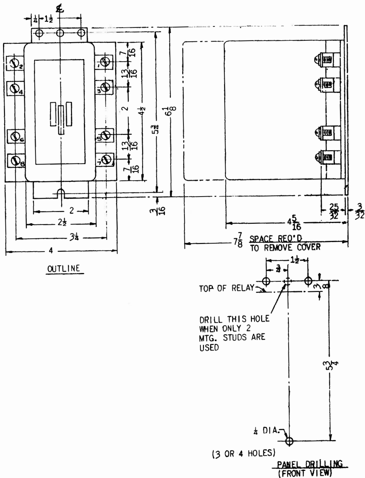
Figure 8 (0208A3642-1) Outline and Panel Dimensions for the Front Connected NGA15L with Solid Front Cover
