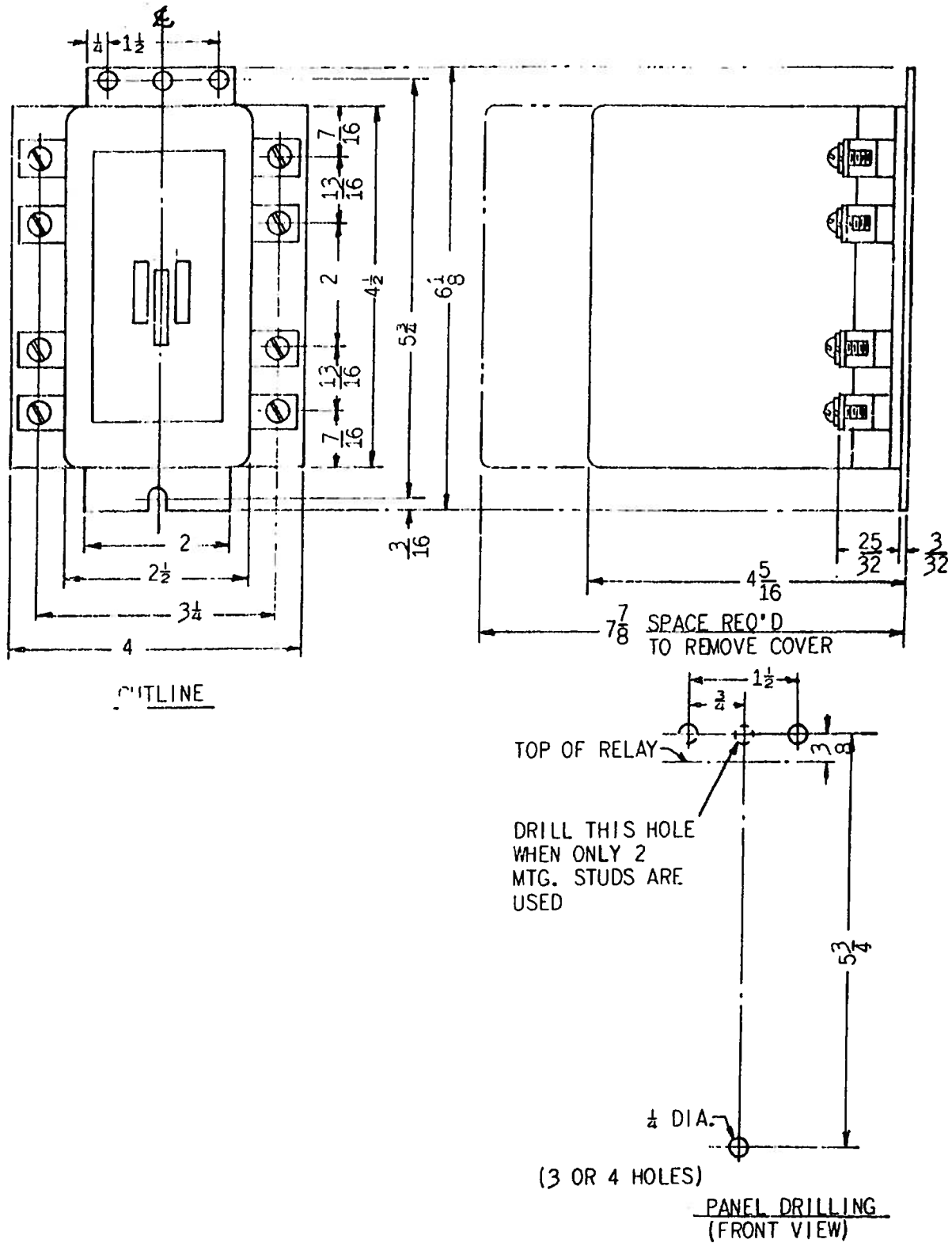
FIG. 2 (0208A3642-0) Outline, Panel Drilling For The NGA15X1 Relay
