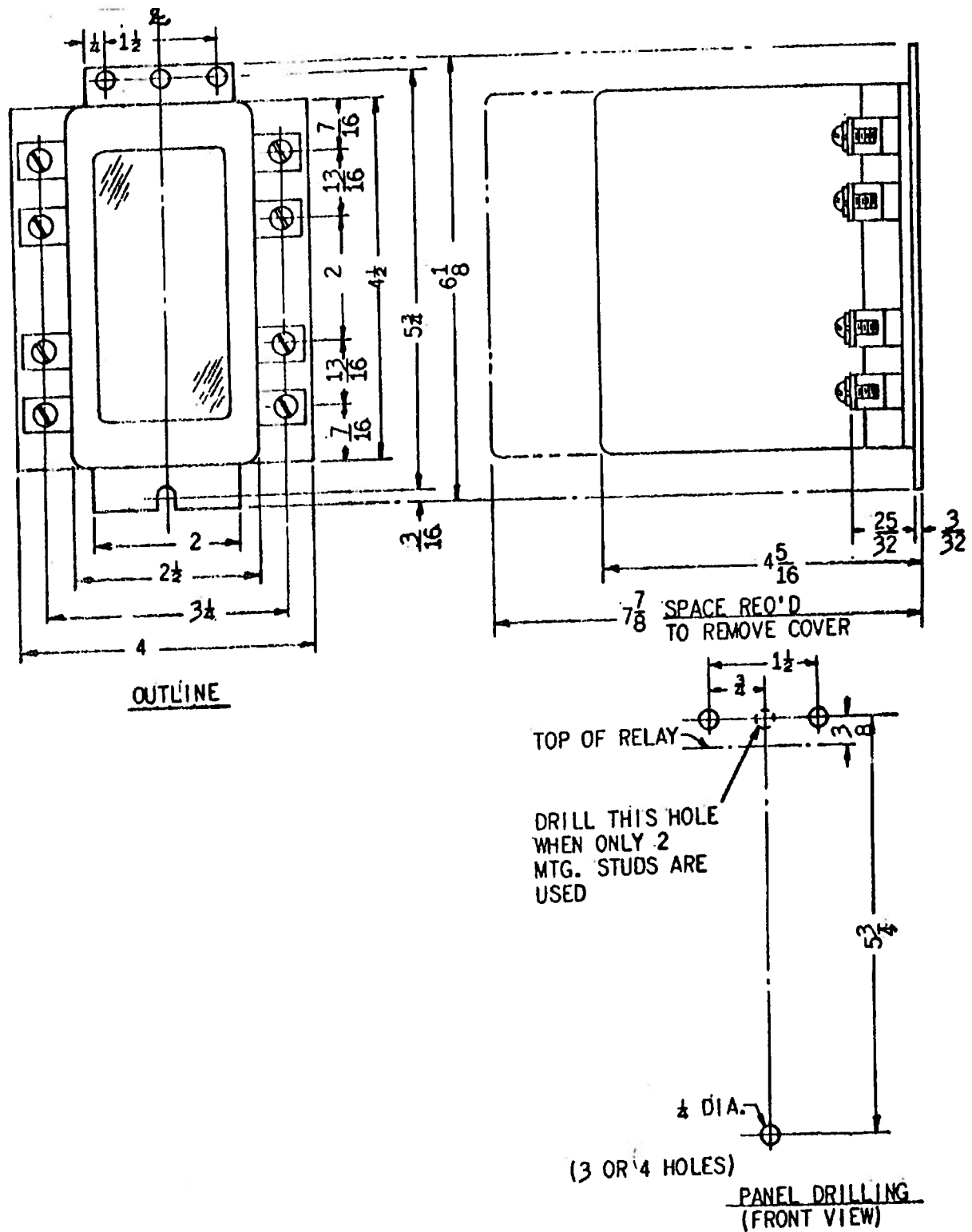
FIG. 3 (0208A3643-0) Outline, Panel Drilling For The NGA15X1 Relay
