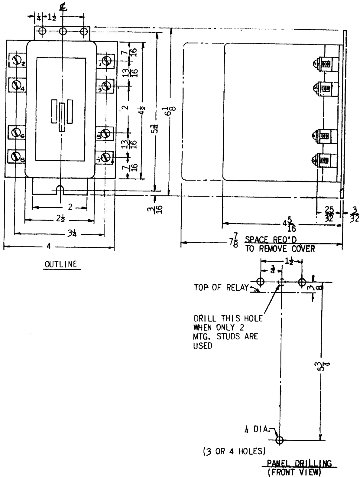
Figure 8 (0208A3642-1) Outline and Panel Dimensions for the Front Connected NG15L with Solid Front Cover
