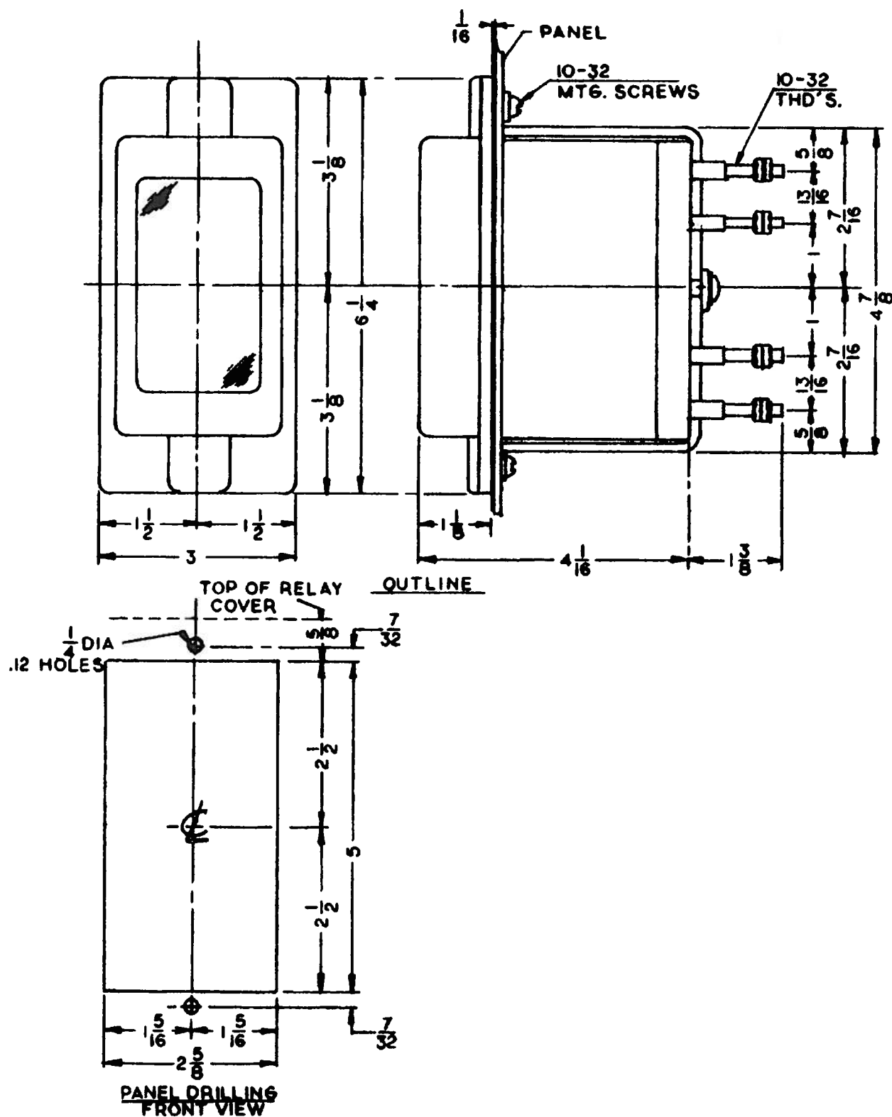
Figure 6 (0148A3978-7) Outline and Panel Drilling Dimensions for the Semi-Flush Mounted NGA15A Relay
