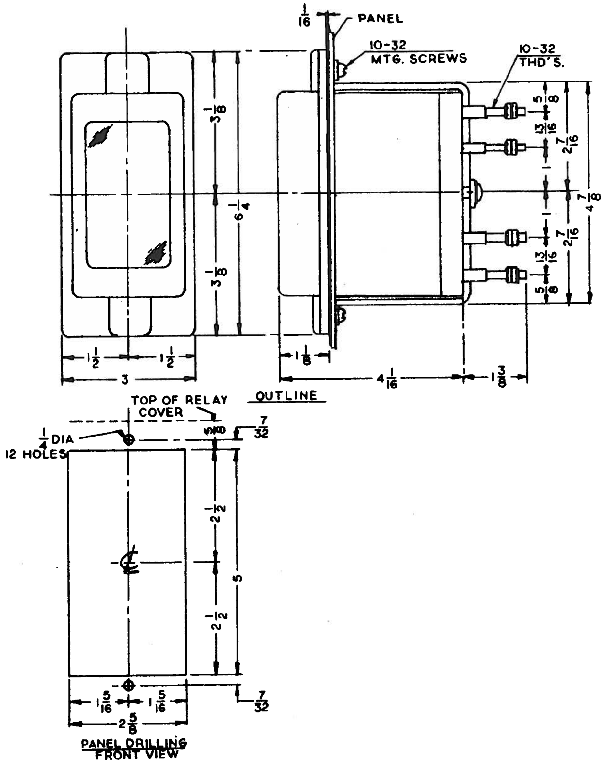
* Figure 2 (0148A3978-7) Outline and Panel Drilling Dimensions for the Semi-Flush-Mounted NGV15A Relay
