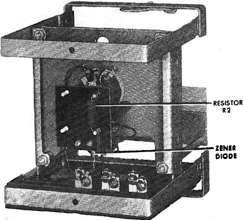
Fig. 2 (8035275) NGV18A Relay Removed From Case (Rear View)
