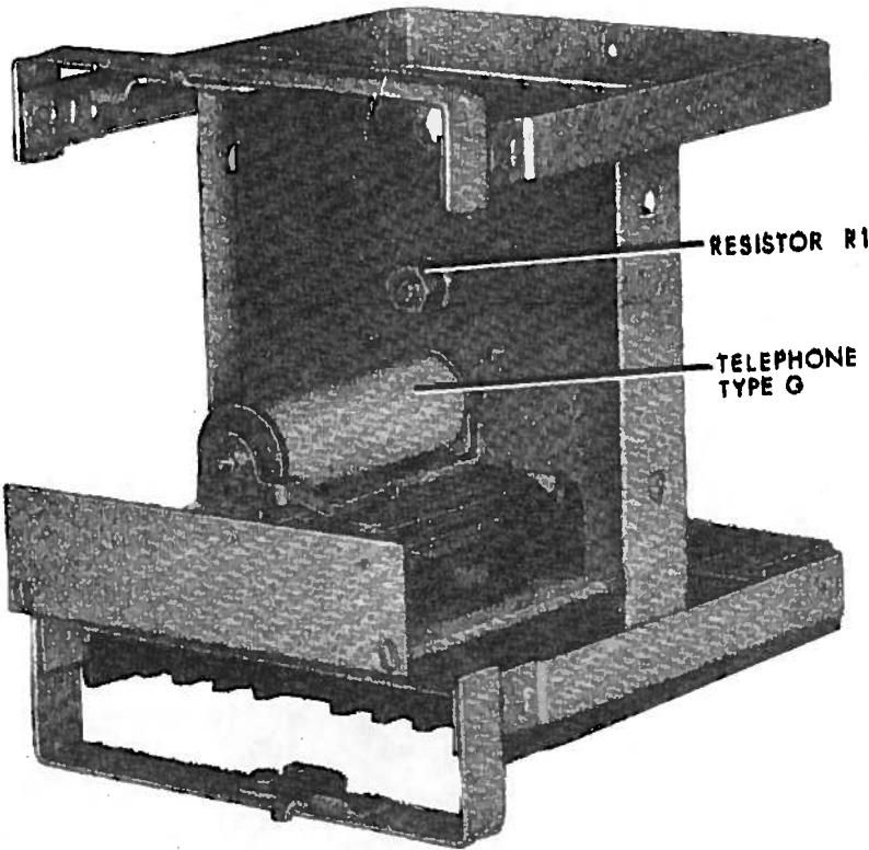
Fig. 1 (8035274) NGV18A Relay Removed From Case (Front View)
