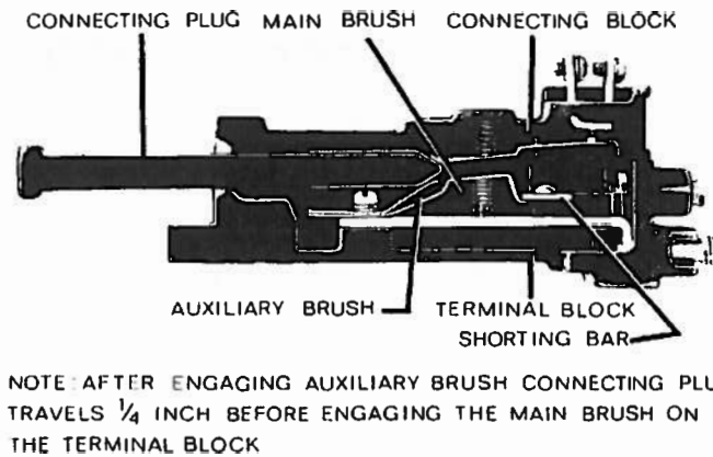
Figure 1 (8025039) Cross Section of Drawout Case Showing Position of Auxiliary Brush
