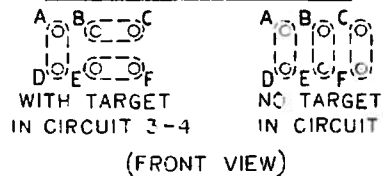
Figure 8A (0275A4380-1) Internal Connections Diagram for the NGV13B-Revision A Relay (Front View)
