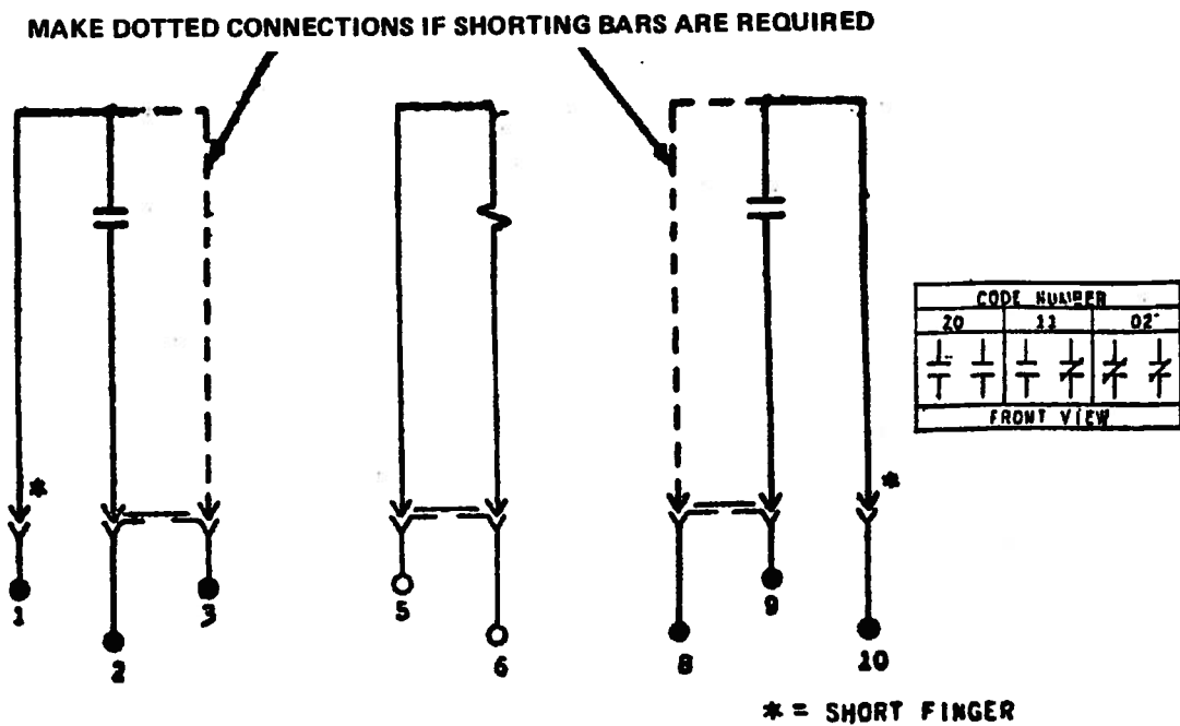
Figure 3 (K-6375600-4) Internal Connections for Type PJC11AV and PJC12D Relays (Front View)
