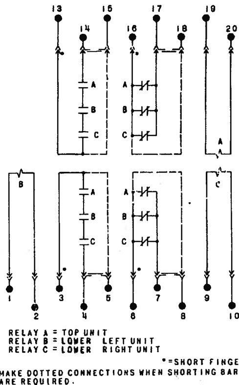
Fig. 23 Internal Connections for Type PJVI4D Relay
