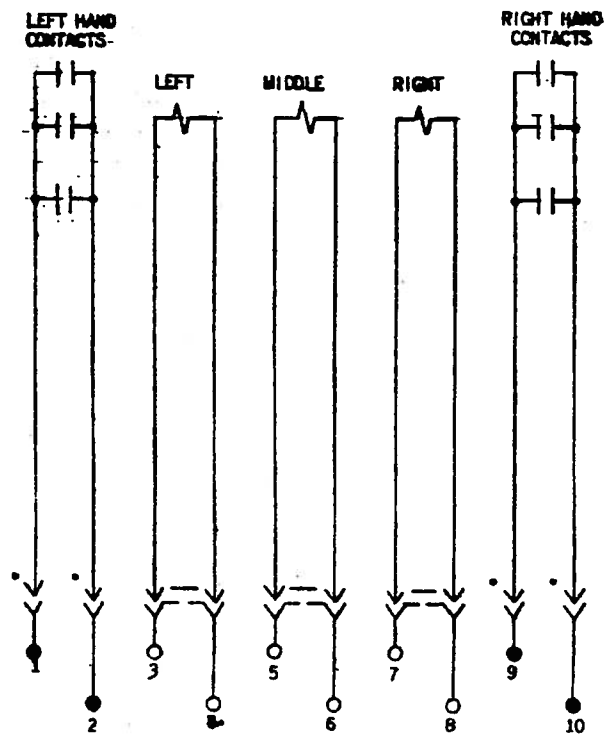
Fig. 9 Internal Connections for Type PJC11AR Relay
