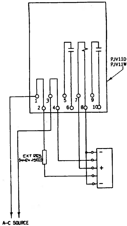
Fig. 4 External Connections for Type PJV11W Relay
