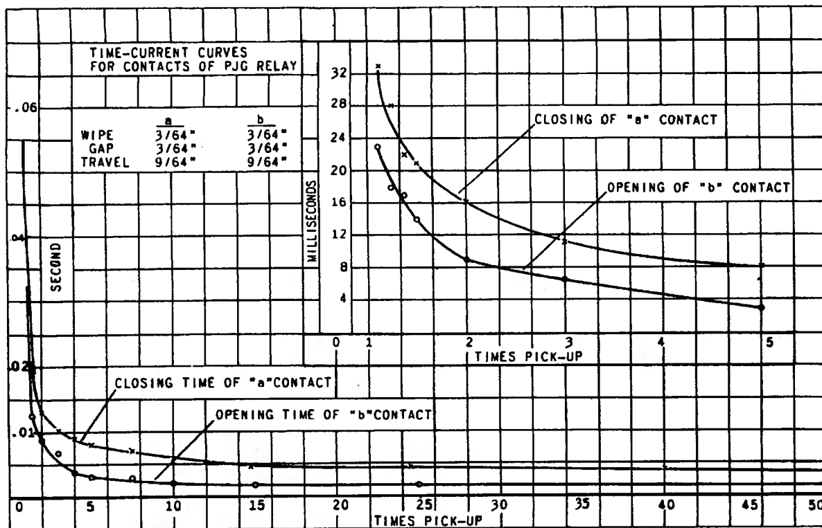
Fig. 1 Time-Current Curves For Type PJC Relays
