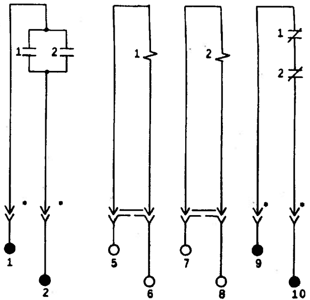
Fig. 9 Internal Connections for Type PJC11AR Relay
