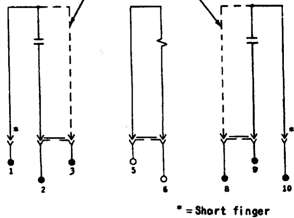
Fig. 7 Internal Connection for Type PJC11AH Relay
