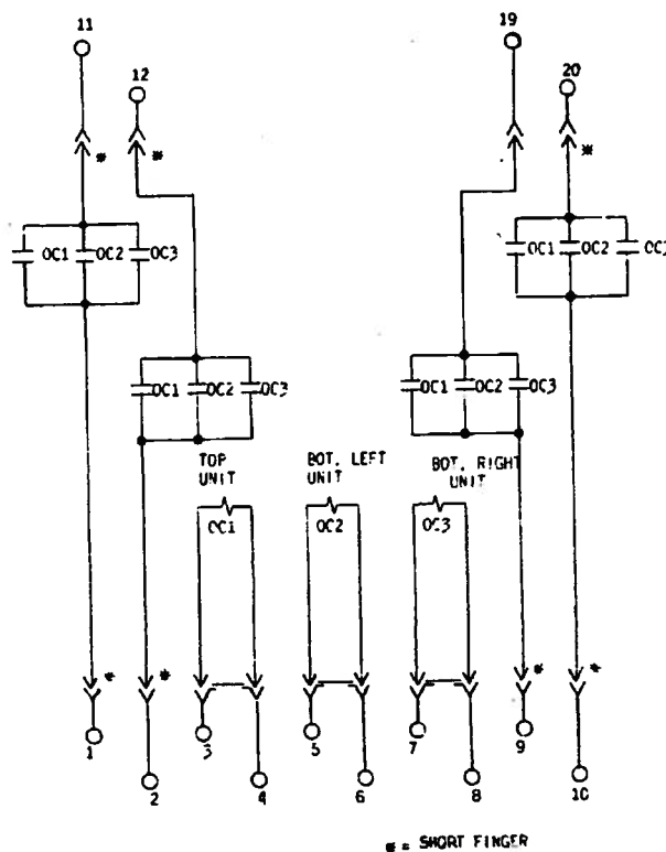
Fig. 15 Internal Connections for Type PJC15F Relay
