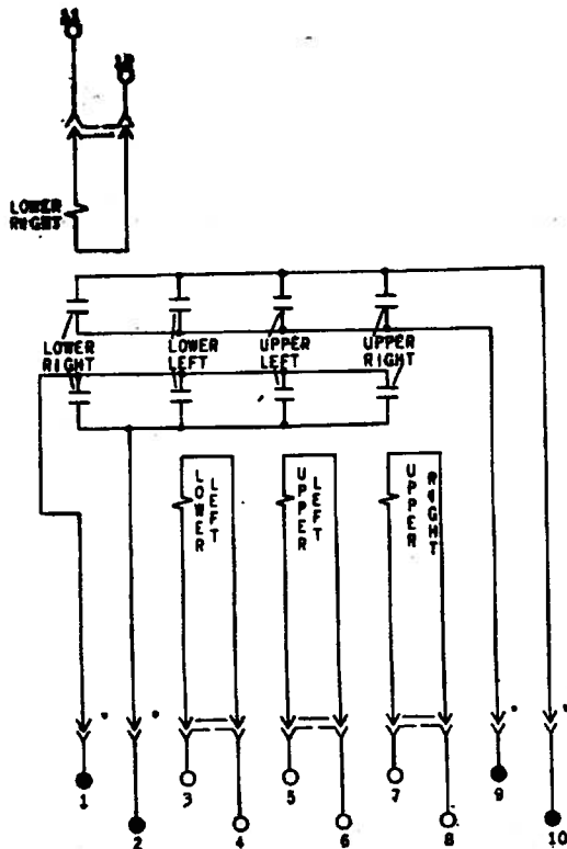
Fig. 6 Internal Connections for Type PJC11AD Relay
