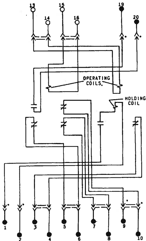
Fig. 18 Internal Connections for Type PJC16A Relay
