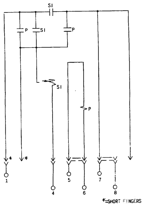
Fig. 19 Internal Connections for Type PJC21A Relay
