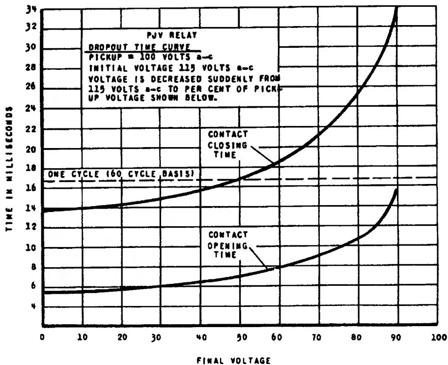
Fig. 2 Dropout-Time Curves For Type PJV Relay
