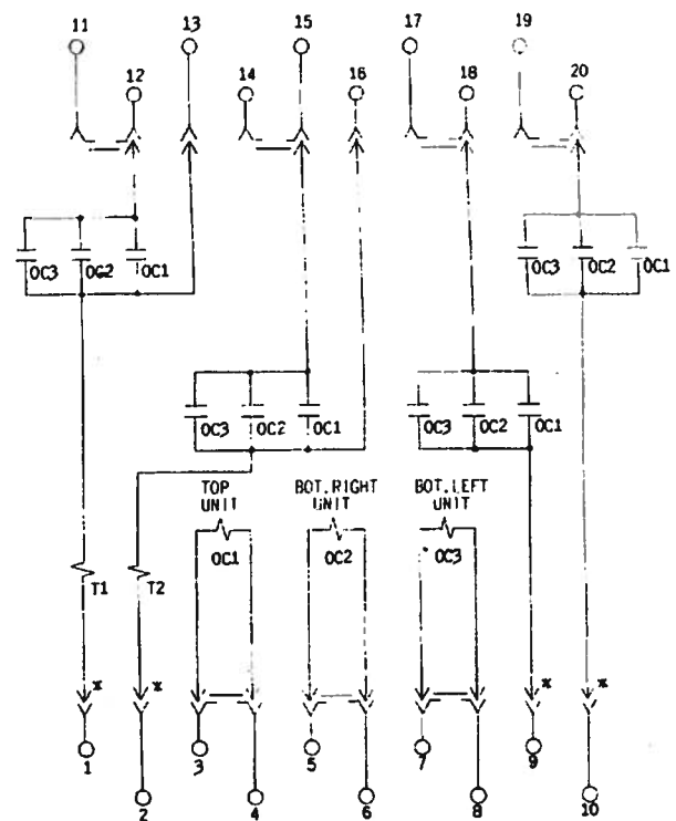
Fig. 17 Internal Connections for Type PJC15E Relay
