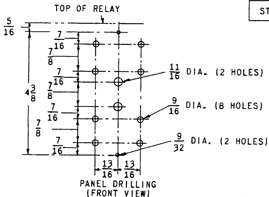
Figure 4 (6375721-0) Outline, Panel Drilling and Internal Connections Diagram for Type PJC20A Relay
