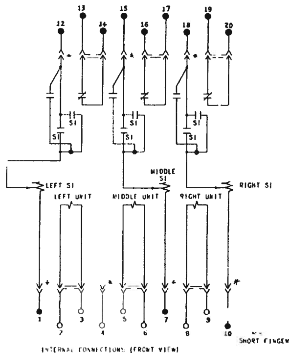
Figure 6 (6375727-4) Internal Connections Diagram for the PJC32D Relay (Front View)
