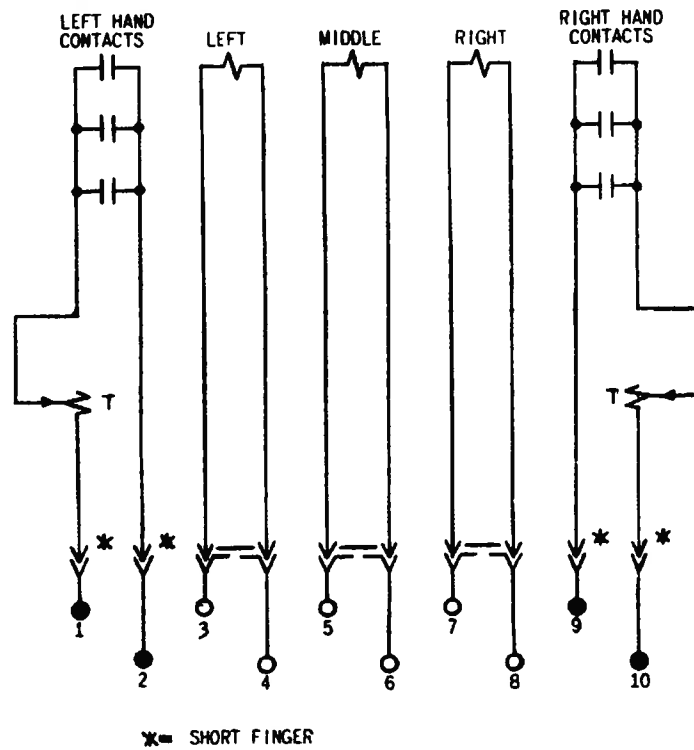
Figure 13 (0127A9547-2) Internal Connections Diagram for the PJC32L Relay (Front View)
