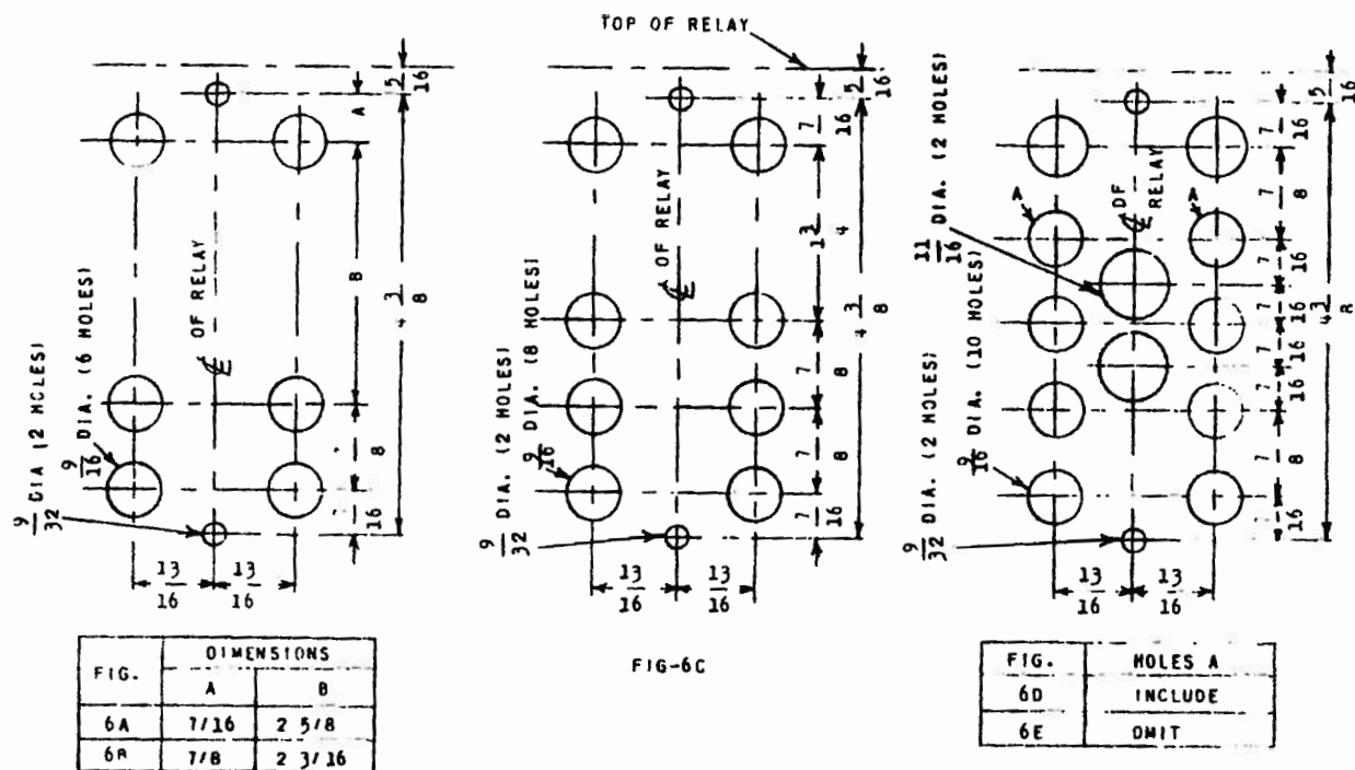
Figure 6. (376A945-1) Panel Drilling Dimensions of the Type PJC Relays.
