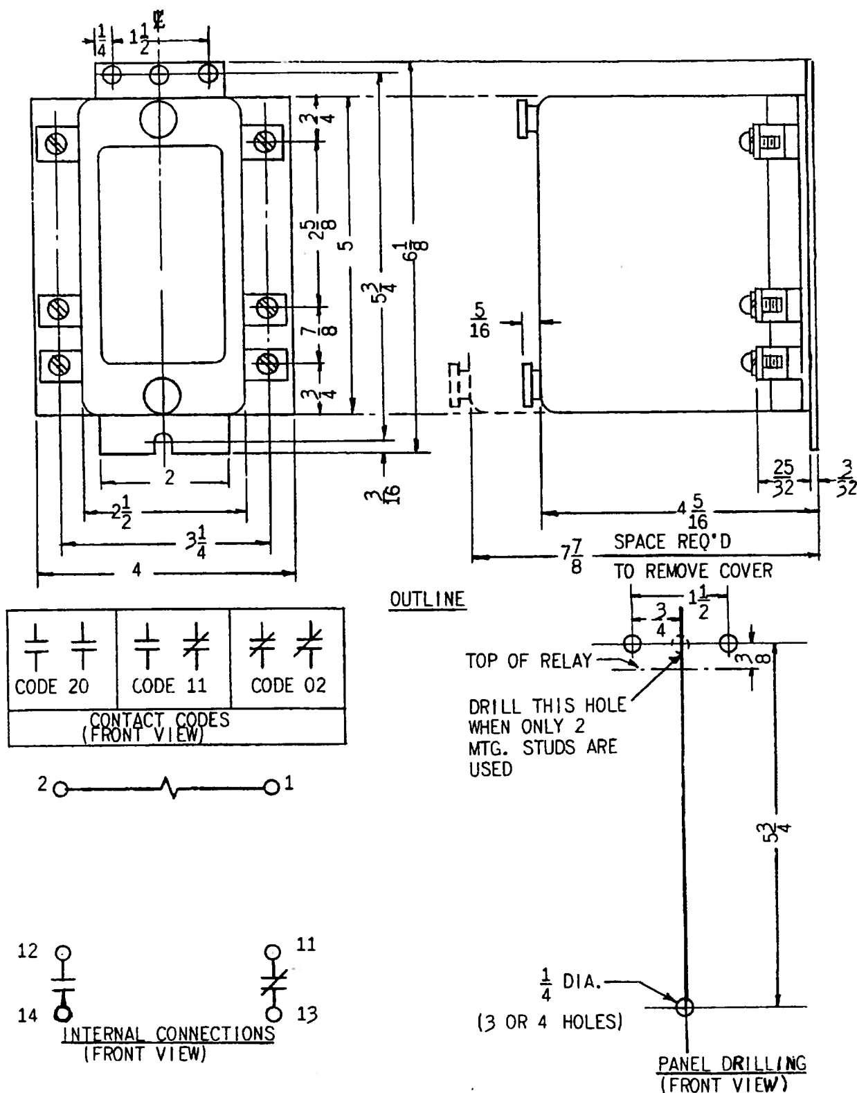
FIG. 1 (0165A7526-1) Outline And Panel Drilling Dimensions For Relay Type PJC11BA.
