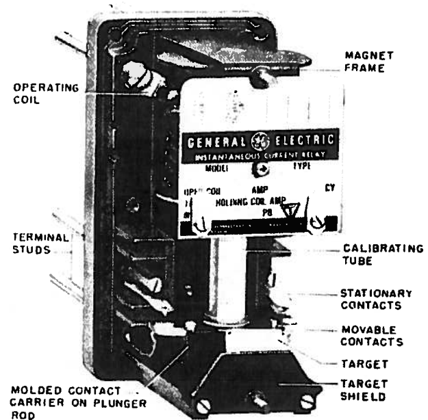
Fig. 3 Type PJC11A Relay Without Cover (Front View)
