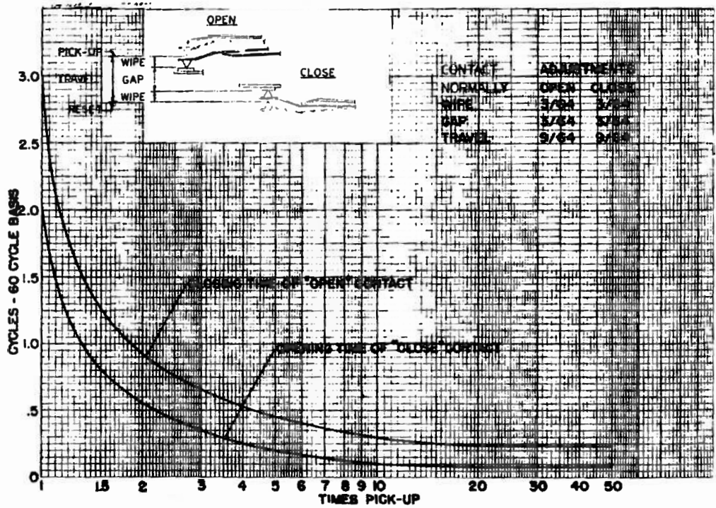
* Figure 2. (418A711-1) Time-Current Curves for Type PJC Relays.
