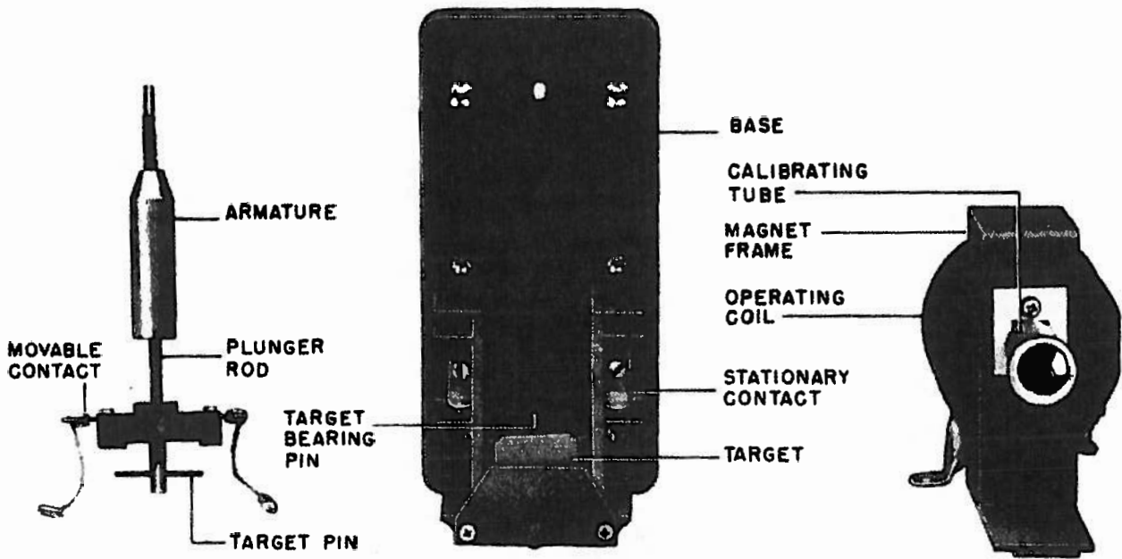
Figure 1. (8014170) Type PJC11A Relay Disassembled (Cover Not Shown)
