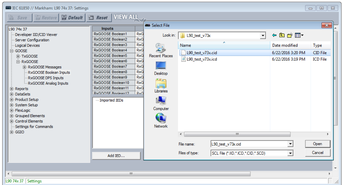
Figure 41: RxGOOSE Boolean Input panel (Edition 2)
