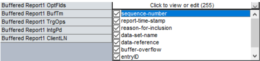
Figure 46: Options for buffered report messages (Edition 2)
