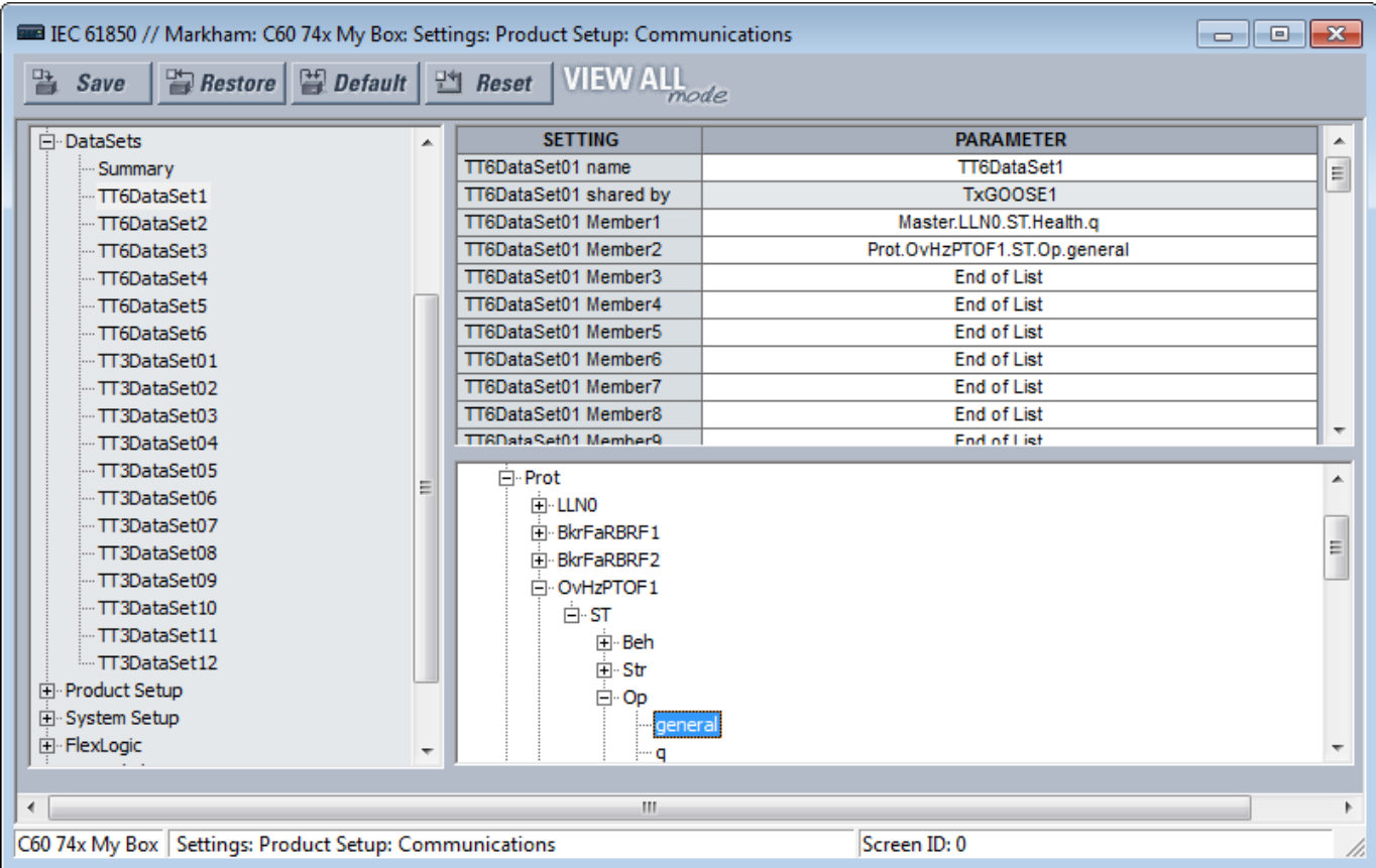
Figure 47: IEC 61850 DataSets (Edition 2)
