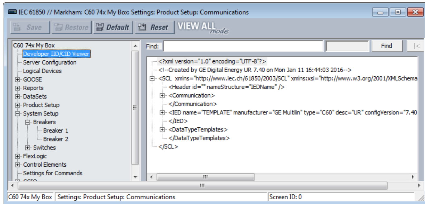
Figure 32: View CID settings file (Edition 2)
