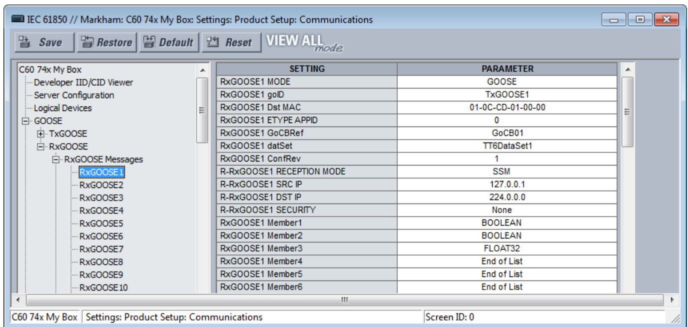
Figure 13: IEC 61850 RxGOOSE Messages panel
