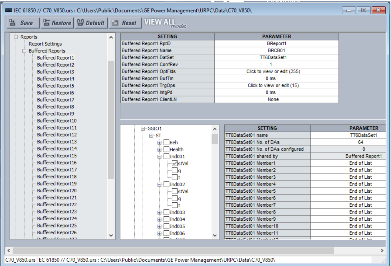
Figure 45: IEC 61850 buffered report panel
