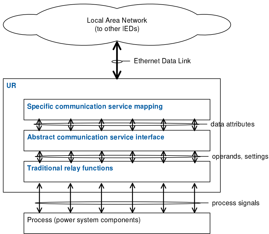
Figure 8: IEC 61850 and device overview
