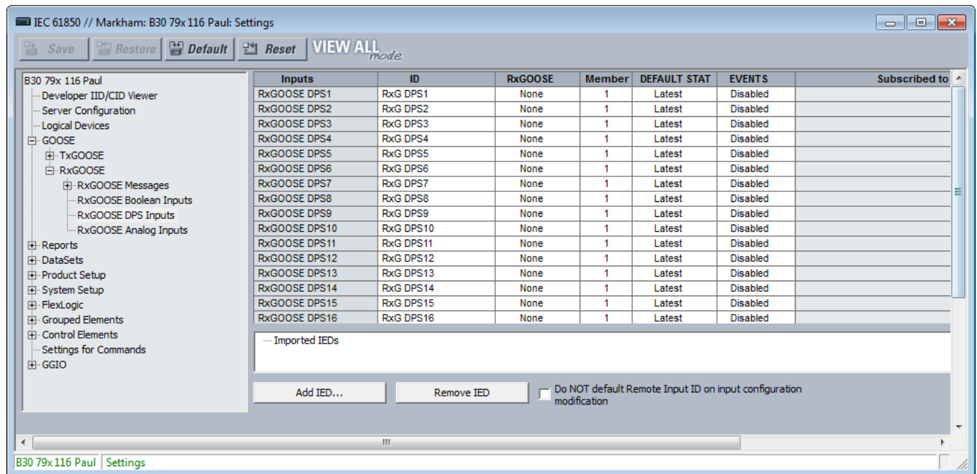
Figure 42: RxGOOSE DPS Inputs panel (Edition 2)
