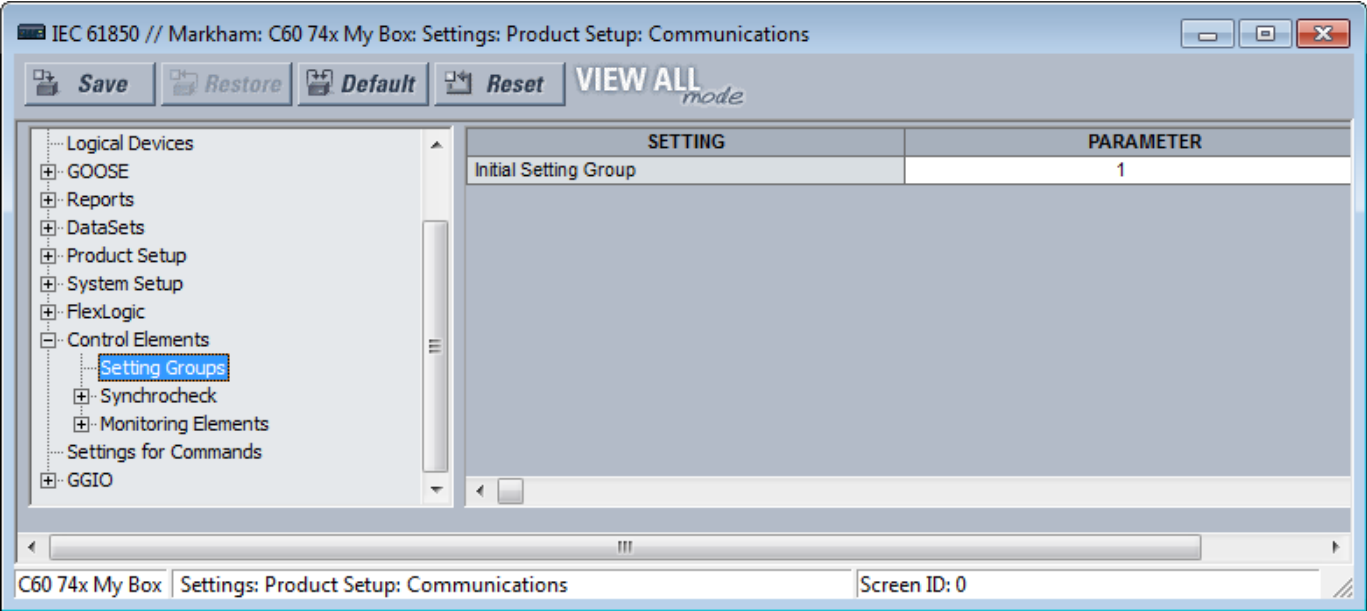
Figure 55: Setting Groups panel (Edition 2)
