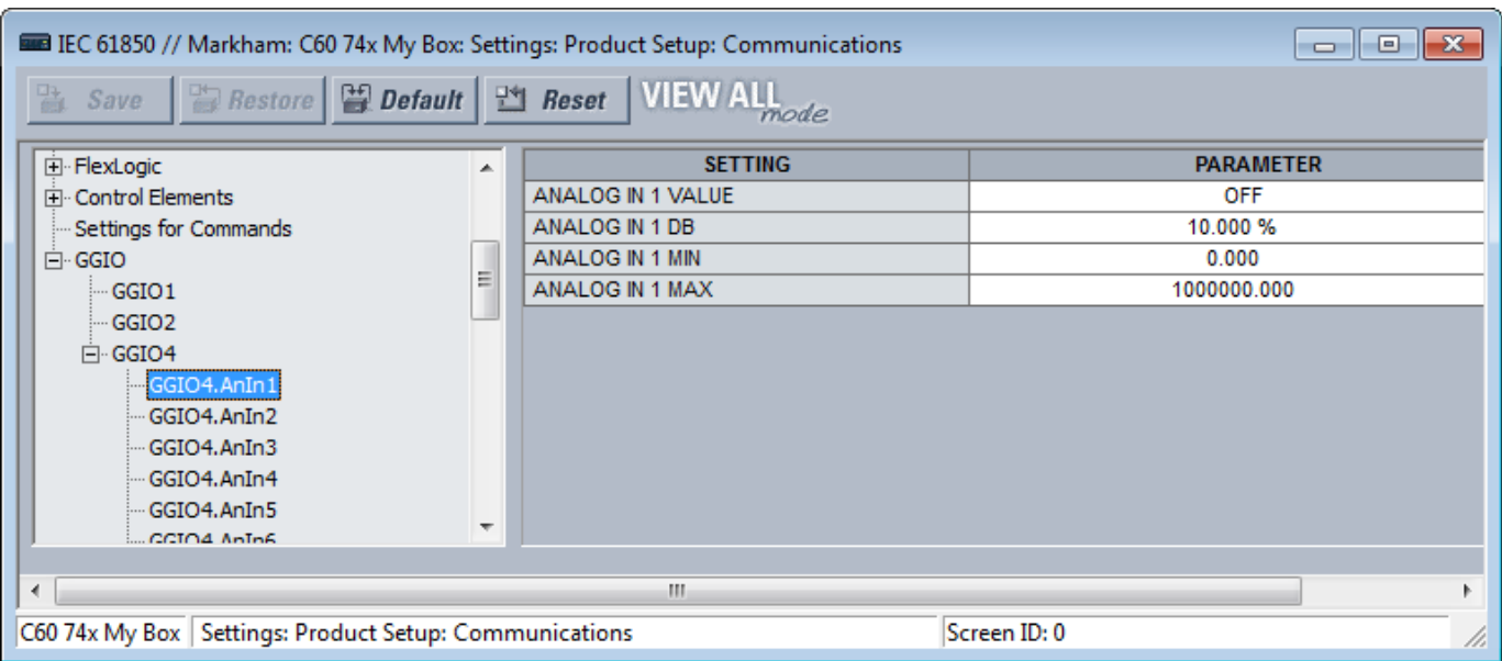
Figure 59: GGIO4 panel (Edition 2)
