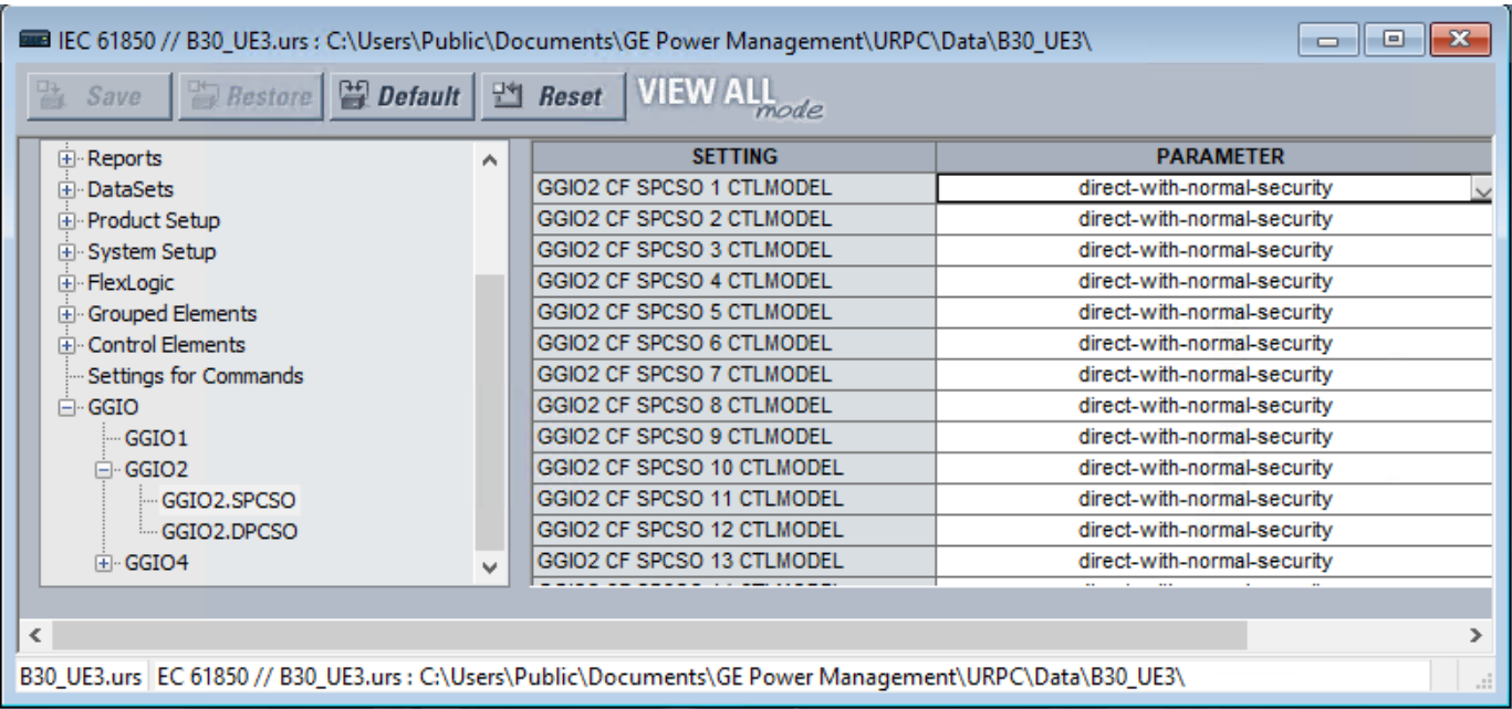
Figure 58: GGIO2 panel (Edition 2)
