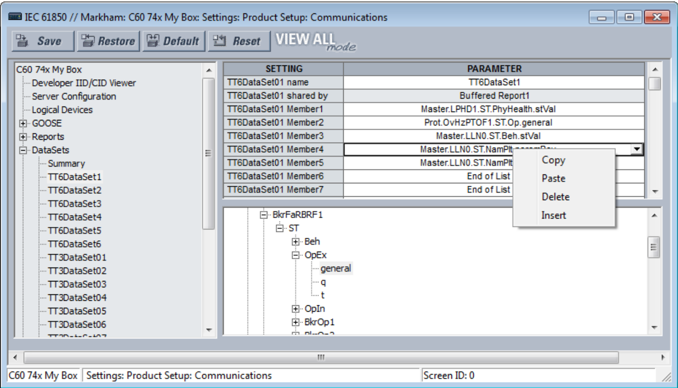
Figure 48: Member right-click
