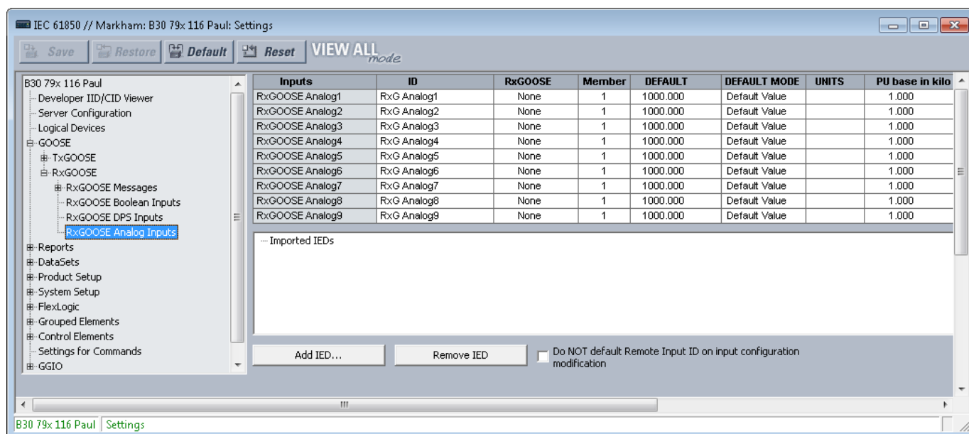
Figure 43: RxGOOSE Analog Inputs panel (Edition 2)
