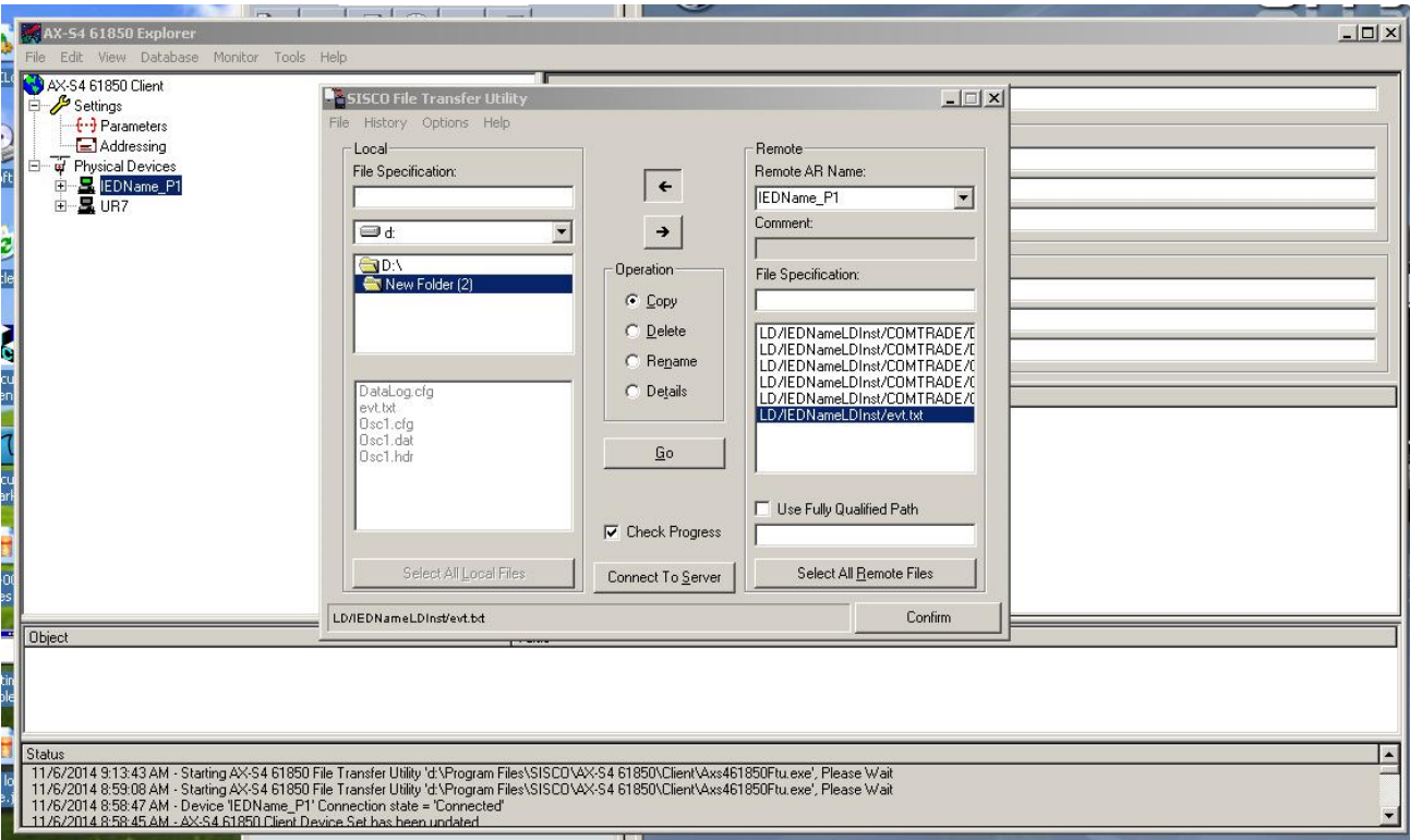
Figure 60: File transfer by IEC 61850
