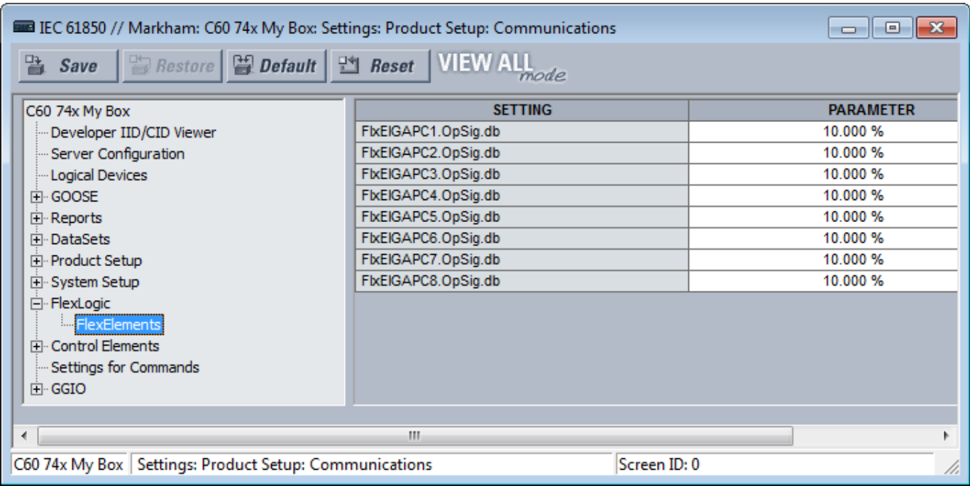
Figure 51: Deadband settings with .db suffix (Edition 2)
