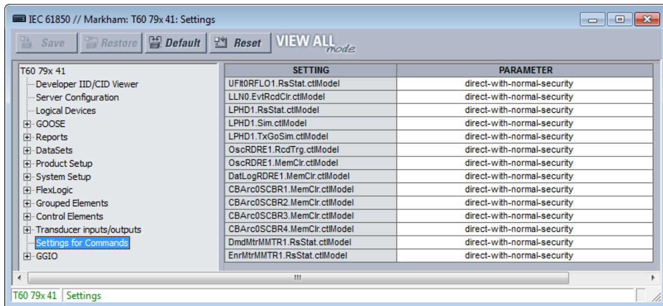
Figure 56: Commands panel (Edition 2)
