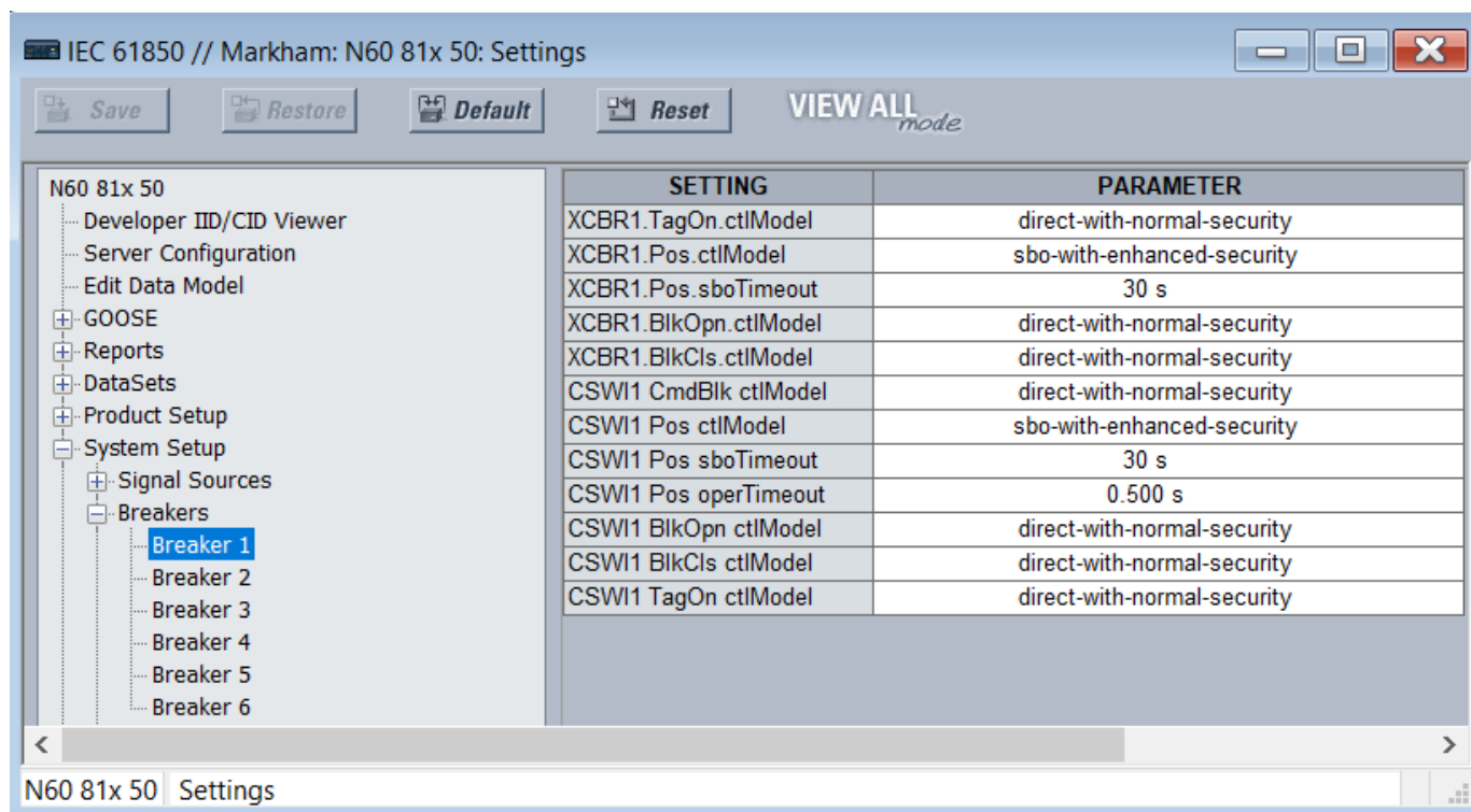
Figure 53: IEC 61850 Breaker panel (Edition 2)
