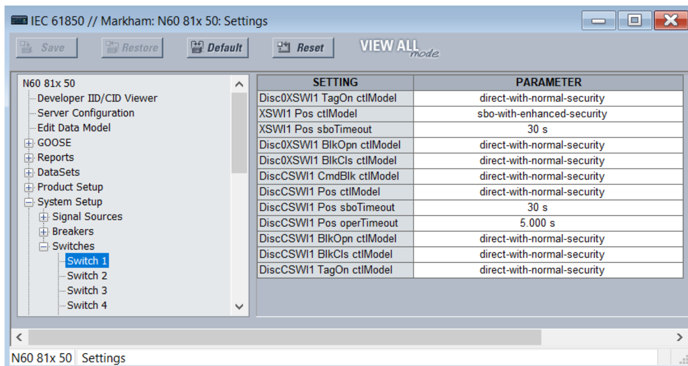
Figure 54: Switch panel
