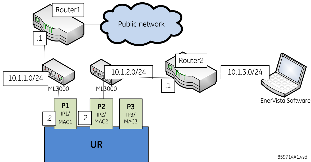
Figure 4: Using static routes
