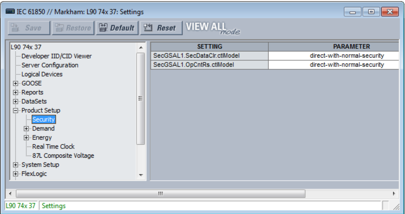
Figure 49: IEC 61850 Security
