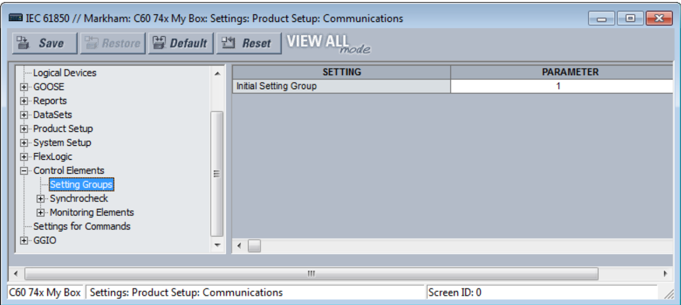
Figure 56: Setting Groups panel (Edition 2)
