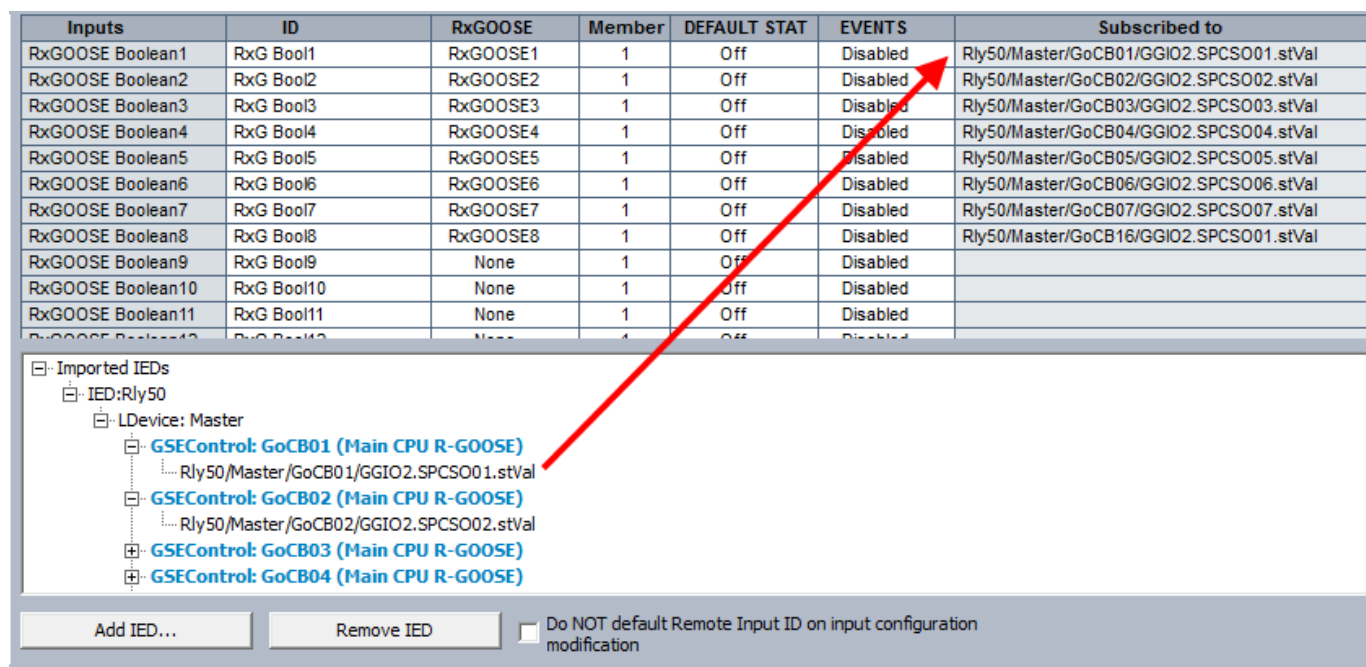
Figure 40: RxGOOSE subscription
