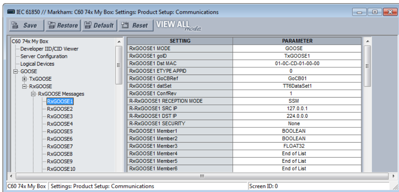
Figure 13: IEC 61850 RxGOOSE Messages panel
