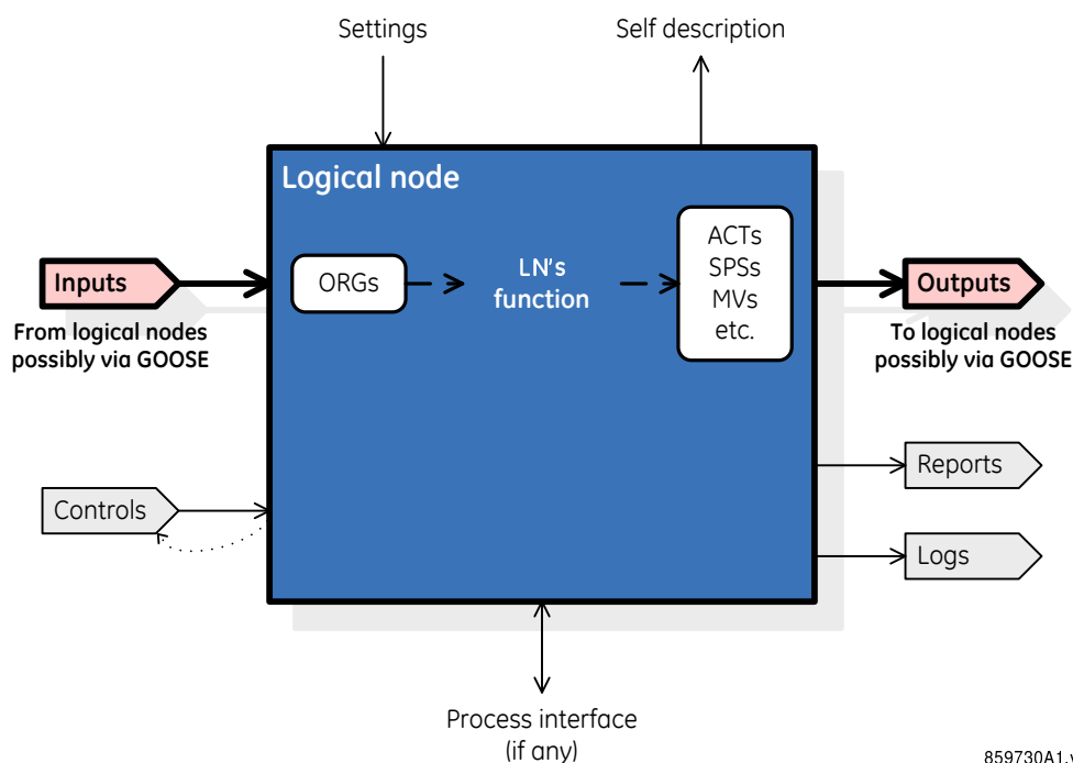
Figure 22: Generic logical node interfaces for the "logical nodes communicate with logical nodes" standard
