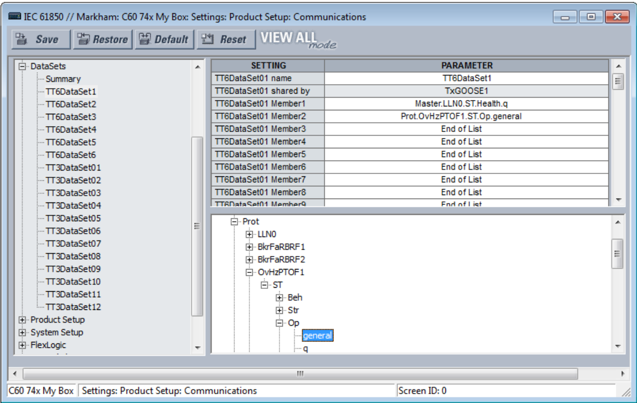
Figure 10: IEC 61850 DataSets
