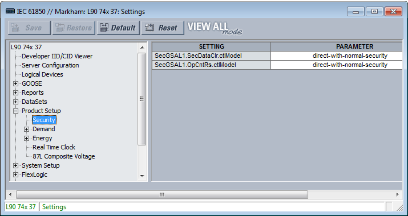
Figure 50: IEC 61850 Security
