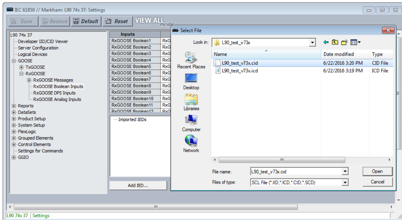
Figure 42: RxGOOSE Boolean Input panel (Edition 2)
