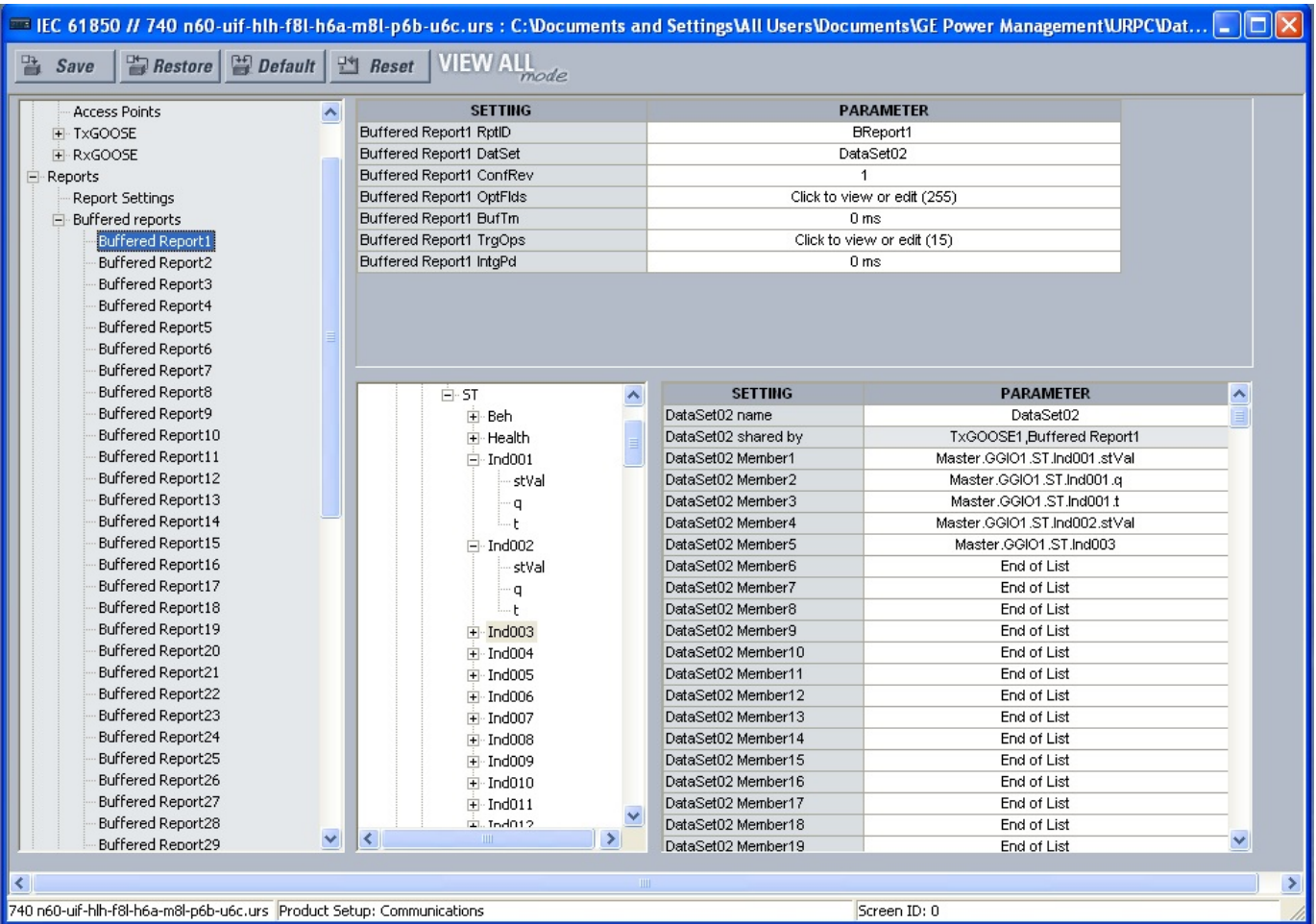
Figure 16: IEC 61850 buffered report panel
