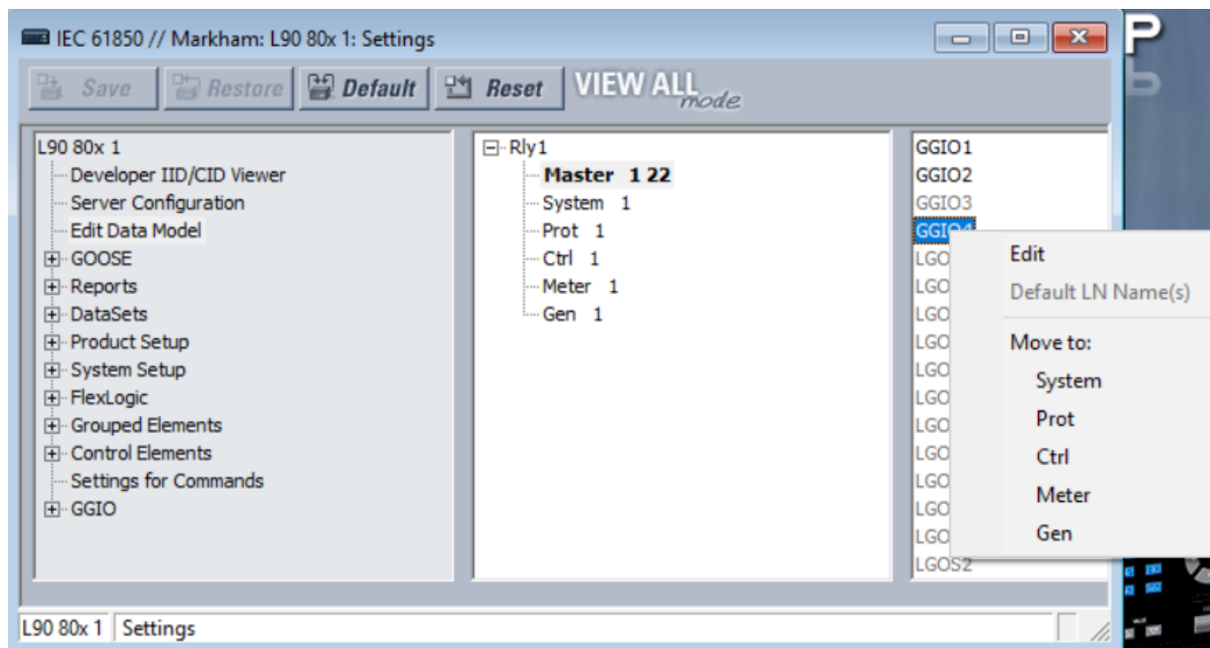
Figure 37: Move logical node (Edition 2)
