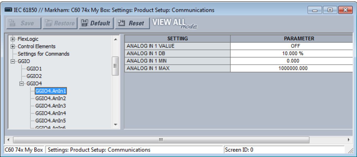
Figure 60: GGIO4 panel (Edition 2)
