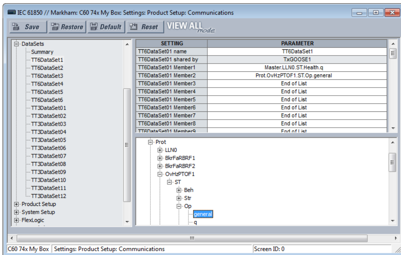
Figure 48: IEC 61850 DataSets (Edition 2)
