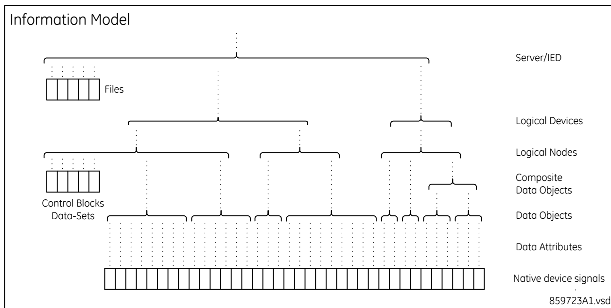
Figure 9: ACSI block
