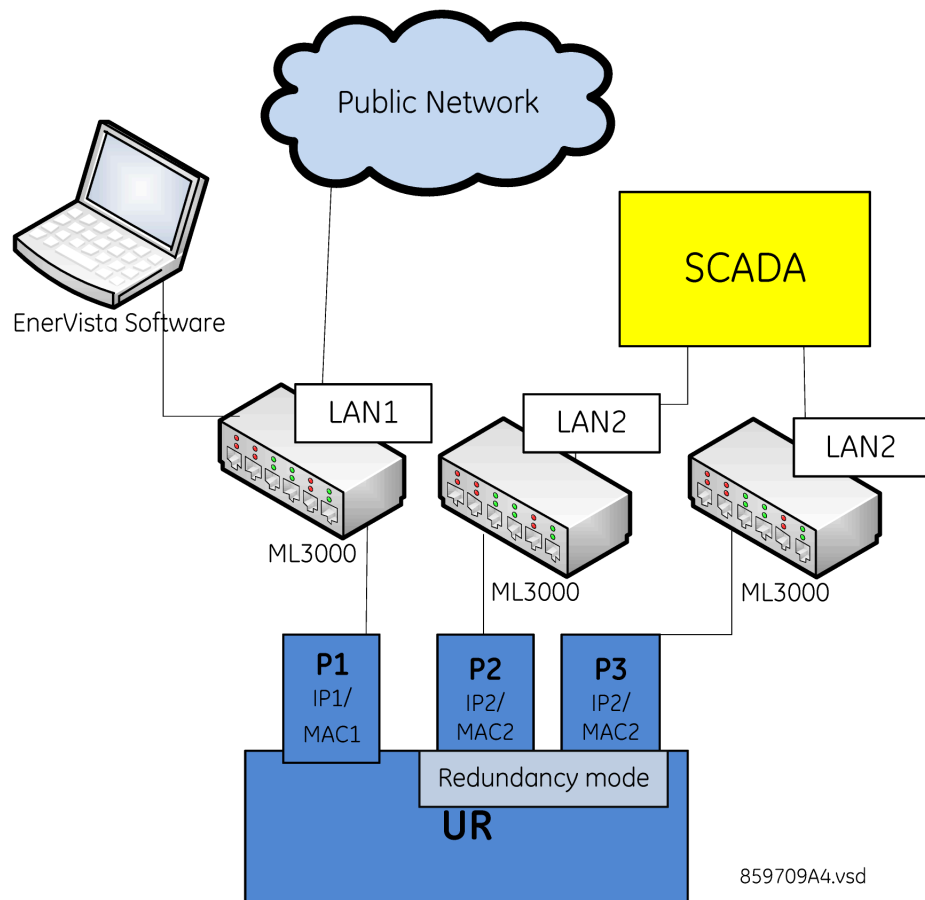
Figure 2: Multiple LANs, with redundancy
