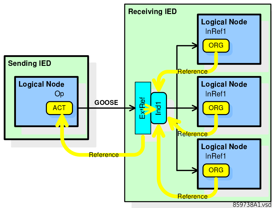
Figure 28: Intermediate object at the receiving end
