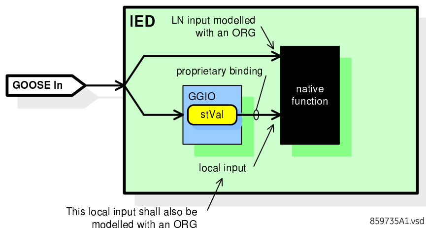
Figure 26: Mapping local inputs
