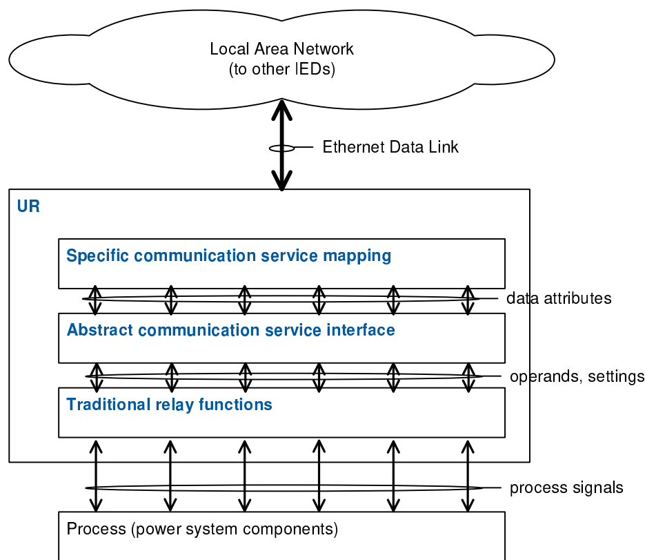
Figure 8: IEC 61850 and device overview
