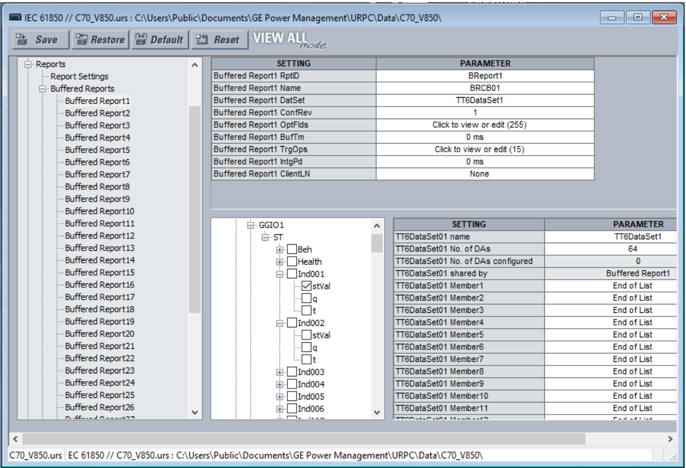
Figure 46: IEC 61850 buffered report panel
