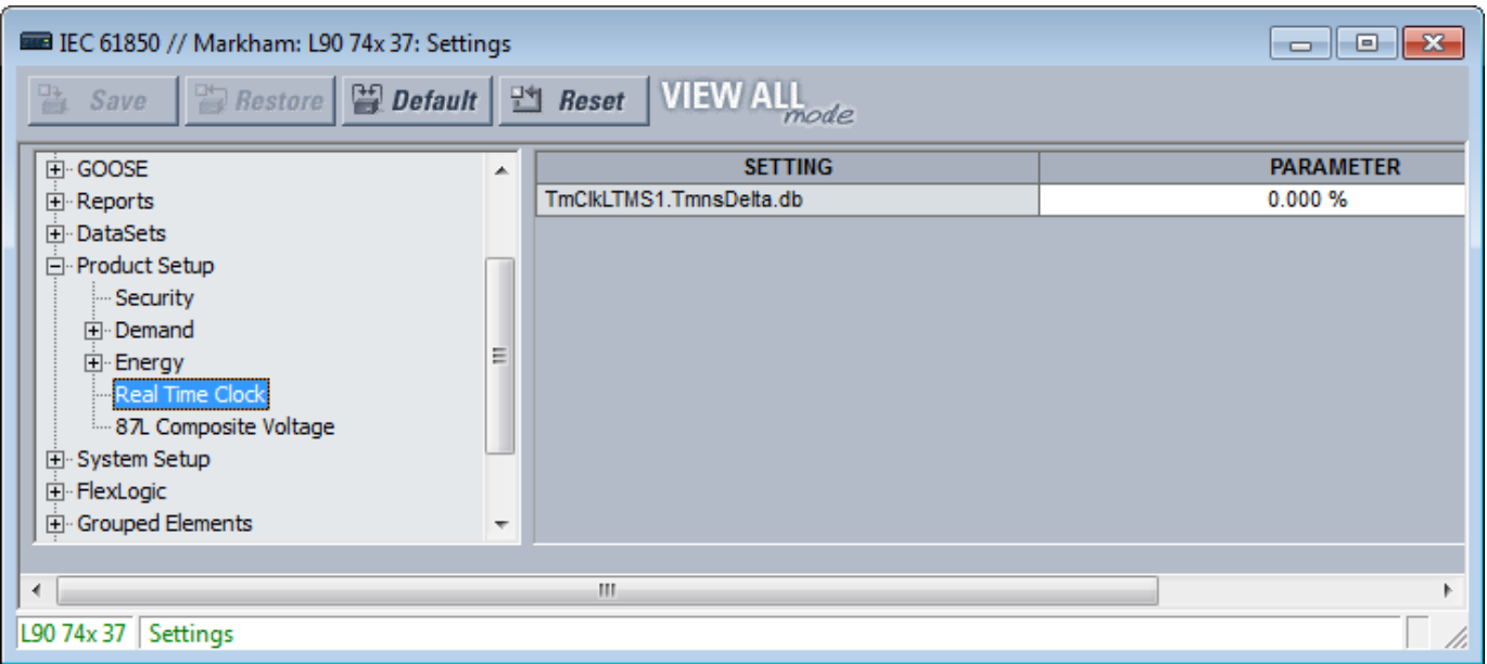
Figure 51: IEC 61850 Real Time Clock
