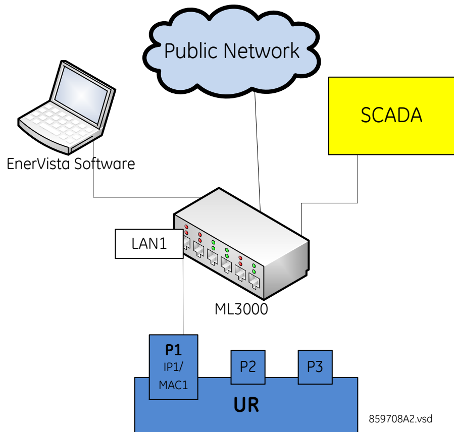
Figure 1: Network configuration for single LAN
