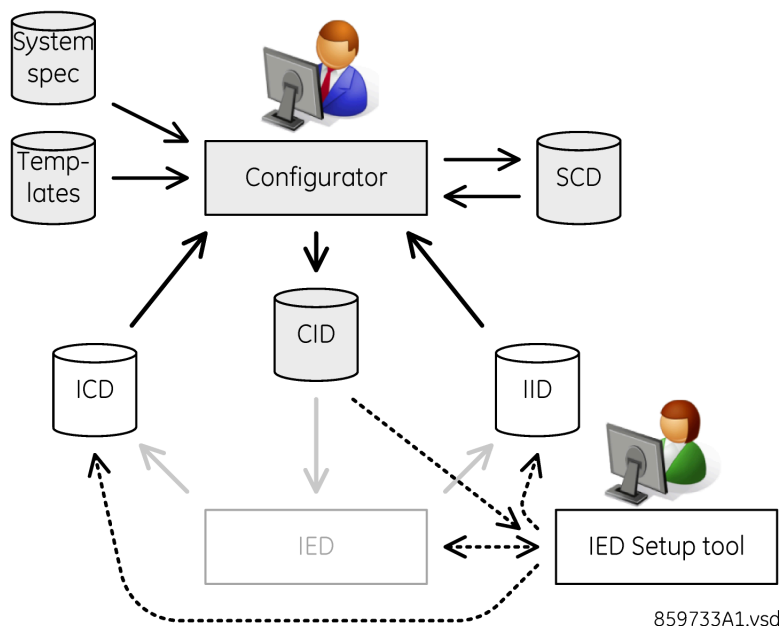
Figure 24: SCL file flow using IED setup tool
