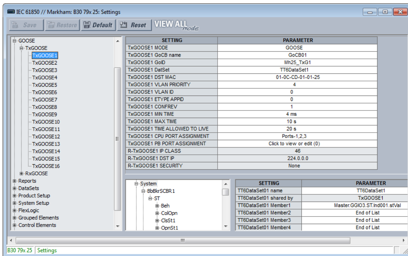
Figure 38: IEC 61850 TxGOOSE panel (Edition 2 and with Process Bus Module)
