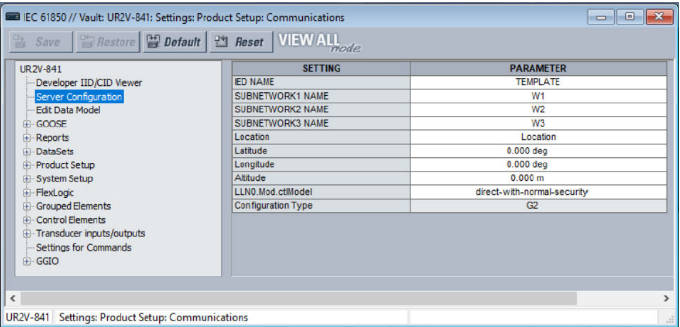
Figure 31: IEC 61850 panel (Edition 2)
