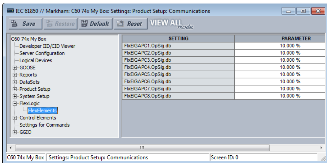
Figure 52: Deadband settings with .db suffix (Edition 2)
