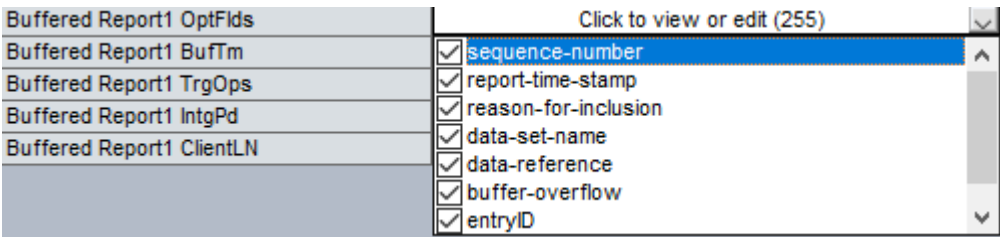
Figure 47: Options for buffered report messages (Edition 2)
