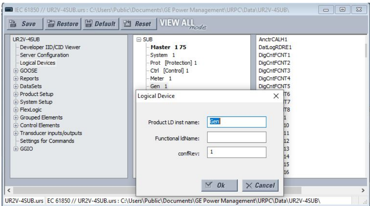
Figure 35: Insert new logical device (Edition 2)
