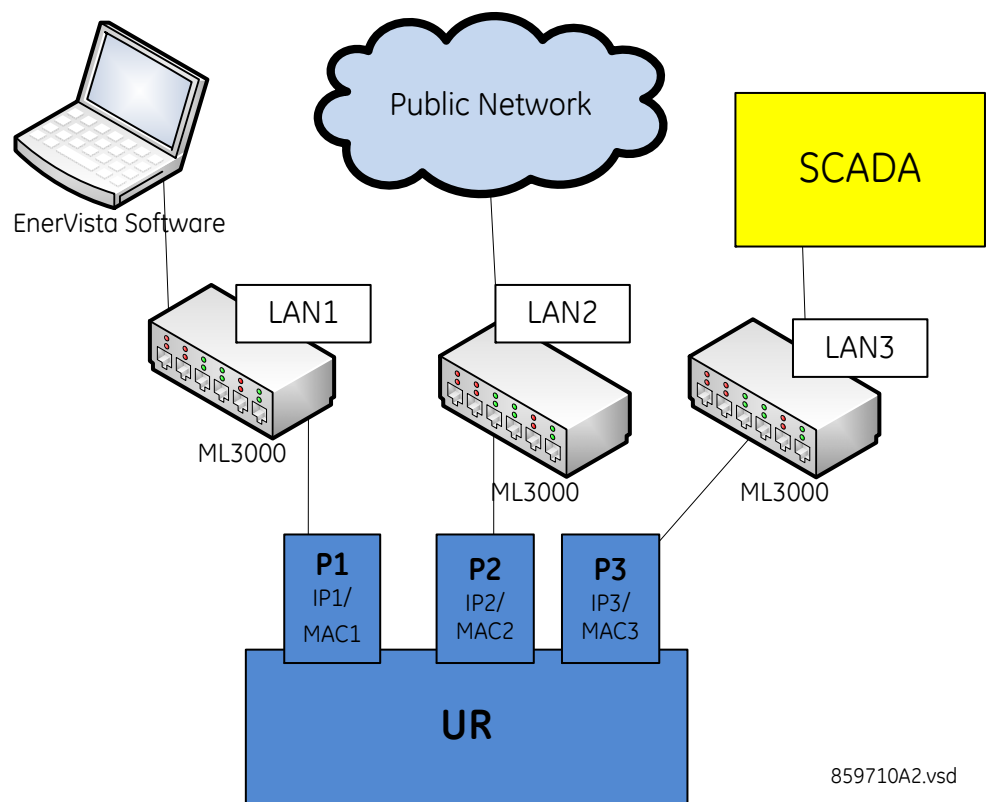
Figure 3: Multiple LANS, no redundancy
