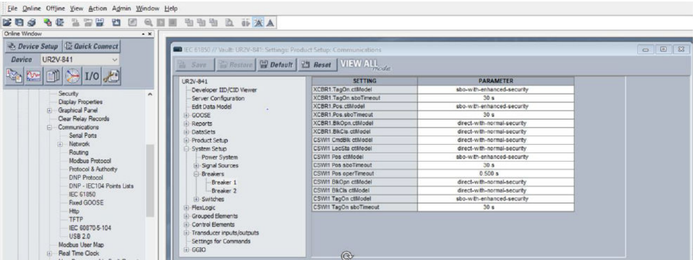
Figure 30: IEC 61850 Edition 2 setup screen in EnerVista
