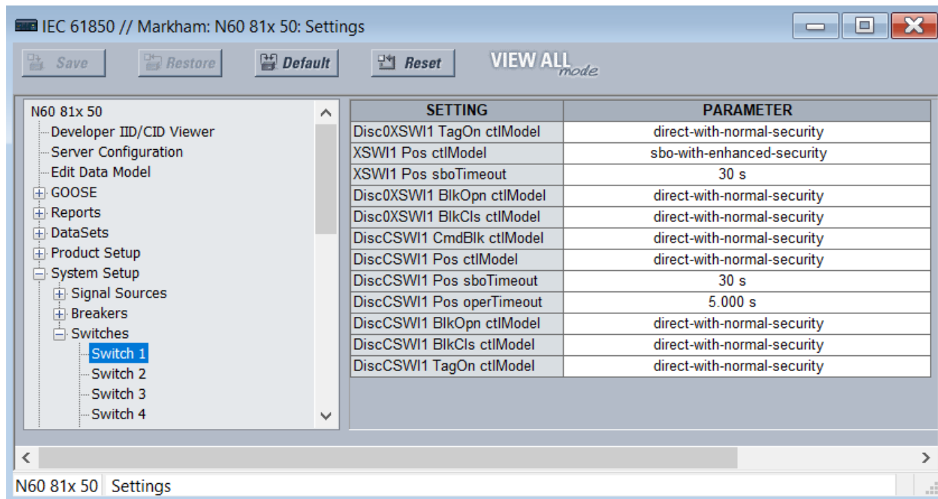
Figure 55: Switch panel
