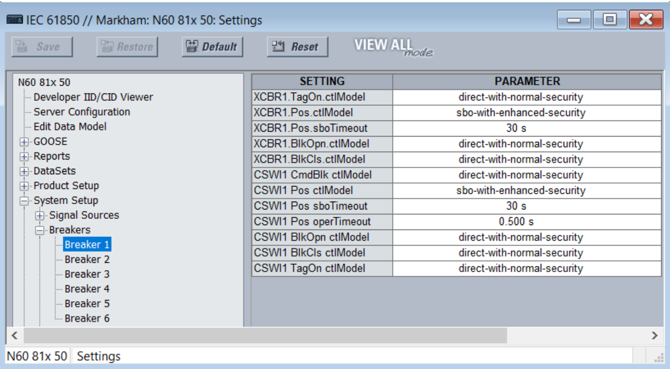
Figure 54: IEC 61850 Breaker panel (Edition 2)
