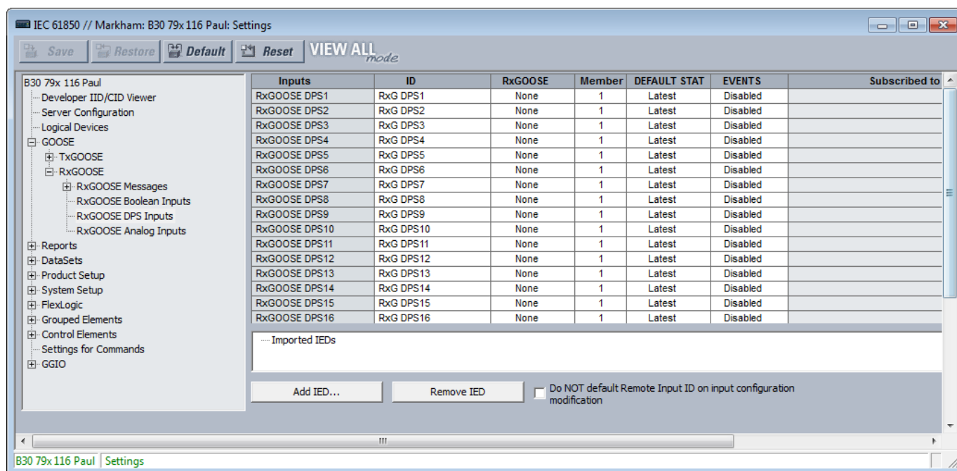
Figure 43: RxGOOSE DPS Inputs panel (Edition 2)
