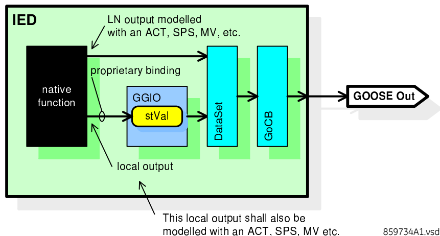
Figure 25: Mapping local outputs
