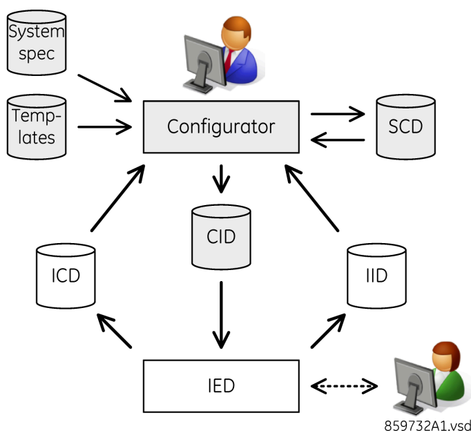
Figure 23: SCL file flow for IED configuration
