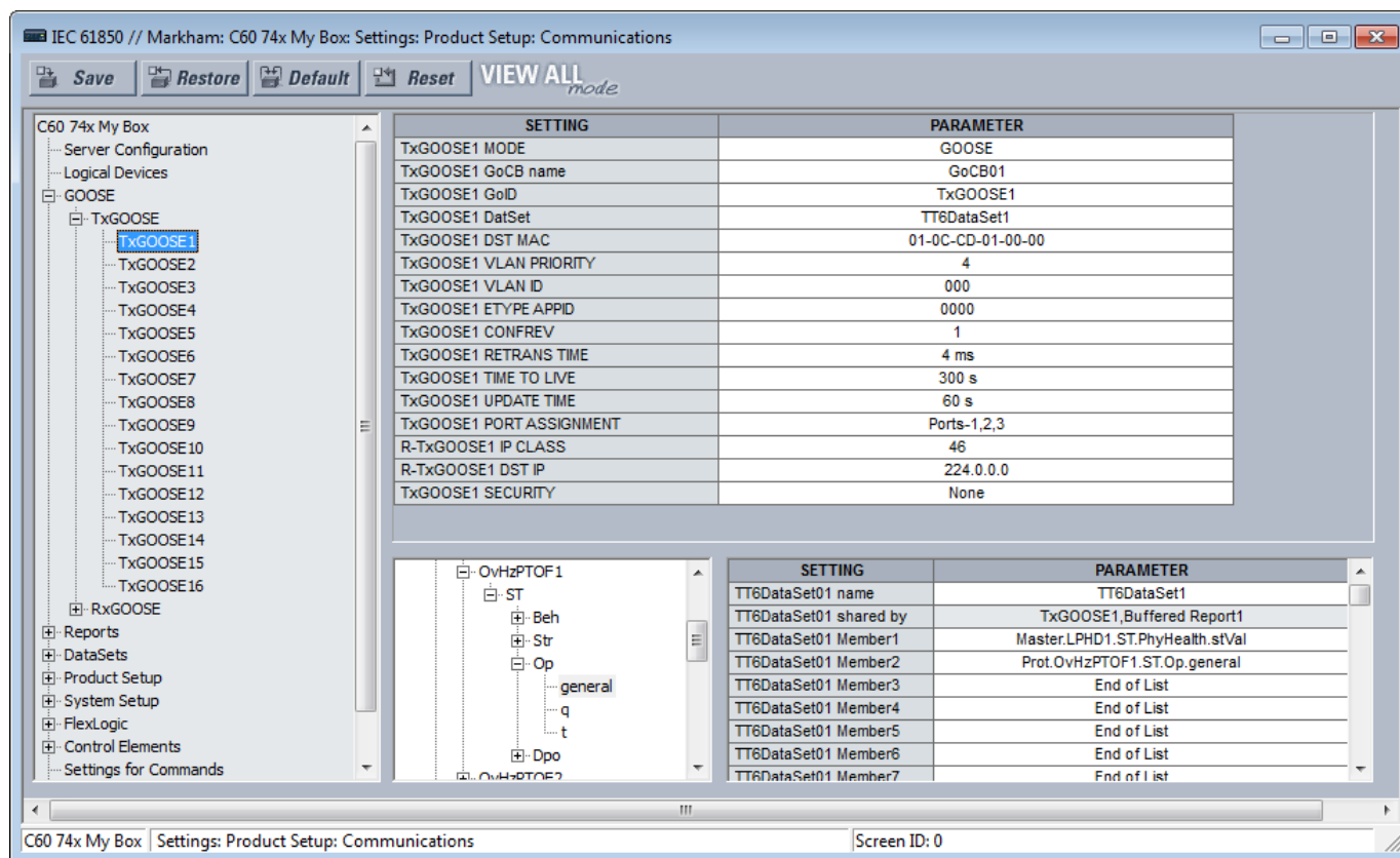
Figure 12: IEC 61850 TxGOOSE panel
