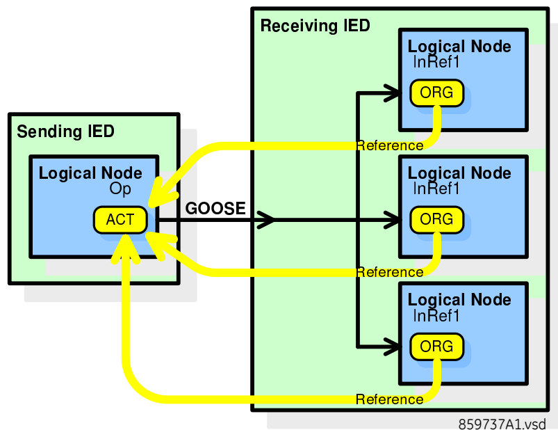
Figure 27: Logical nodes communicate with logical nodes
