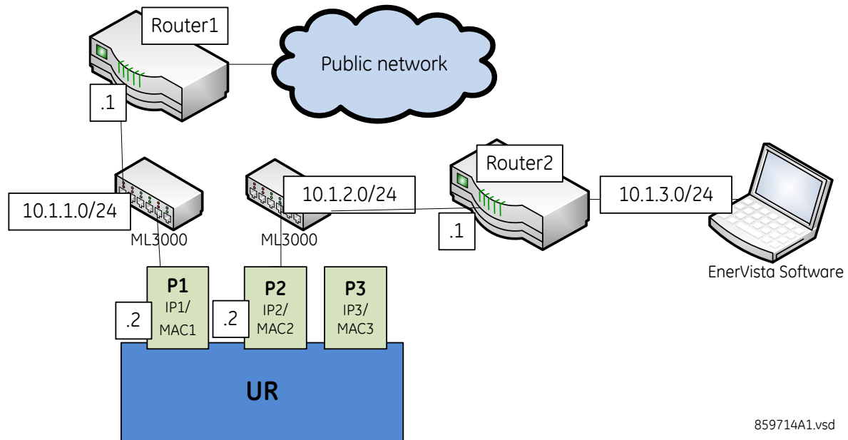
Figure 4: Using static routes
