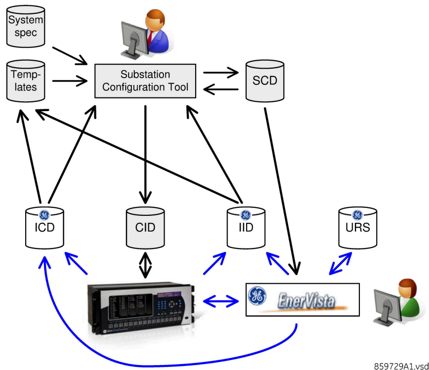
Figure 17: Configuration for IEC 61850
