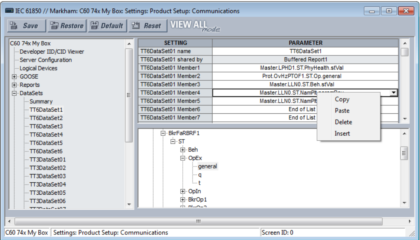
Figure 49: Member right-click
