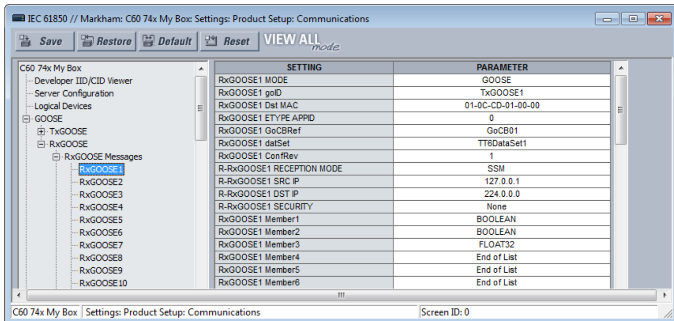
Figure 39: IEC 61850 RxGOOSE Messages panel (Edition 2)
