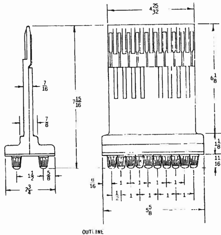
Fig. 12 Outline of the XLA13A Test Plug
