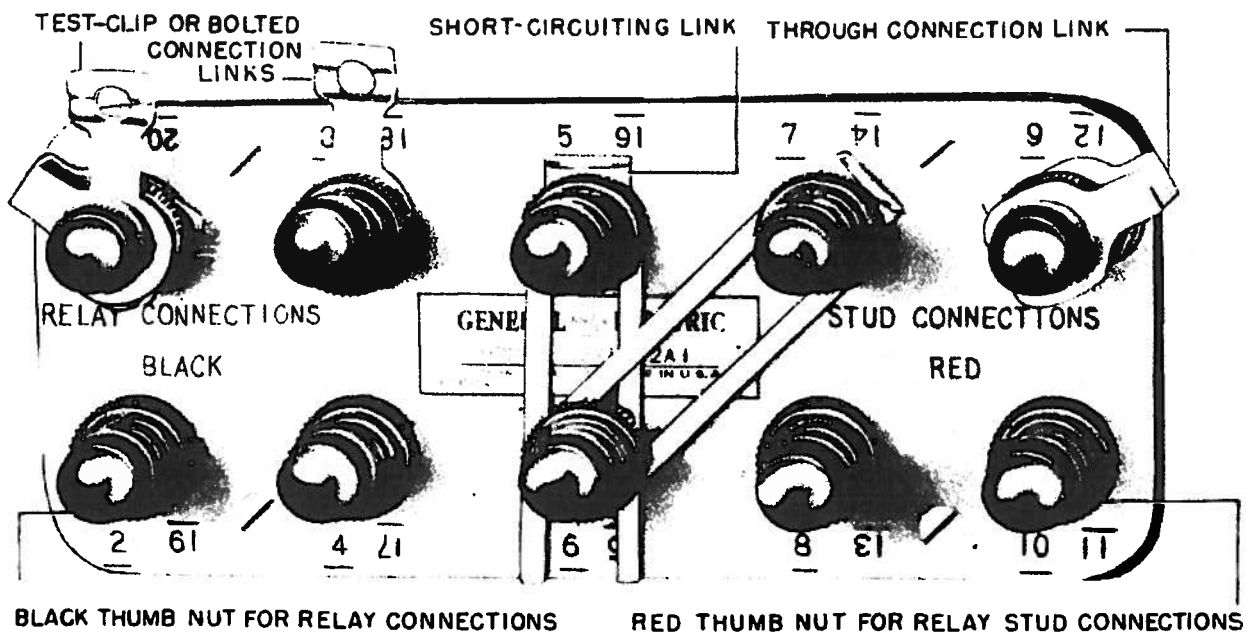
Fig. 4 Test Links in Use on the XLA12A Test Plug
