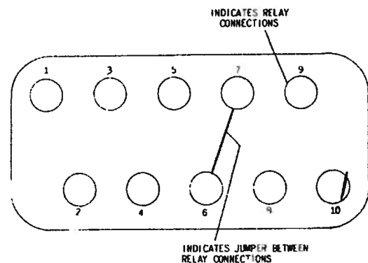
Fig. 10 Conventional Representation of XLA13A Test Plug Connections
