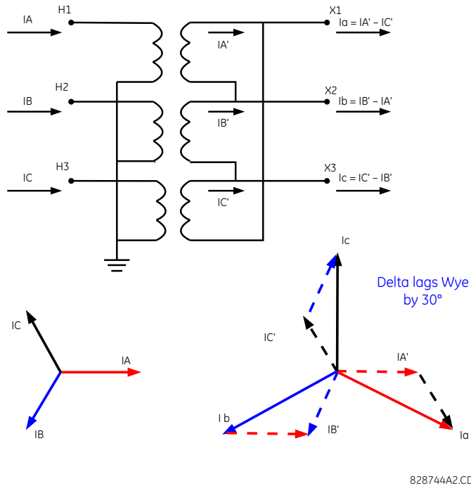
FIGURE 1. ABC Power System Rotation
