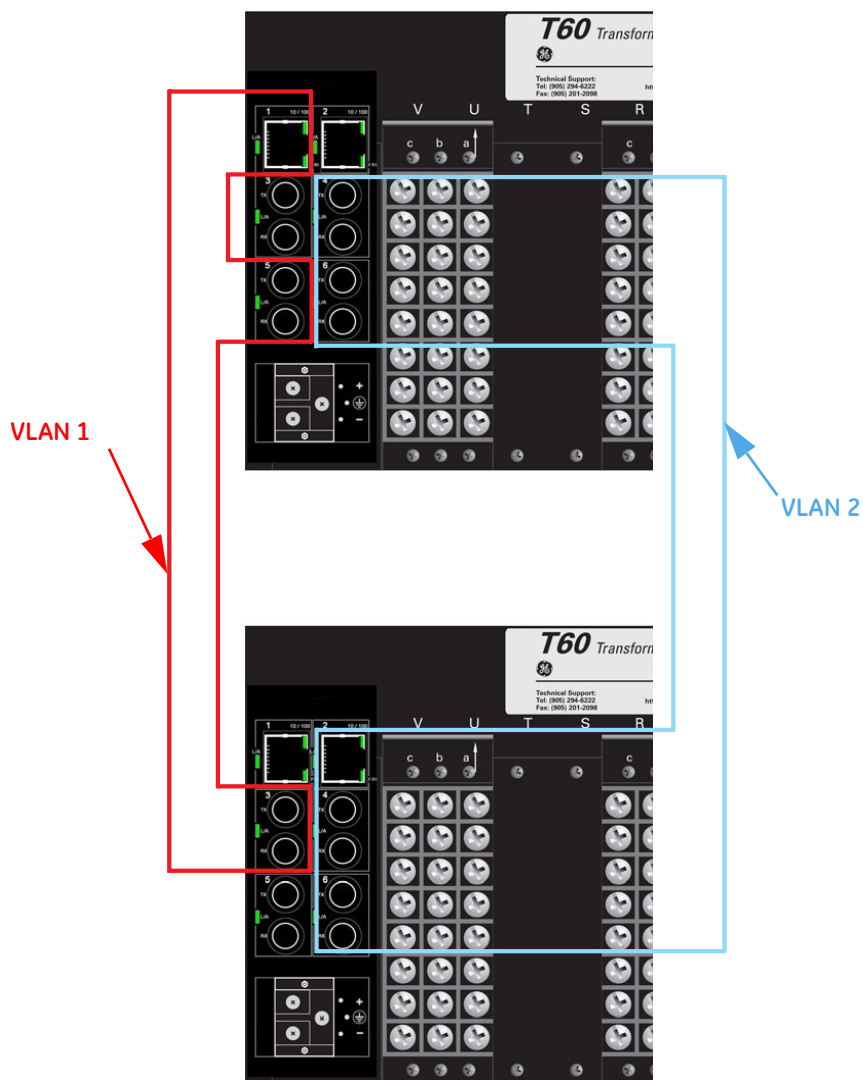
FIGURE QS-13: Tagged Virtual LANs
