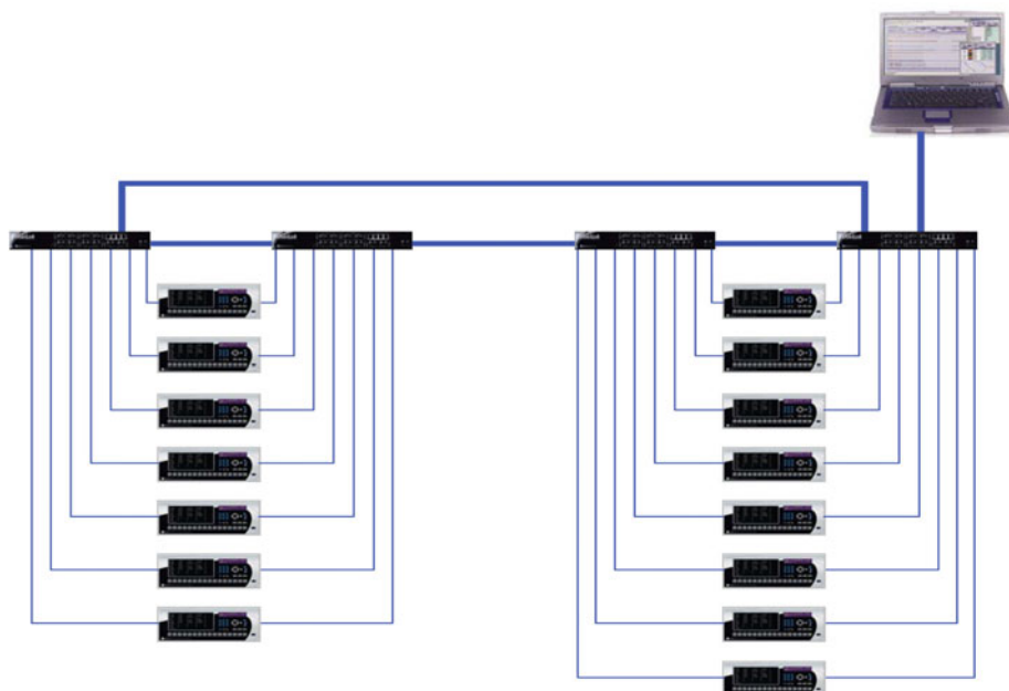
FIGURE QS-5: Traditional Redundant UR LAN Topology
