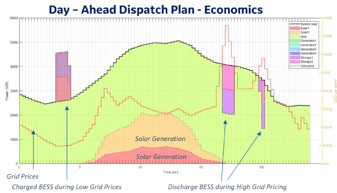
Figure 6: Economic dispatch plan
