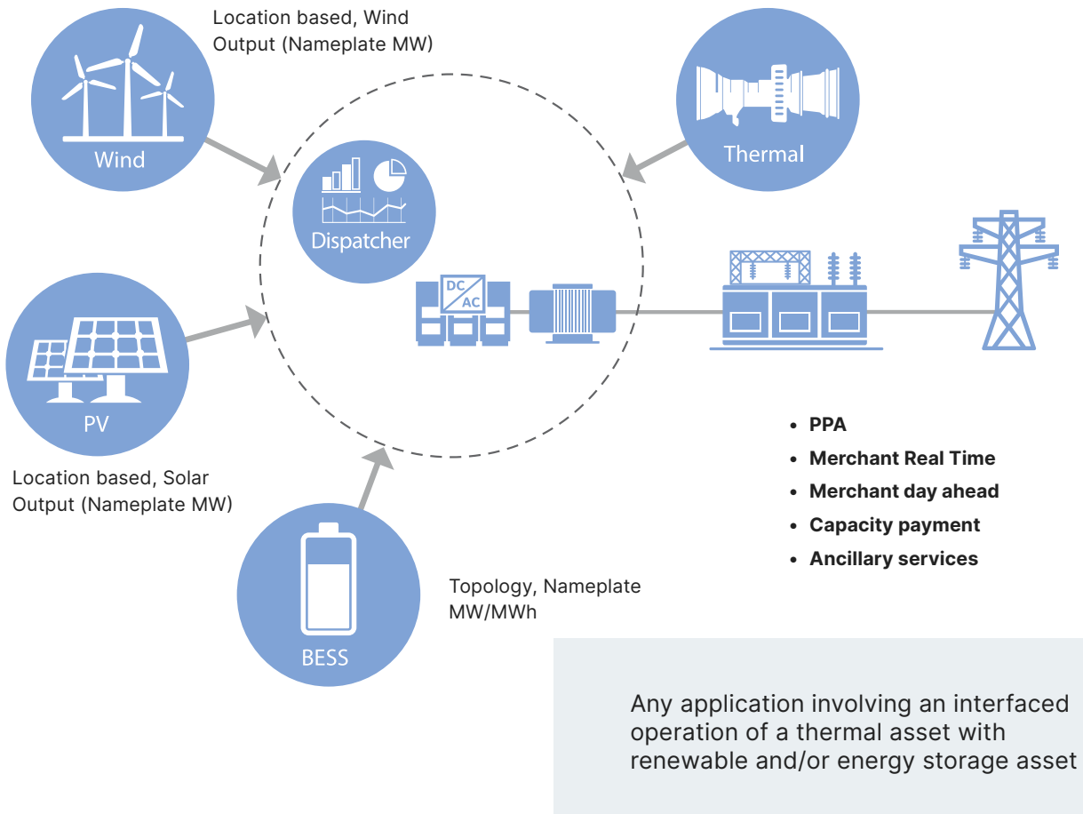
Figure 7. Thermal Hybrids
