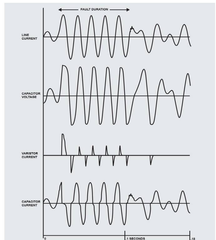
Figure 2. External line fault oscillogram.
