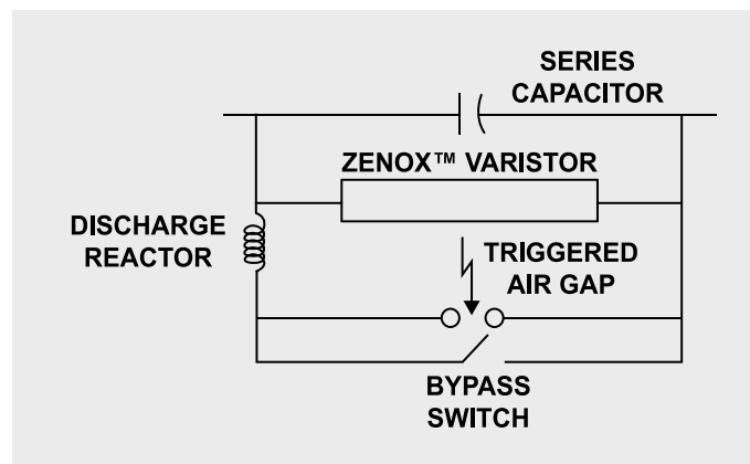
Figure 4. One-Line diagram of an MOV protected series capacitor.
