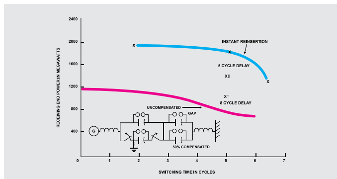
Figure 3. Effect of reinsertion delay on power transfer.
