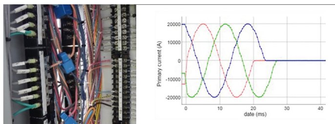
Acquiring interrupted current from primary CTs
