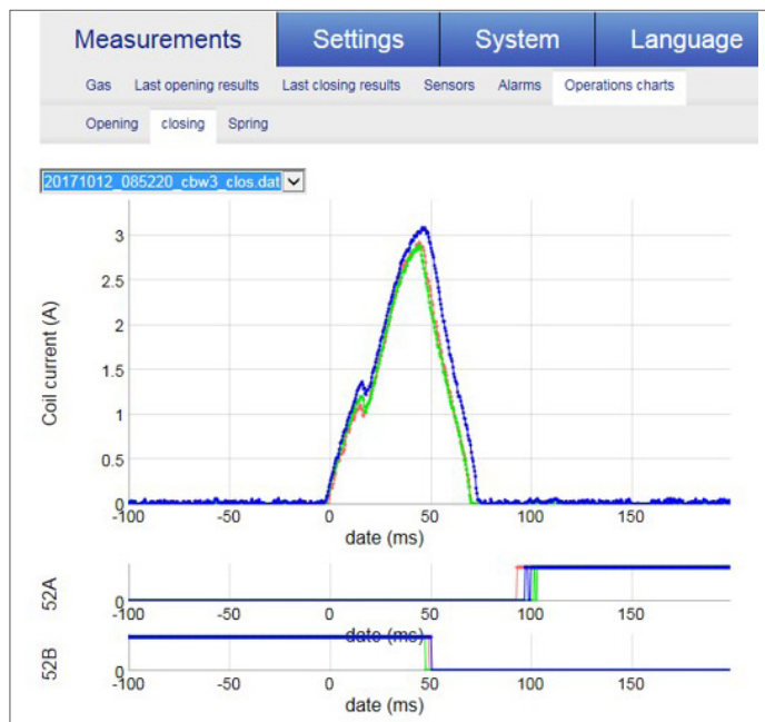
Coil Current - Closing
