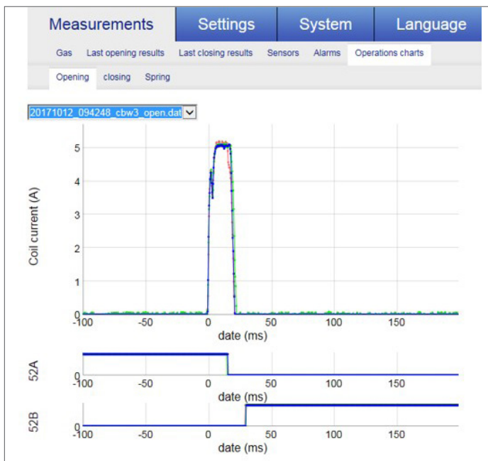
Coil Current - Opening
