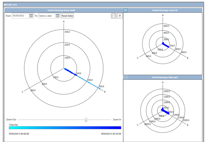
Partial discharge alarms and PRPD evaluation
