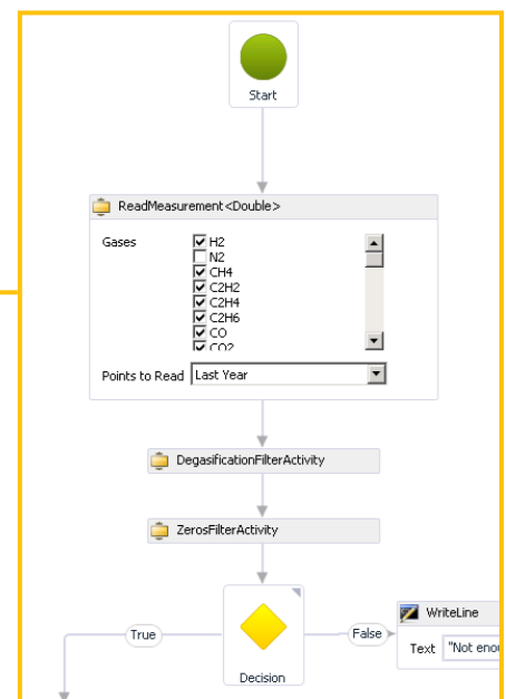
Algorithm workflow evaluation statements and decisions
