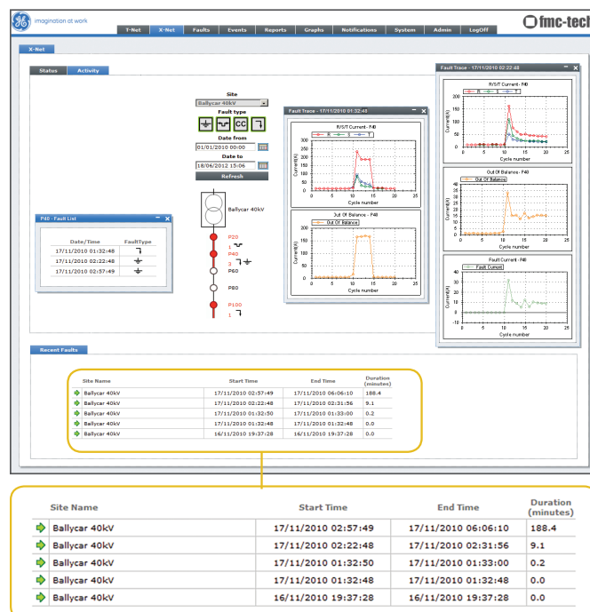
Support maintenance prioritization based on fault history activity for feeder segments
